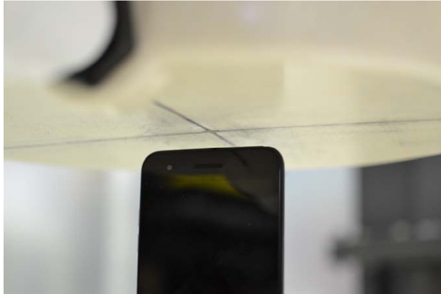
SAR Test Setup Photo 7: Top at 1.0 cm
