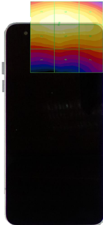
Figure 18-4 E-Field WD Scan overlay (T-Coil Centered Scan area pictured)
