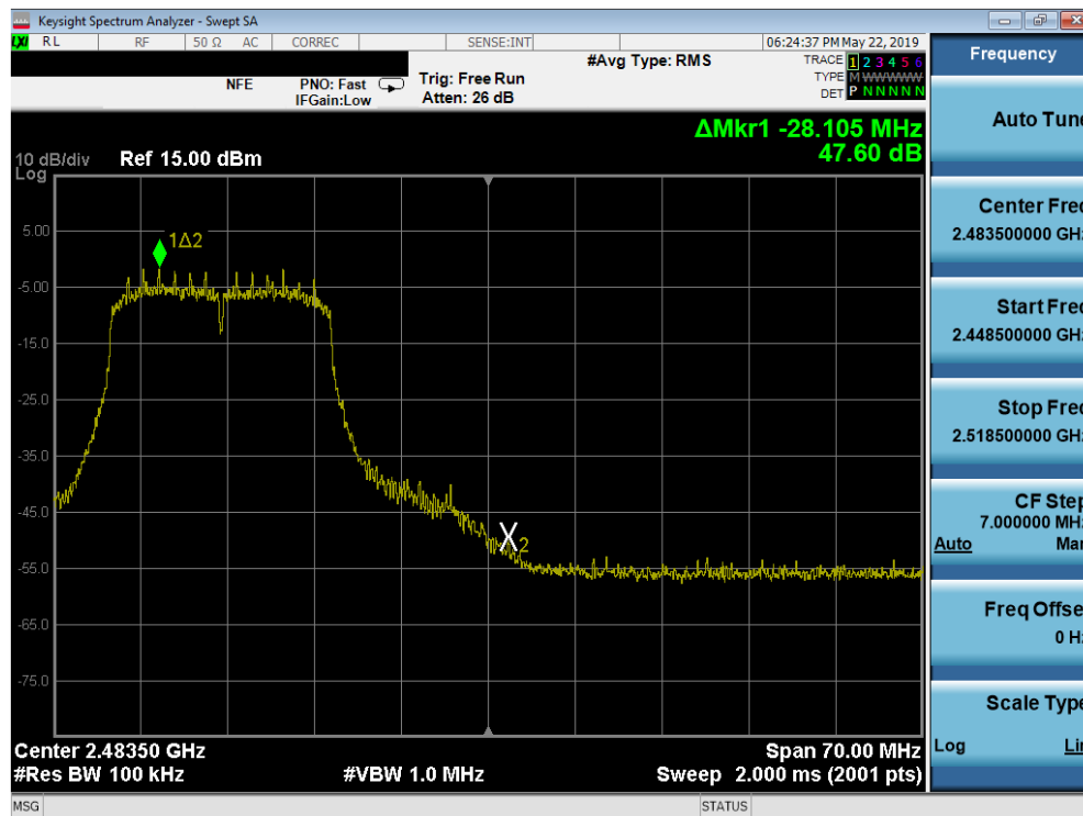
Plot 7-27. Band Edge Plot (802.11n (2.4GHz) – Ch. 11)
