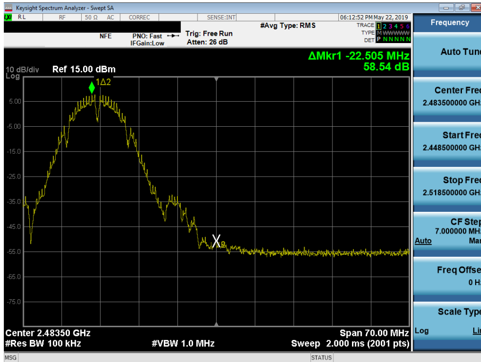
Plot 7-21. Band Edge Plot (802.11b – Ch. 11)
