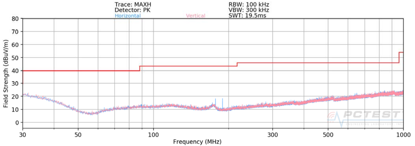
Plot 7-44. Radiated Spurious Plot below 1GHz
