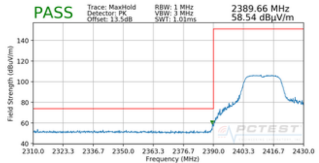
Plot 7-39. Radiated Restricted Lower Band Edge Measurement (Peak)
