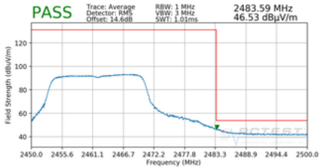
Plot 7-42. Radiated Restricted Upper Band Edge Measurement (Average)
