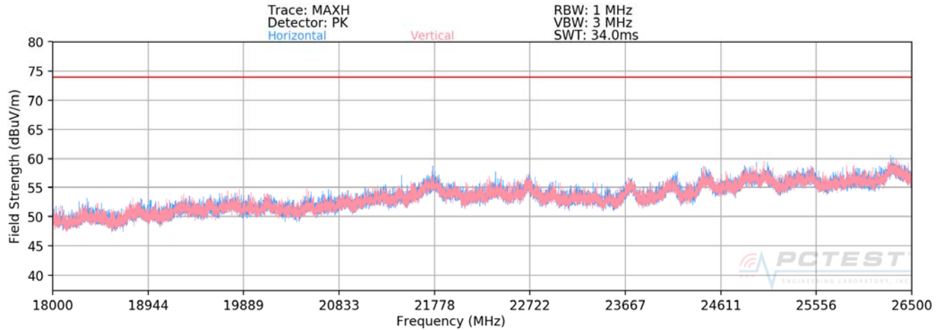
Plot 7-37. Radiated Spurious Plot above 18GHz
