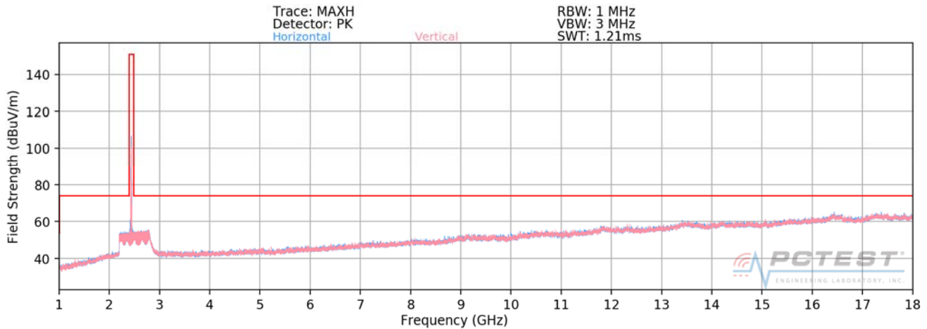
Plot 7-35. Radiated Spurious Plot above 1GHz (802.11b – Ch. 6)
