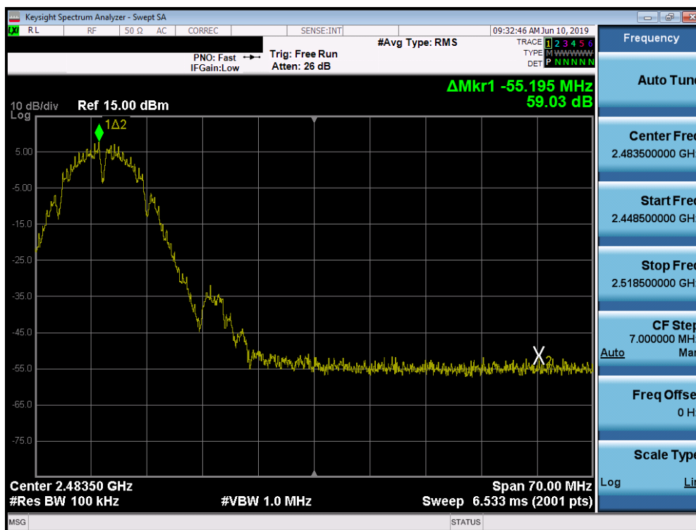
Plot 7-20. Band Edge Plot (802.11b – Ch. 10)
