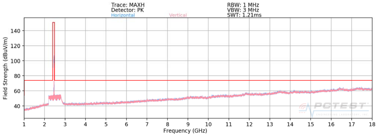
Plot 7-36. Radiated Spurious Plot above 1GHz (802.11b – Ch. 11)
