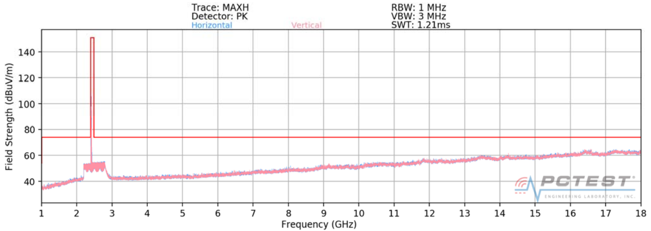
Plot 7-34. Radiated Spurious Plot above 1GHz (802.11b – Ch. 1)
