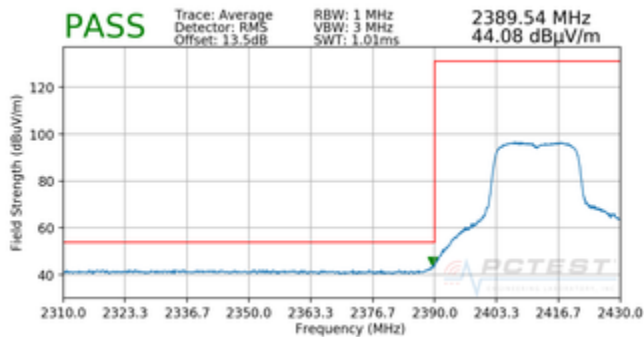
Plot 7-38. Radiated Restricted Lower Band Edge Measurement (Average)
