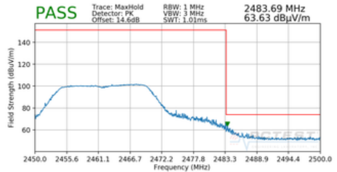
Plot 7-43. Radiated Restricted Upper Band Edge Measurement (Peak)
