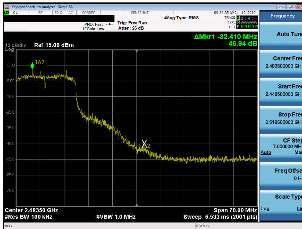
Plot 7-26. Band Edge Plot (802.11n (2.4GHz) – Ch. 10)
