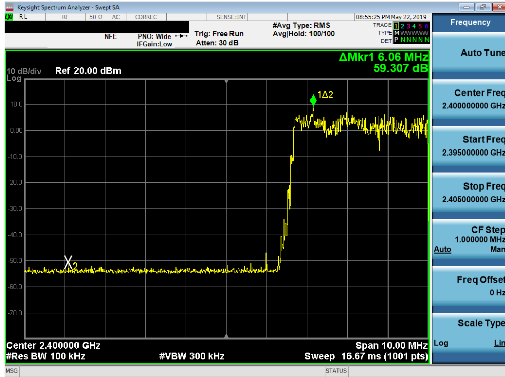
Plot 7-30. Band Edge Plot (Bluetooth with Hopping Enabled, GFSK, ePA)
