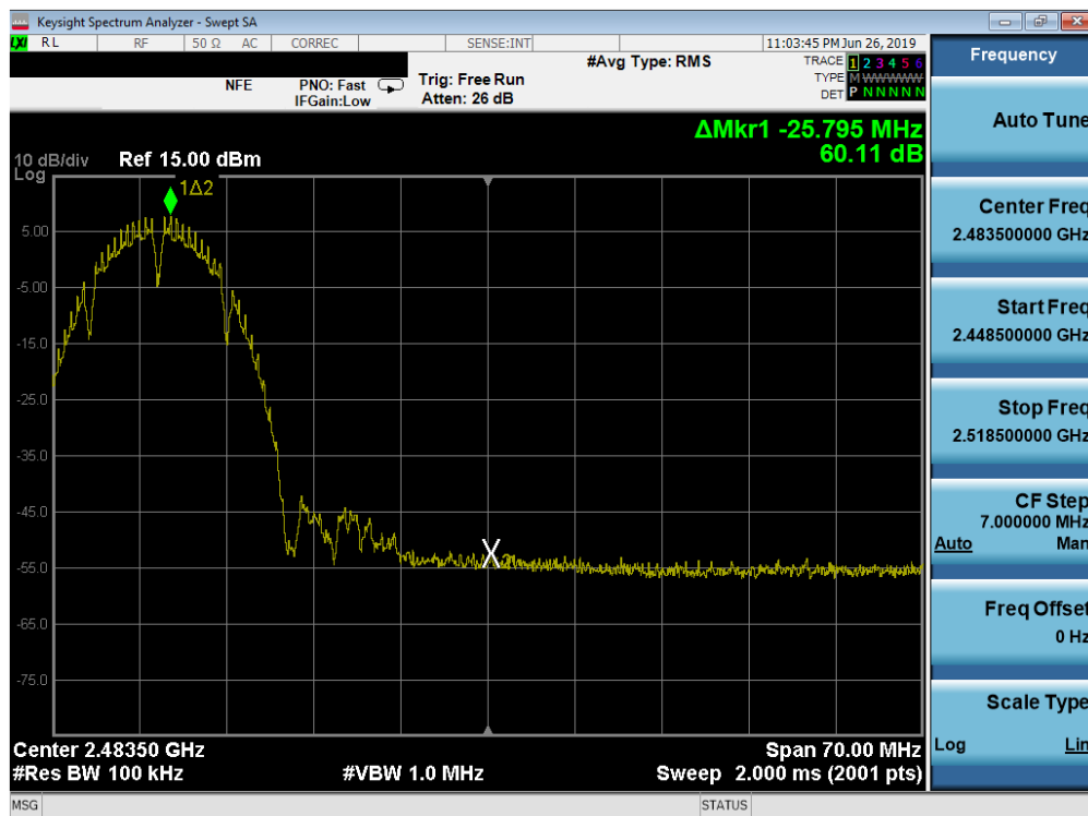
Plot 7-21. Band Edge Plot (802.11b – Ch. 10)
