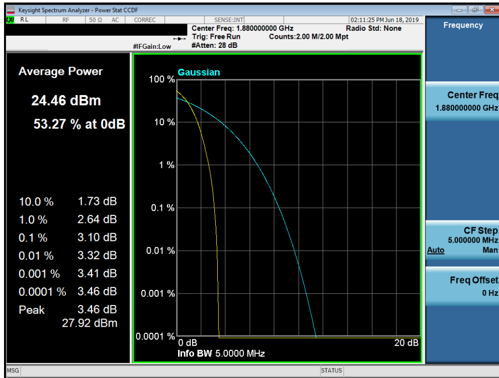
Plot 7-101. Peak-Average Ratio Plot (PCWCDMA Mode)
