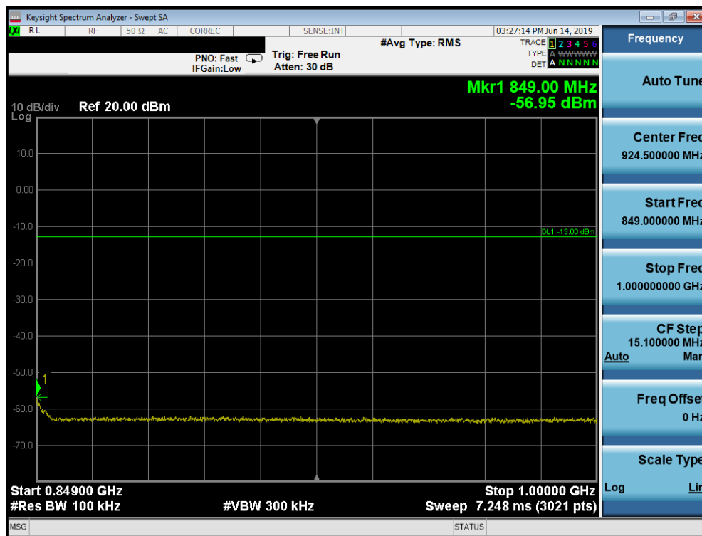
Plot 7-50. Conducted Spurious Plot (Cellular WCDMA Mode - Mid Channel)
