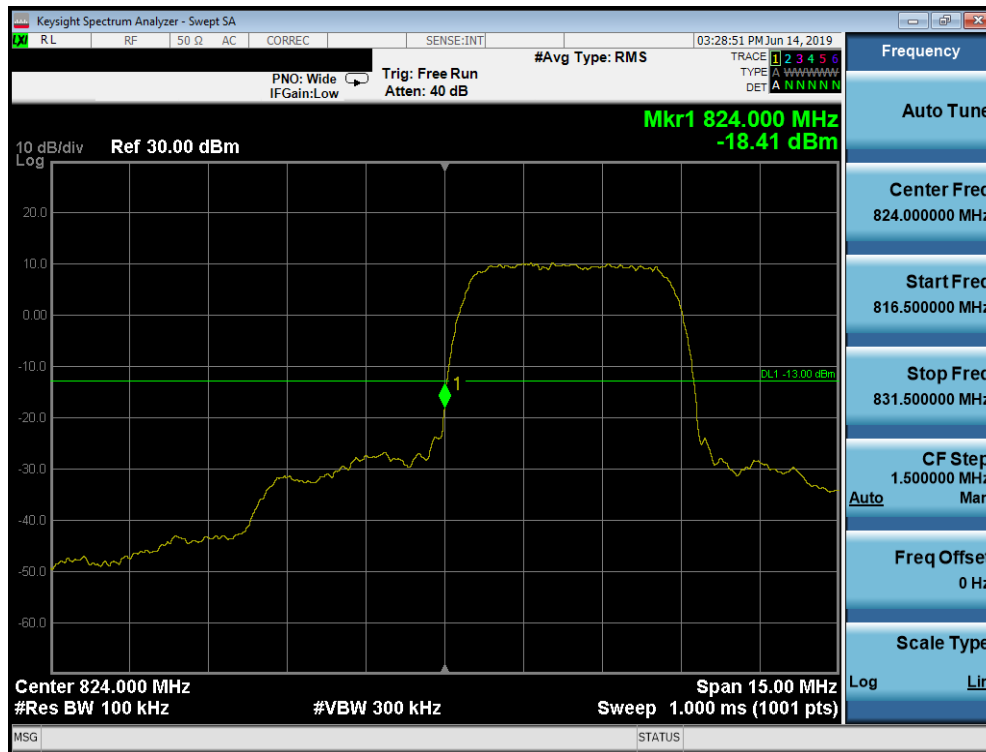
Plot 7-87. Band Edge Plot (Cellular WCDMA Mode - Low Channel)
