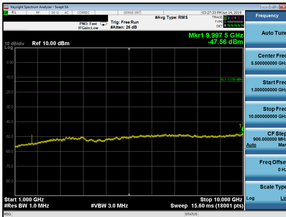
Plot 7-51. Conducted Spurious Plot (Cellular WCDMA Mode - Mid Channel)
