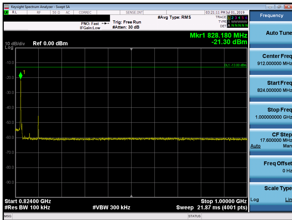
Plot 7-25. Conducted Spurious Plot (LTE Band 26, 15MHz QPSK – RB Size 1, RB Offset 0 – Low Channel)
