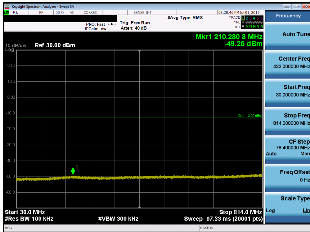
Plot 7-24. Conducted Spurious Plot (LTE Band 26, 15MHz QPSK – RB Size 1, RB Offset 0 – Low Channel)
