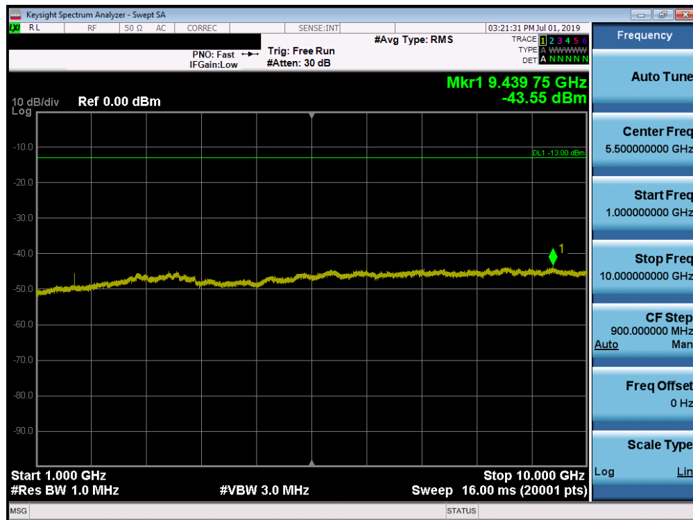
Plot 7-26. Conducted Spurious Plot (LTE Band 26, 15MHz QPSK – RB Size 1, RB Offset 0 – Low Channel)
