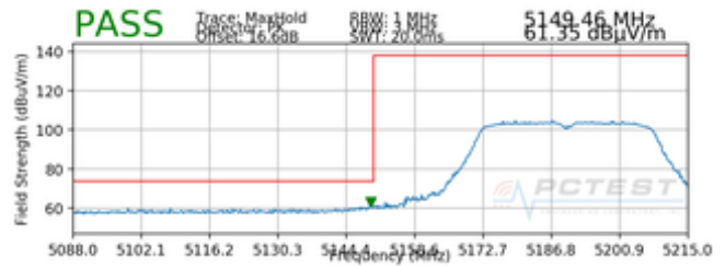
Plot 7-81. Radiated Lower Band Edge Plot (Peak – UNII Band 1)
