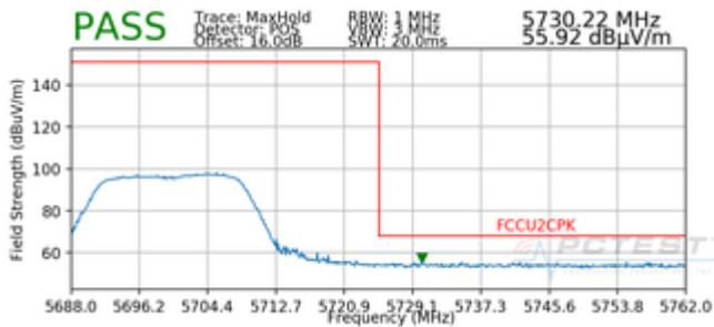
Plot 7-89. Radiated Upper Band Edge Plot SISO ANT1 (Peak – UNII Band 2C)
