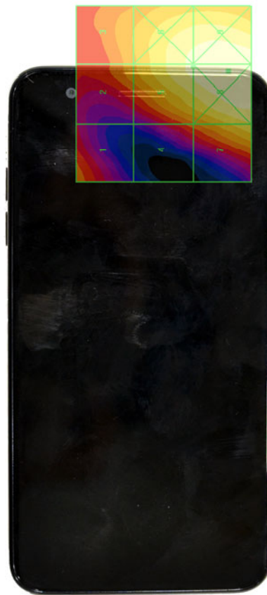
Figure 17-4 E-Field WD Scan overlay (Pictured with T-coil Centered Scan Area)
