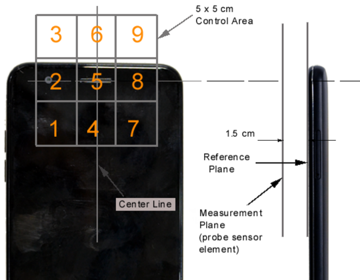
Figure 17-3 5x5 Scan grid above WD (Pictured with Acoustic Centered Scan Area)
