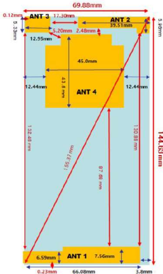
Rear view
