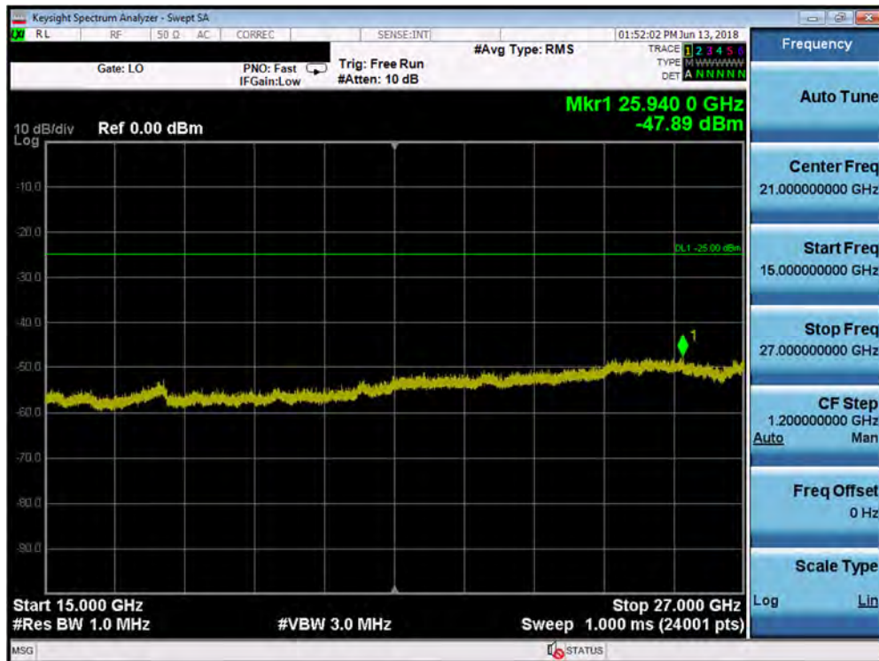
Plot 7-122. Conducted Spurious Plot (Band 41 PC2 - 5.0MHz QPSK - RB Size 1, RB Offset 0 - Mid Channel)
