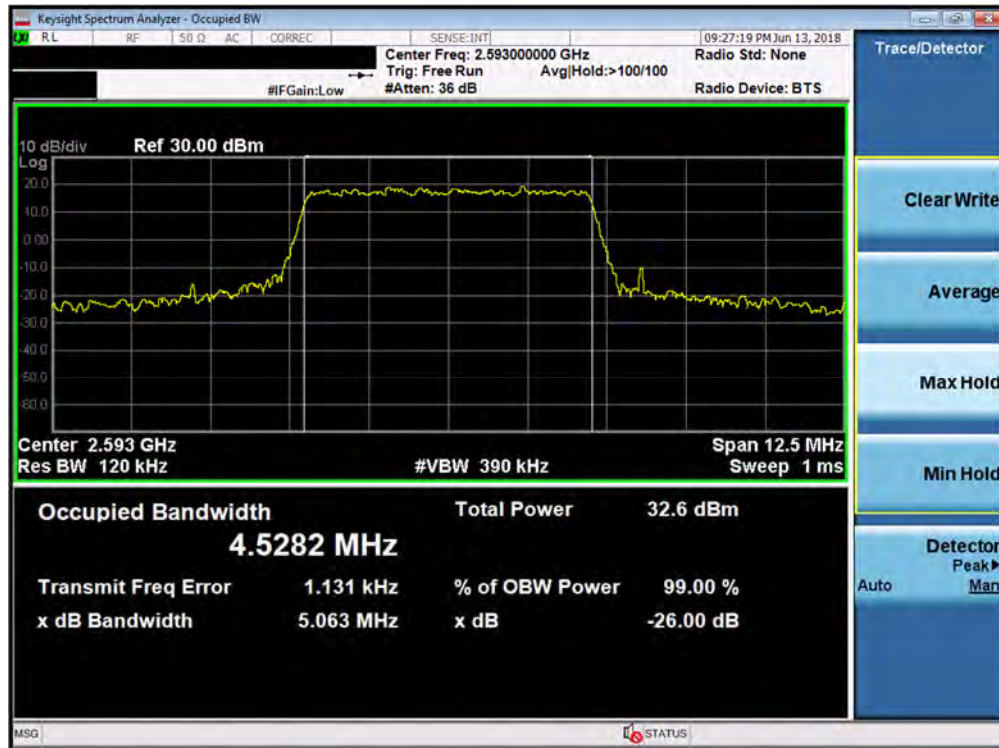
Plot 7-47. Occupied Bandwidth Plot (Band 41 PC3 - 5.0MHz QPSK - Full RB Configuration)
