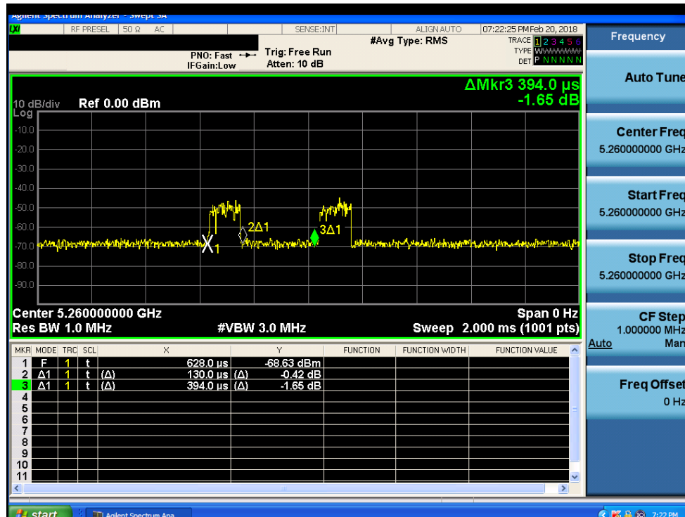
Figure 5-1. Band 2A Channel Loading Time
