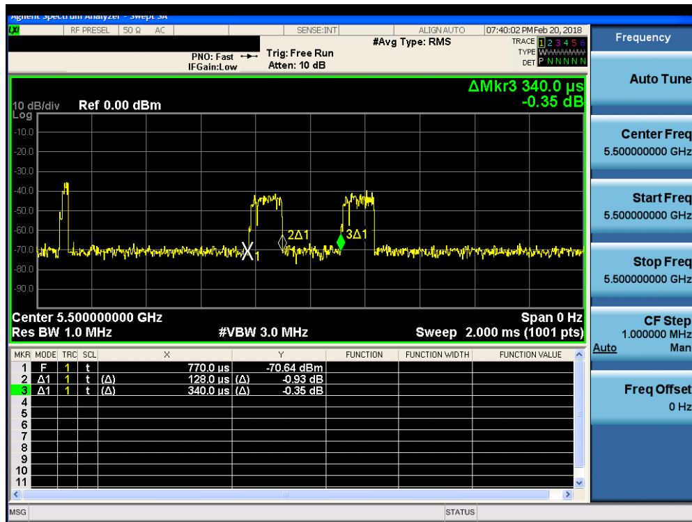
Figure 5-2. Band 2C Channel Loading Time
