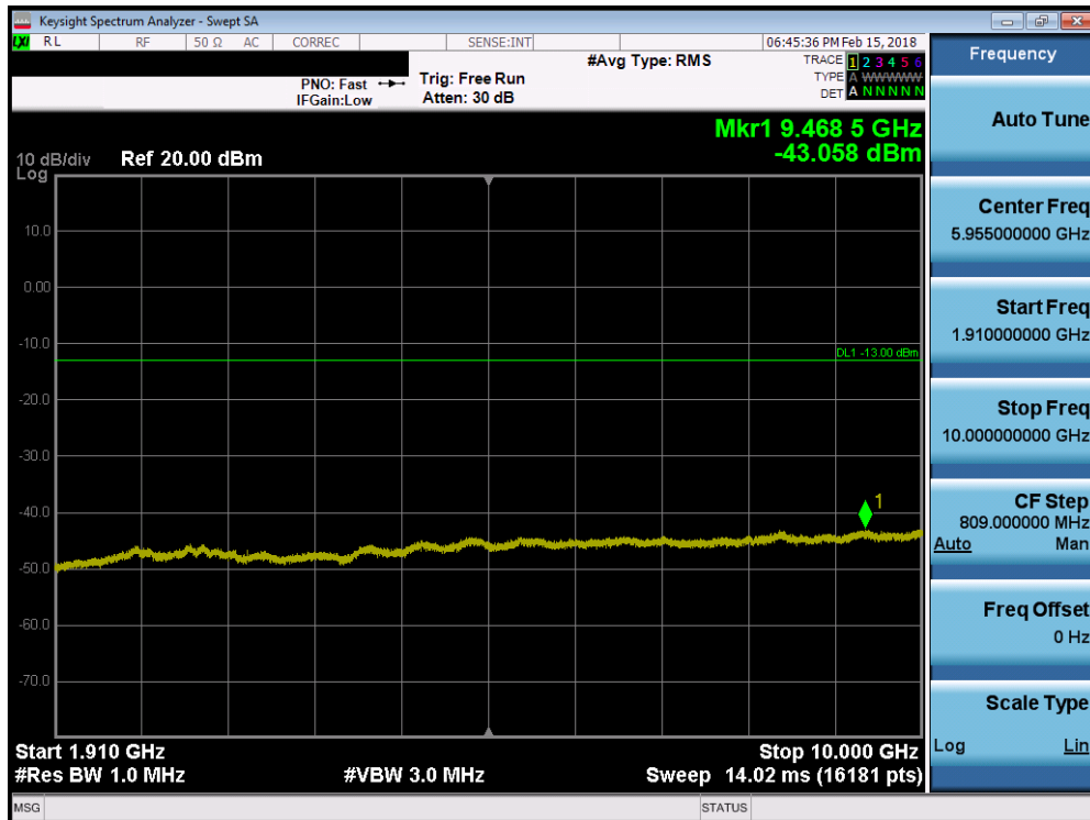
Plot 7-91. Conducted Spurious Plot (Band 2 - 5.0MHz QPSK - RB Size 1, RB Offset 0 - Low Channel)
