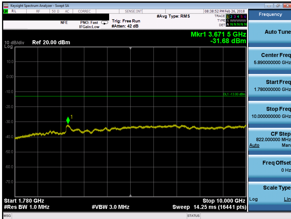
Plot 7-82. Conducted Spurious Plot (Band 66/4 - 10.0MHz QPSK - RB Size 1, RB Offset 0 - Low Channel)
