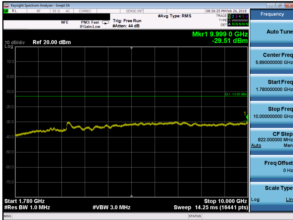
Plot 7-85. Conducted Spurious Plot (Band 66/4 - 10.0MHz QPSK - RB Size 1, RB Offset 0 - Mid Channel)
