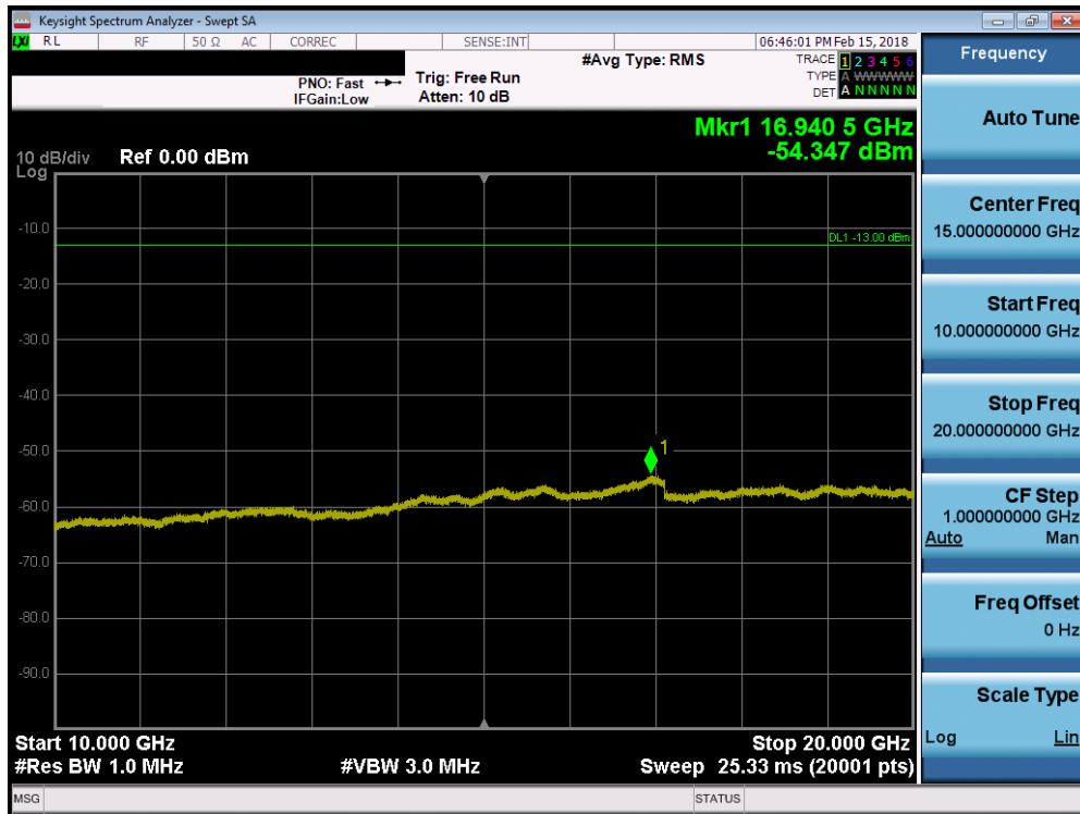
Plot 7-92. Conducted Spurious Plot (Band 2 - 5.0MHz QPSK - RB Size 1, RB Offset 0 - Low Channel)
