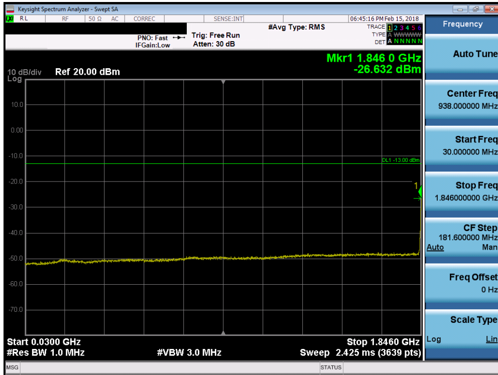
Plot 7-90. Conducted Spurious Plot (Band 2 - 5.0MHz QPSK - RB Size 1, RB Offset 0 - Low Channel)
