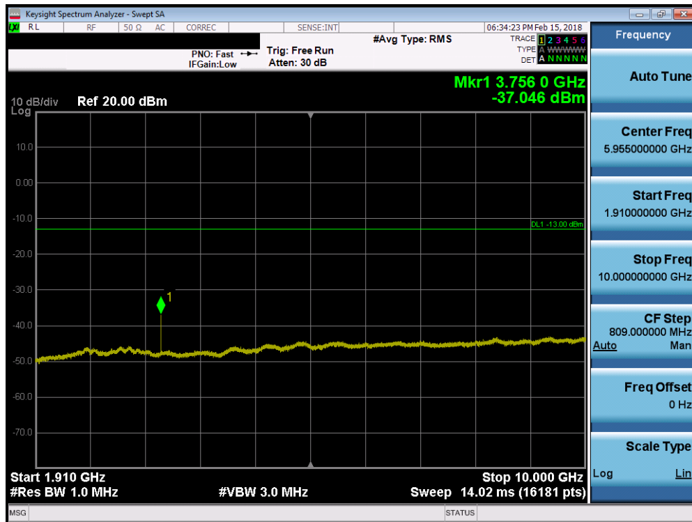
Plot 7-94. Conducted Spurious Plot (Band 2 - 5.0MHz QPSK - RB Size 1, RB Offset 0 - Mid Channel)
