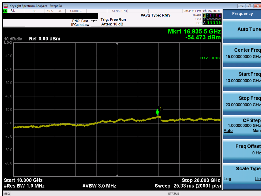
Plot 7-95. Conducted Spurious Plot (Band 2 - 5.0MHz QPSK - RB Size 1, RB Offset 0 - Mid Channel)
