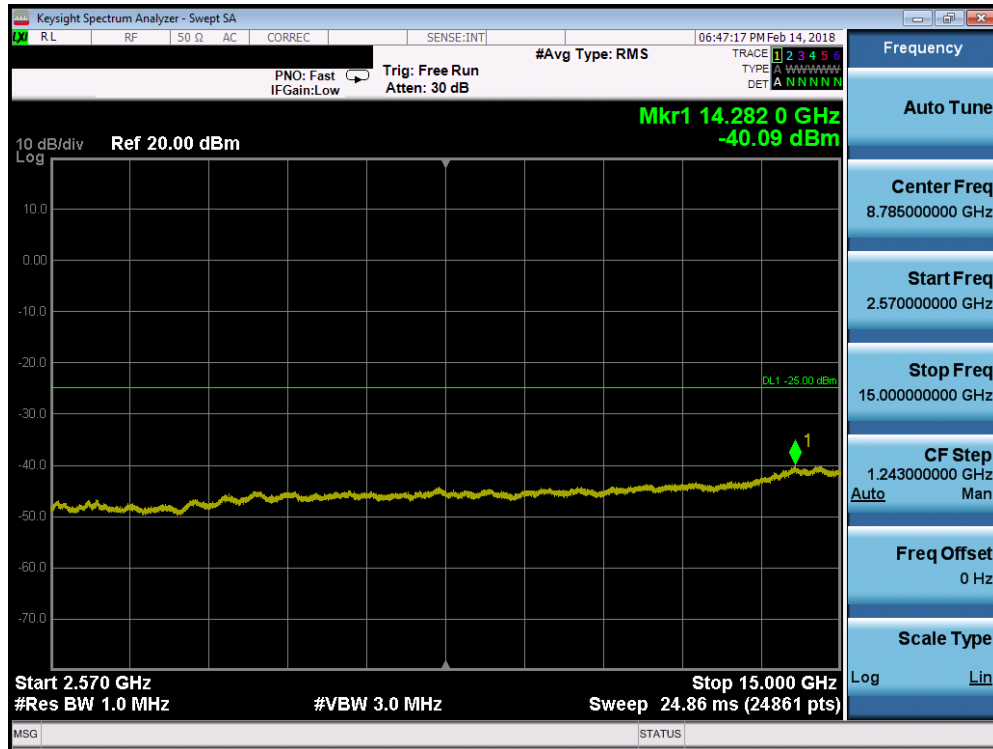
Plot 7-103. Conducted Spurious Plot (Band 7 - 15.0MHz QPSK - RB Size 1, RB Offset 0 - Mid Channel)
