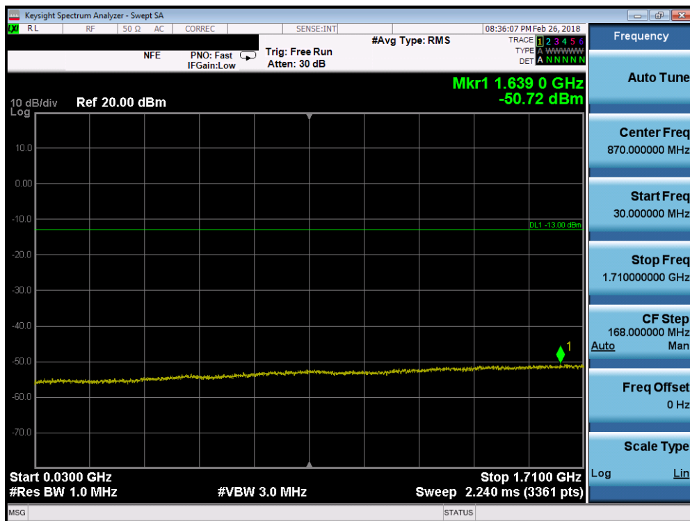
Plot 7-84. Conducted Spurious Plot (Band 66/4 - 10.0MHz QPSK - RB Size 1, RB Offset 0 - Mid Channel)
