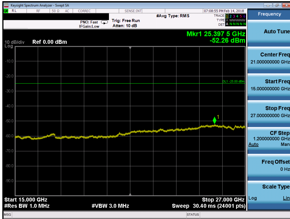
Plot 7-107. Conducted Spurious Plot (Band 7 - 15.0MHz QPSK - RB Size 1, RB Offset 0 - High Channel)
