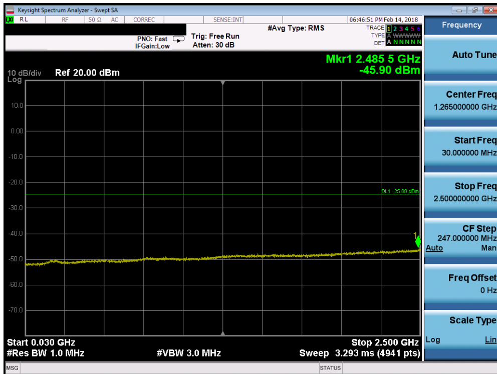
Plot 7-102. Conducted Spurious Plot (Band 7 - 15.0MHz QPSK - RB Size 1, RB Offset 0 - Mid Channel)
