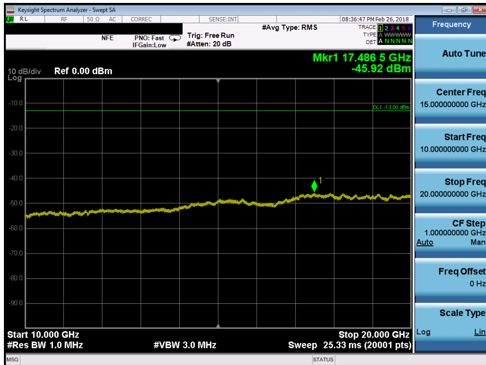
Plot 7-86. Conducted Spurious Plot (Band 66/4 - 10.0MHz QPSK - RB Size 1, RB Offset 0 - Mid Channel)
