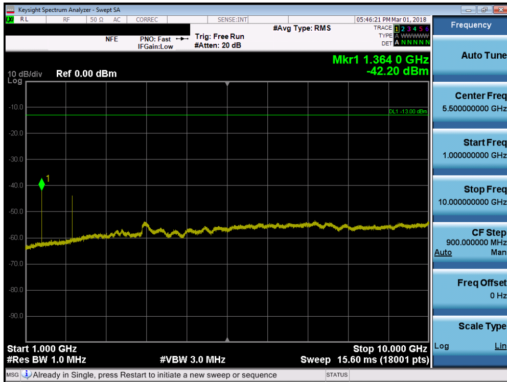
Plot 7-59. Conducted Spurious Plot (Band 71 - 20.0MHz QPSK - RB Size 1, RB Offset 0 - Low Channel)
