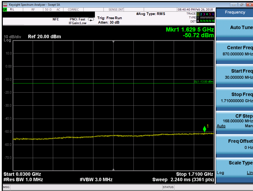
Plot 7-87. Conducted Spurious Plot (Band 66/4 - 10.0MHz QPSK - RB Size 1, RB Offset 0 - High Channel)
