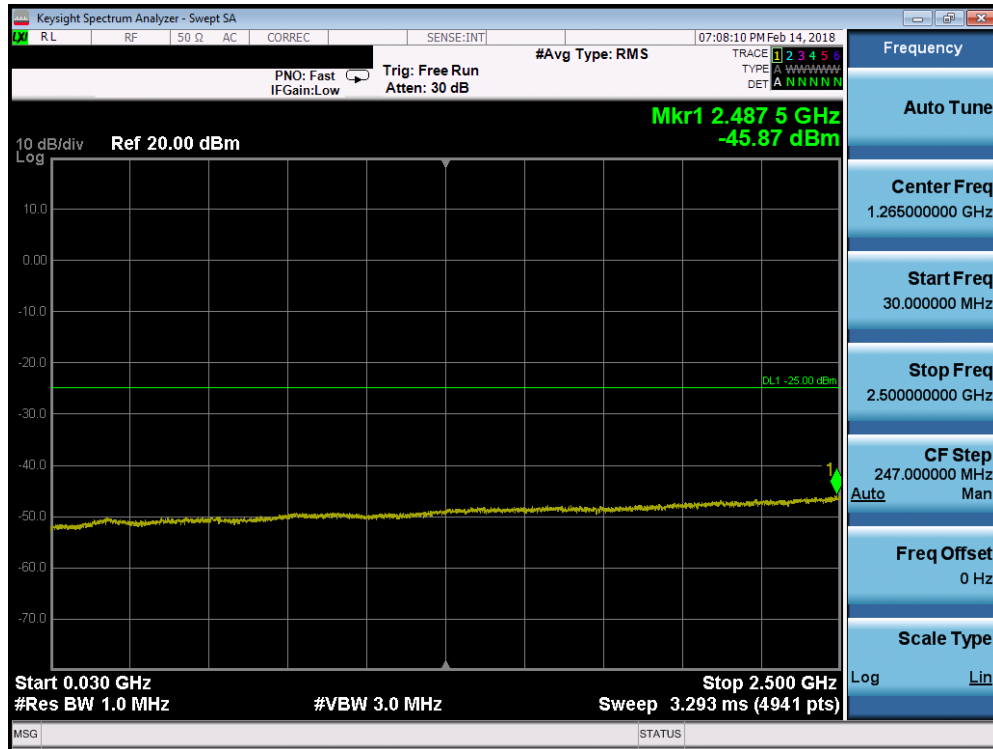
Plot 7-105. Conducted Spurious Plot (Band 7 - 15.0MHz QPSK - RB Size 1, RB Offset 0 - High Channel)
