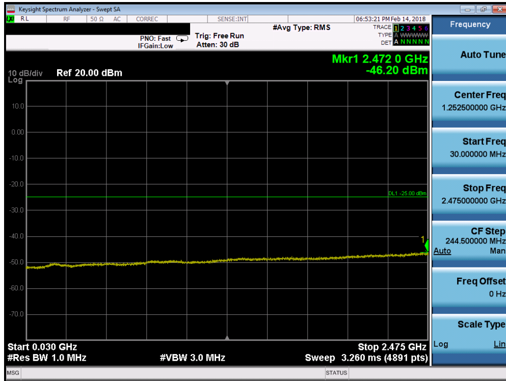
Plot 7-99. Conducted Spurious Plot (Band 7 - 15.0MHz QPSK - RB Size 1, RB Offset 0 - Low Channel)
