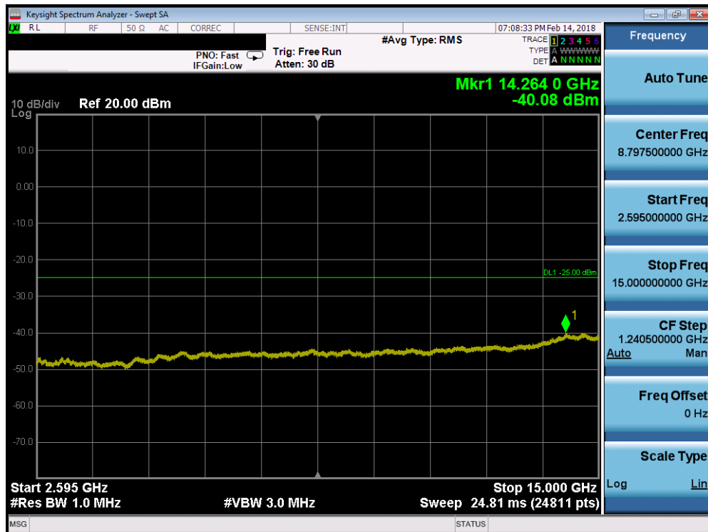
Plot 7-106. Conducted Spurious Plot (Band 7 - 15.0MHz QPSK - RB Size 1, RB Offset 0 - High Channel)
