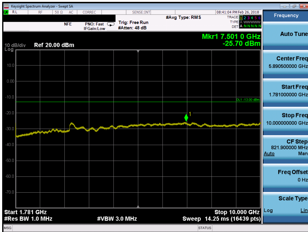
Plot 7-88. Conducted Spurious Plot (Band 66/4 - 10.0MHz QPSK - RB Size 1, RB Offset 0 - High Channel)
