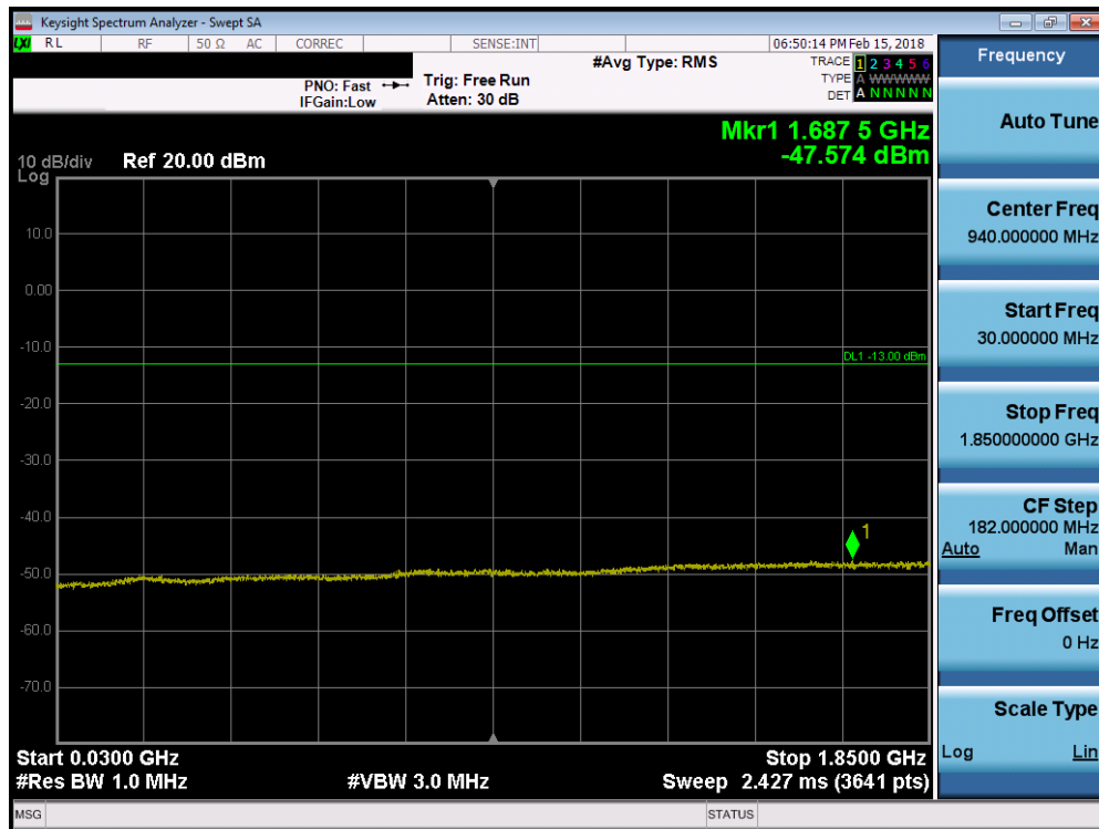
Plot 7-96. Conducted Spurious Plot (Band 2 - 5.0MHz QPSK - RB Size 1, RB Offset 0 - High Channel)
