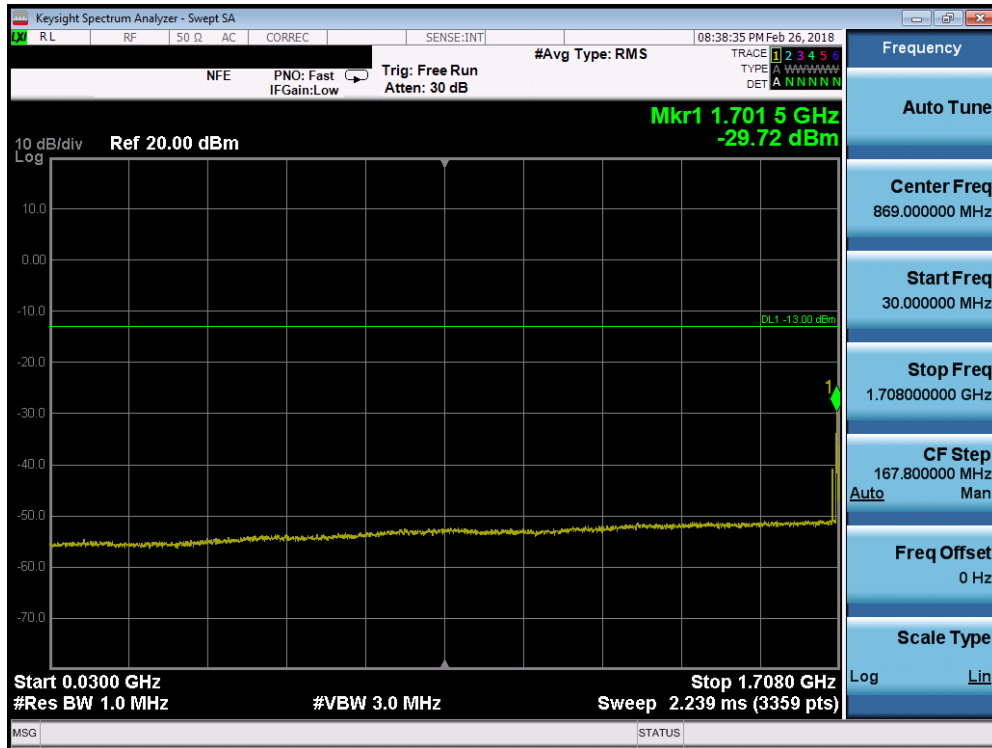
Plot 7-81. Conducted Spurious Plot (Band 66/4 - 10.0MHz QPSK - RB Size 1, RB Offset 0 - Low Channel)
