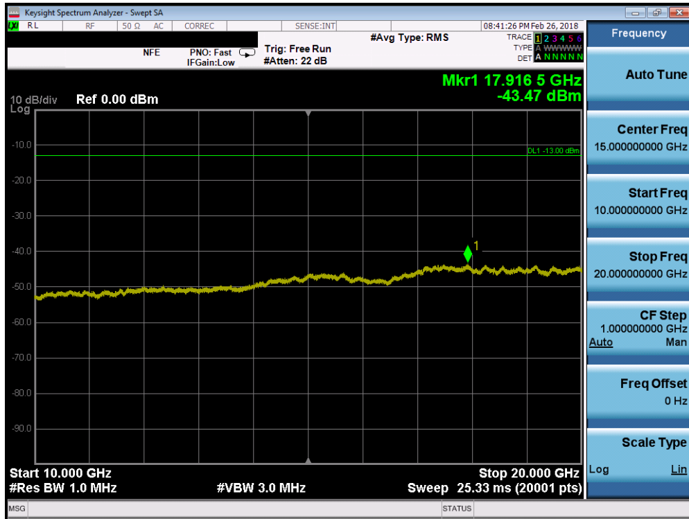
Plot 7-89. Conducted Spurious Plot (Band 66/4 - 10.0MHz QPSK - RB Size 1, RB Offset 0 - High Channel)
