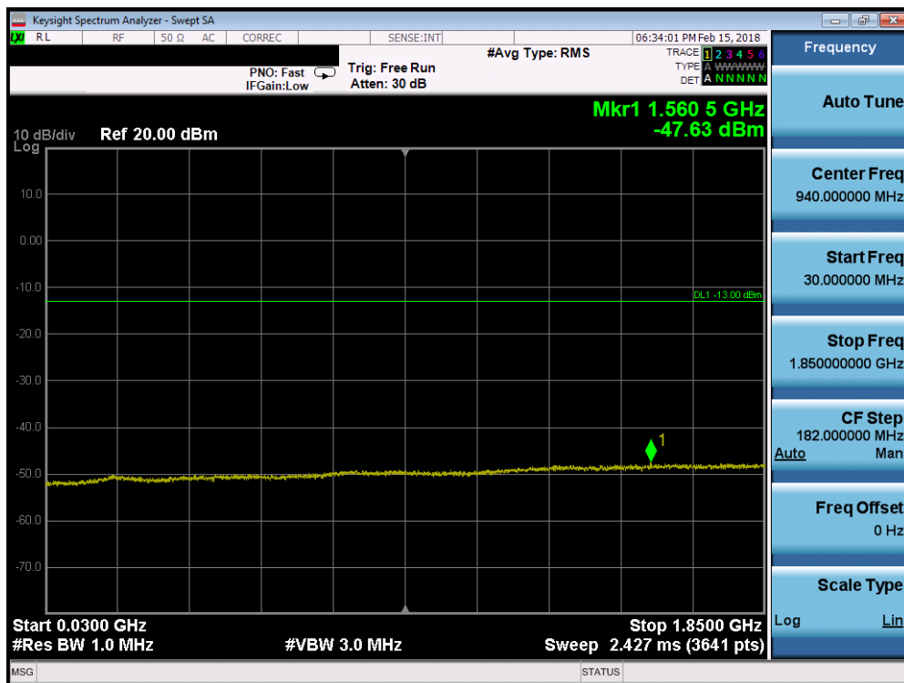
Plot 7-93. Conducted Spurious Plot (Band 2 - 5.0MHz QPSK - RB Size 1, RB Offset 0 - Mid Channel)
