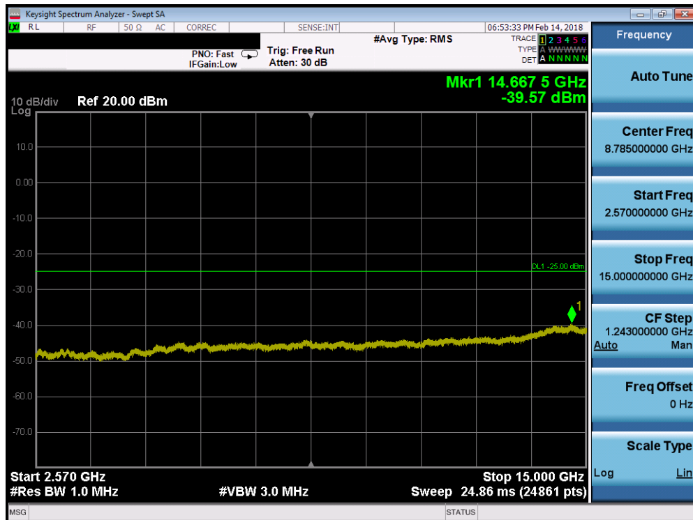
Plot 7-100. Conducted Spurious Plot (Band 7 - 15.0MHz QPSK - RB Size 1, RB Offset 0 - Low Channel)
