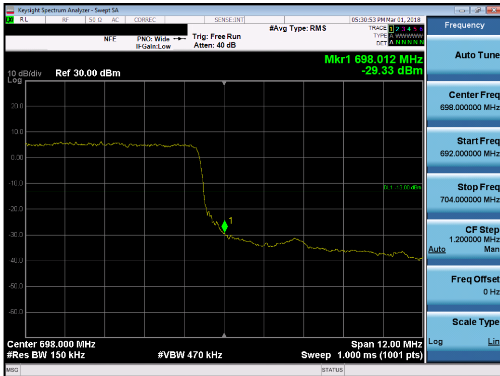
Plot 7-113. Upper Band Edge Plot (Band 71 - 15.0MHz QPSK - Full RB Configuration)
