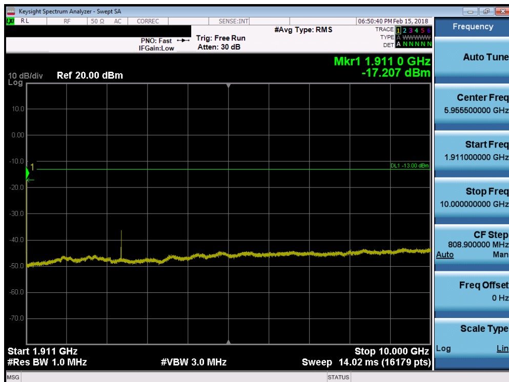
Plot 7-97. Conducted Spurious Plot (Band 2 - 5.0MHz QPSK - RB Size 1, RB Offset 0 - High Channel)
