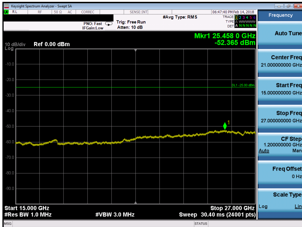
Plot 7-104. Conducted Spurious Plot (Band 7 - 15.0MHz QPSK - RB Size 1, RB Offset 0 - Mid Channel)
