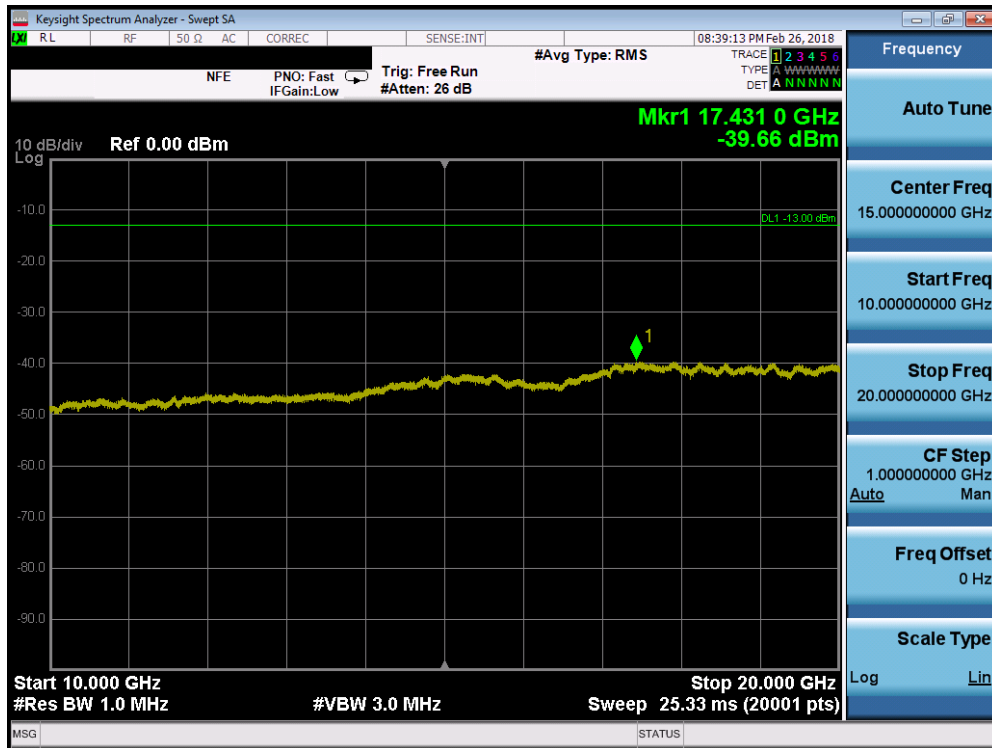
Plot 7-83. Conducted Spurious Plot (Band 66/4 - 10.0MHz QPSK - RB Size 1, RB Offset 0 - Low Channel)
