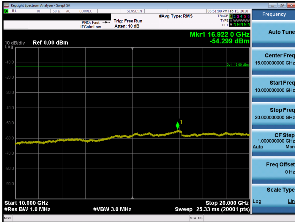
Plot 7-98. Conducted Spurious Plot (Band 2 - 5.0MHz QPSK - RB Size 1, RB Offset 0 - High Channel)
