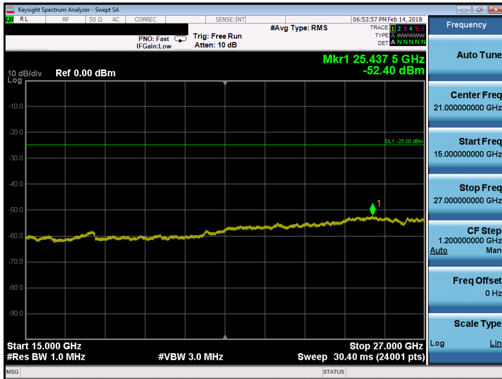
Plot 7-101. Conducted Spurious Plot (Band 7 - 15.0MHz QPSK - RB Size 1, RB Offset 0 - Low Channel)
