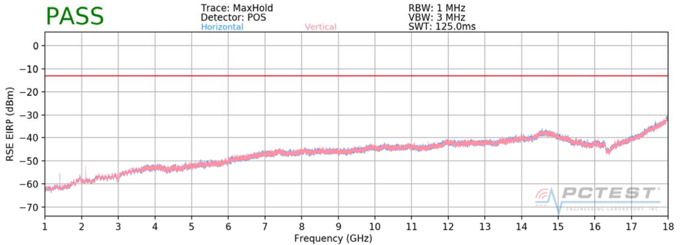
Plot 7-251. Radiated Spurious Plot above 1GHz (Band 12)
