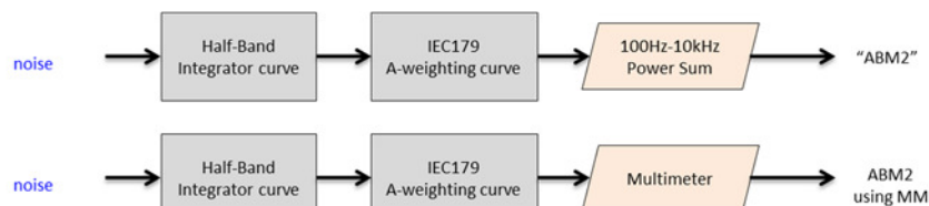
Figure 4-9 ABM2 Validation Block Diagram
