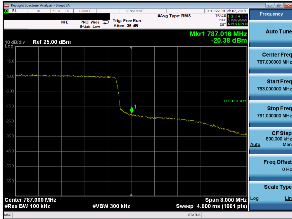
Plot 6-79. Upper Band Edge Plot (Band 13 - 10.0MHz QPSK - Full RB Configuration)
