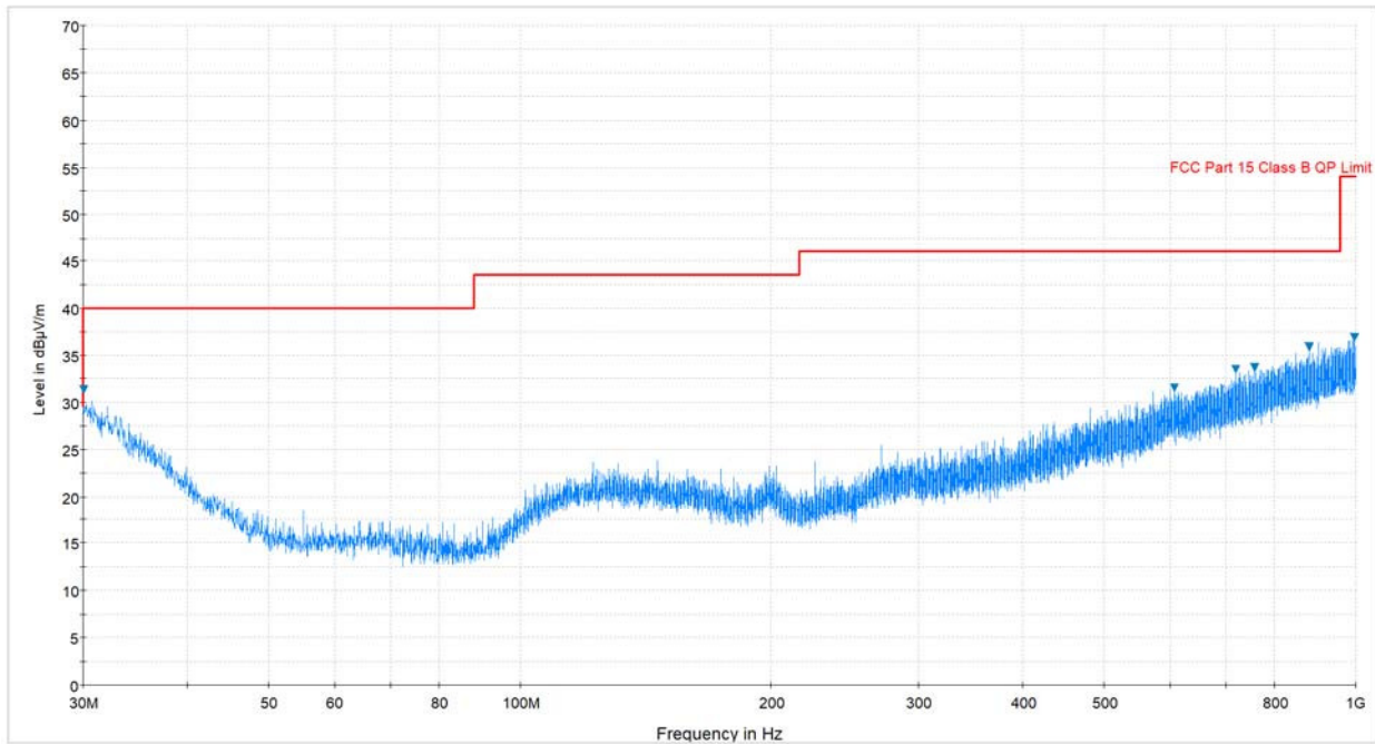
Plot 7-49. Radiated Spurious Emissions Plot (Below 1GHz, V)
