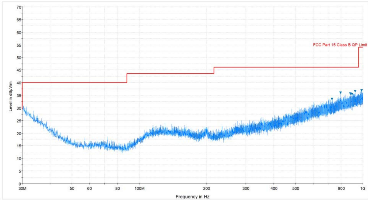
Plot 7-48. Radiated Spurious Emissions Plot (Below 1GHz, H)
