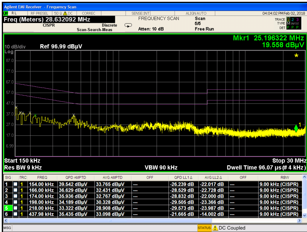
Plot 7-51. Line-Conducted Test Plot (N)
