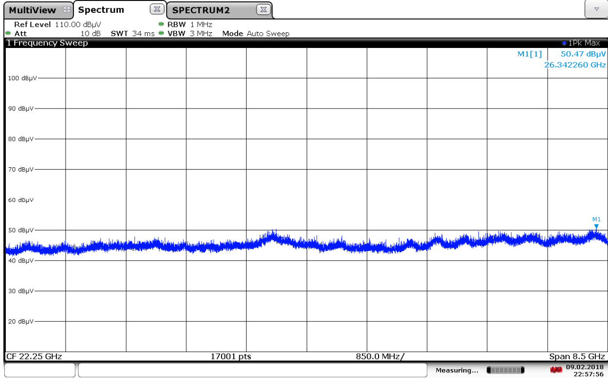
Plot 7-45. Radiated Spurious Plot above 18GHz
