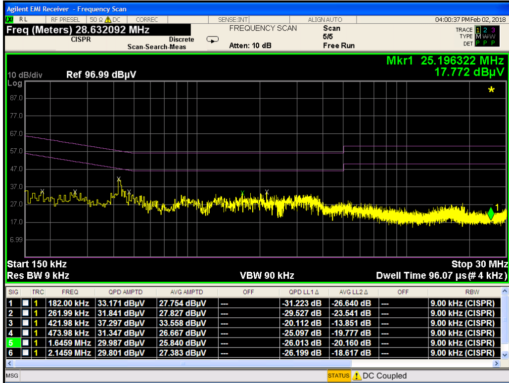
Plot 7-50. Line-Conducted Test Plot (L1)
