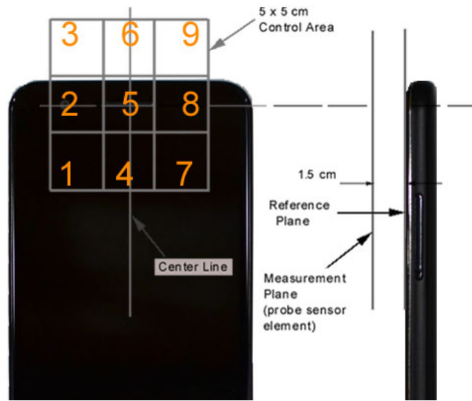
Figure 16-3 5x5 Scan grid above WD
