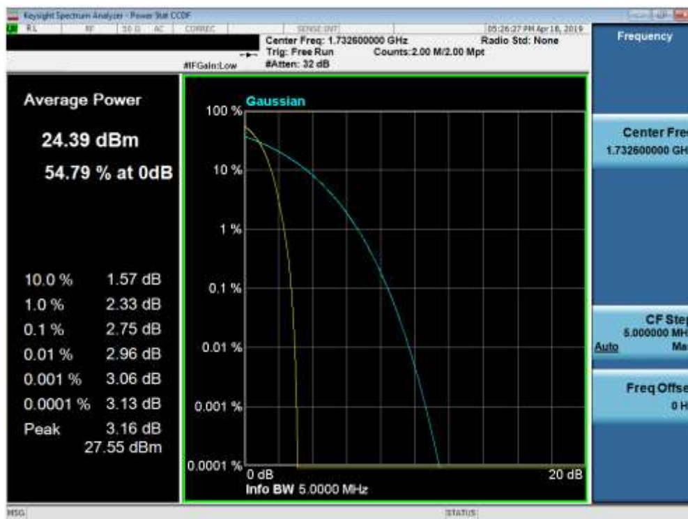
Plot 7-69. Peak-Average Ratio Plot (AWS WCDMA Mode)
