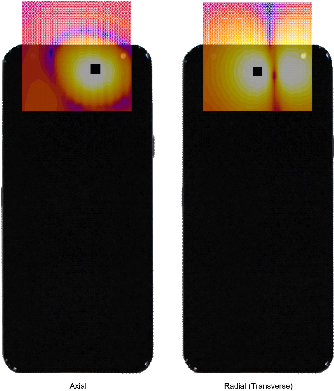
Figure 16-3 CMRS T-Coil Scan Overlay Magnetic Field Distributions
