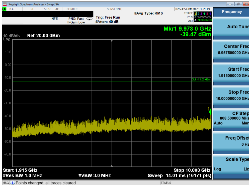
Plot 7-82. Conducted Spurious Plot (Band 25/2 - 1.4MHz QPSK - RB Size 1, RB Offset 0 - Low Channel)
