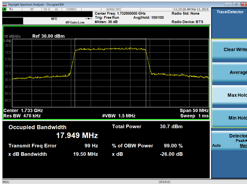
Plot 7-32. Occupied Bandwidth Plot (Band 4 - 20.0MHz 16-QAM - Full RB Configuration)
