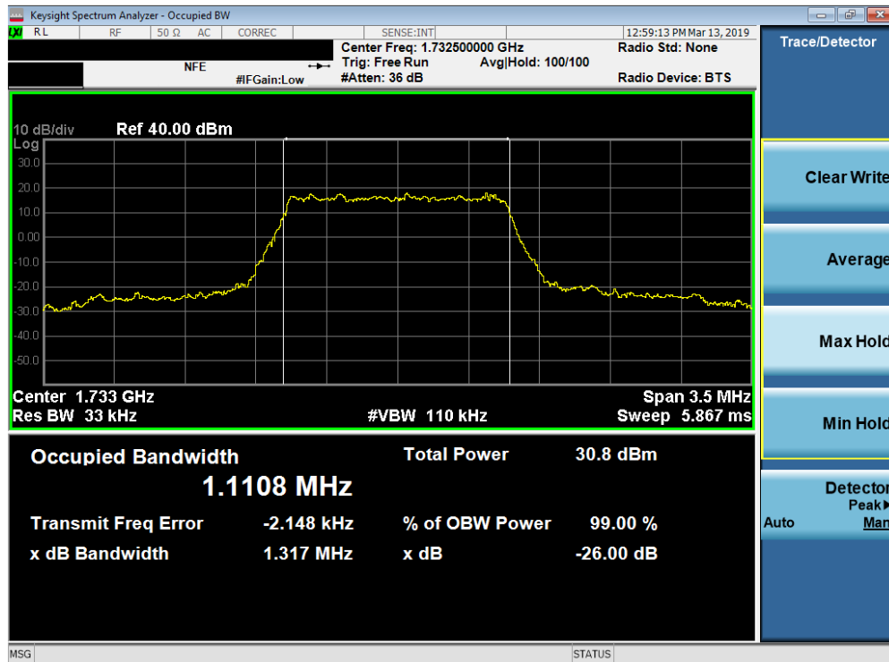
Plot 7-22. Occupied Bandwidth Plot (Band 4 - 1.4MHz 16-QAM - Full RB Configuration)
