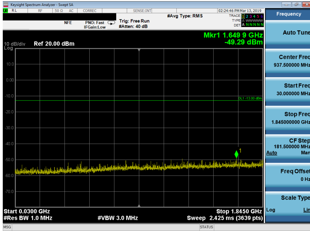
Plot 7-81. Conducted Spurious Plot (Band 25/2 - 1.4MHz QPSK - RB Size 1, RB Offset 0 - Low Channel)
