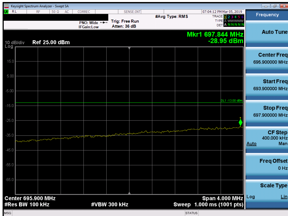
Plot 7-103. Lower Extended Band Edge Plot (Band 12 - 10.0MHz QPSK - Full RB Configuration)
