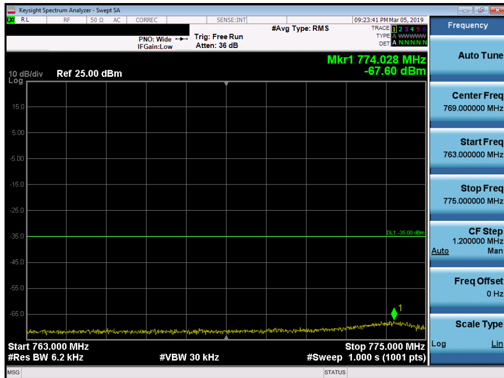
Plot 7-111. Lower Emission Mask Plot (Band 13 - 10.0MHz QPSK - Full RB Configuration)
