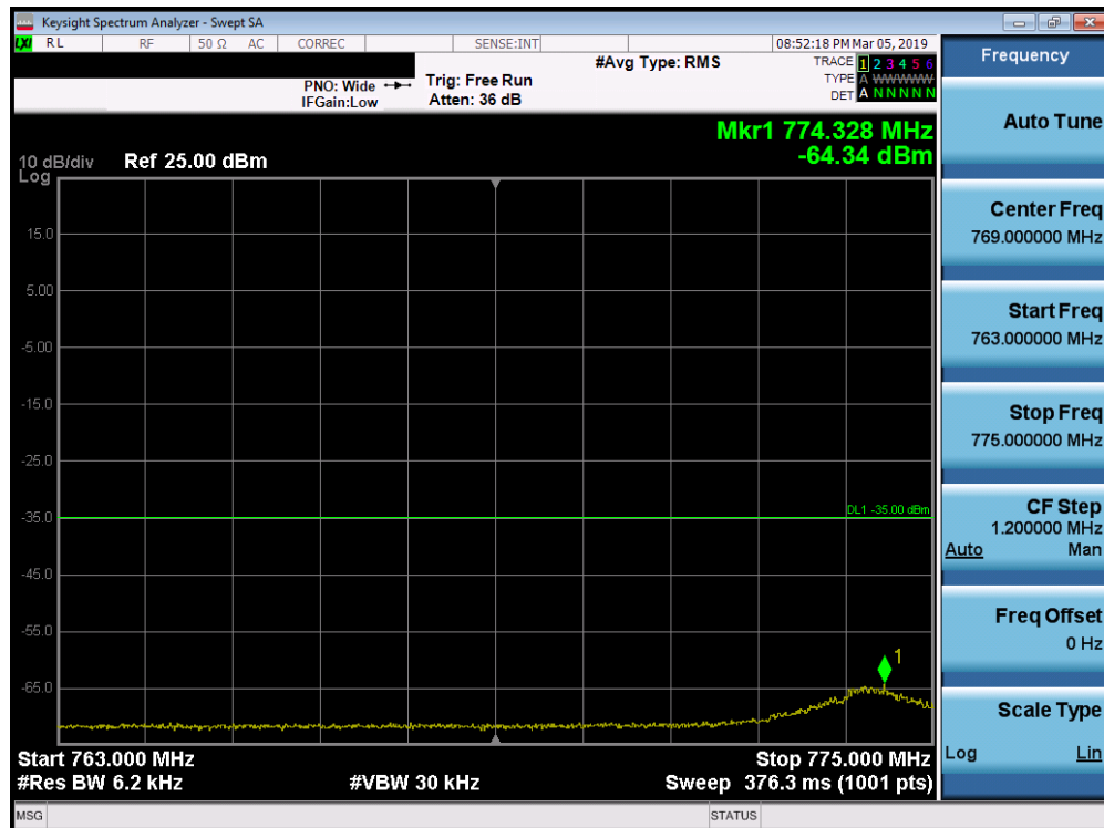
Plot 7-107. Lower Emission Mask Plot (Band 13 - 5.0MHz QPSK - Full RB Configuration)
