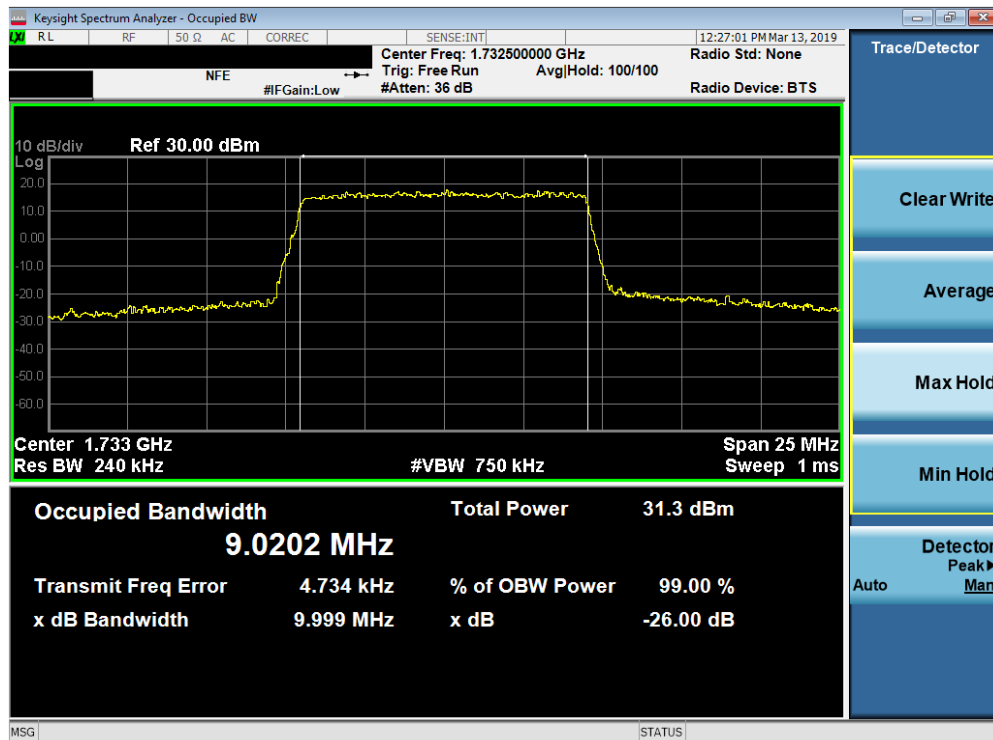
Plot 7-28. Occupied Bandwidth Plot (Band 4 - 10.0MHz 16-QAM - Full RB Configuration)
