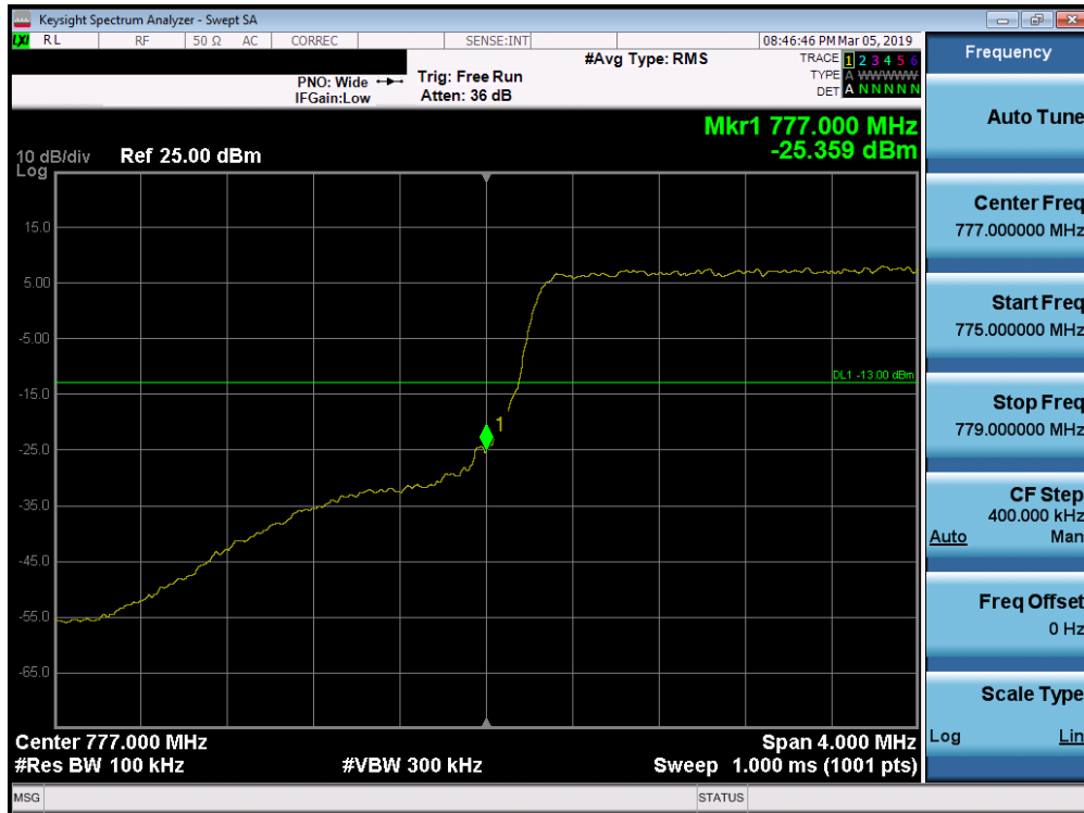
Plot 7-106. Lower Band Edge Plot (Band 13 - 5.0MHz QPSK - Full RB Configuration)
