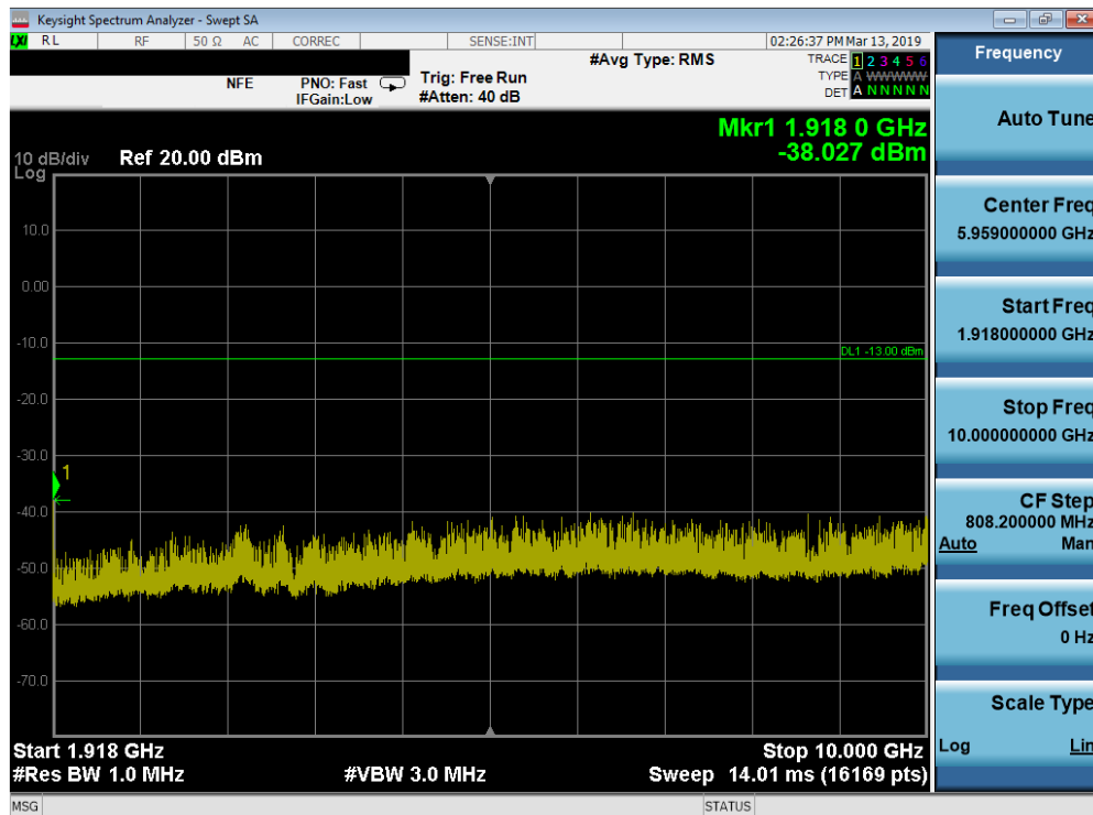
Plot 7-88. Conducted Spurious Plot (Band 25/2 - 1.4MHz QPSK - RB Size 1, RB Offset 0 - High Channel)
