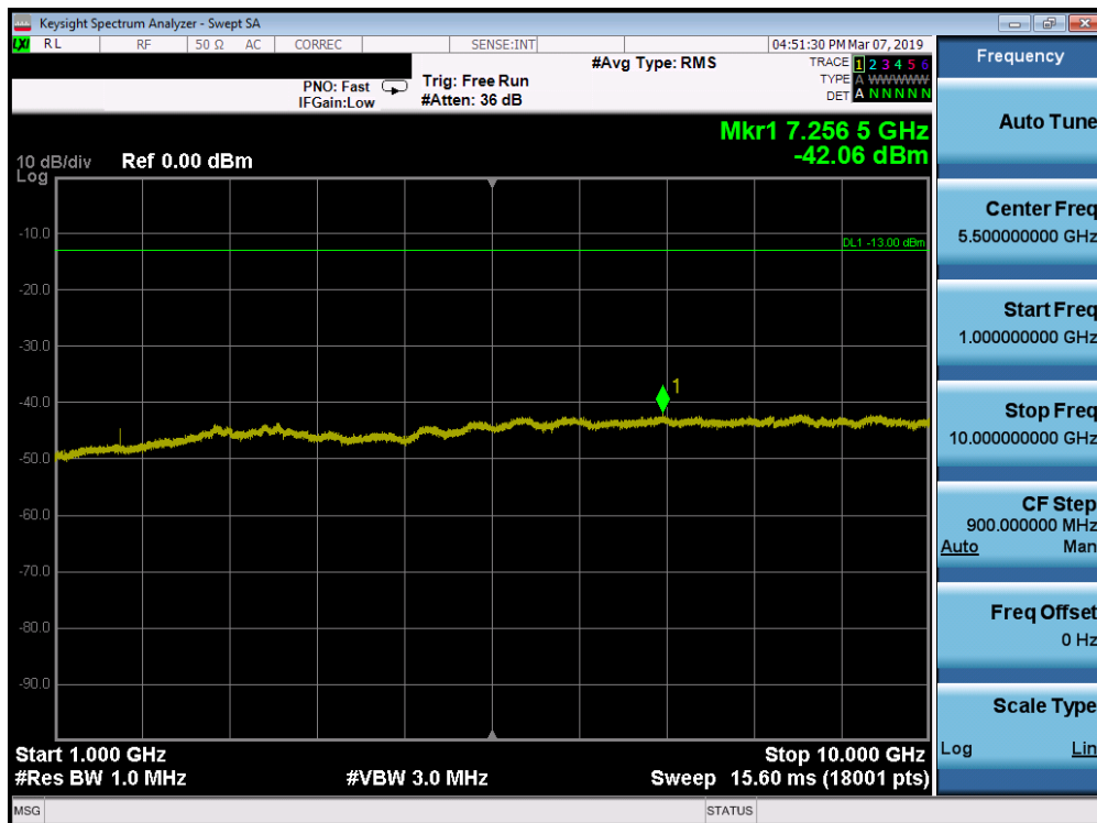
Plot 7-68. Conducted Spurious Plot (Band 5 - 1.4MHz QPSK - RB Size 1, RB Offset 0 - Mid Channel)
