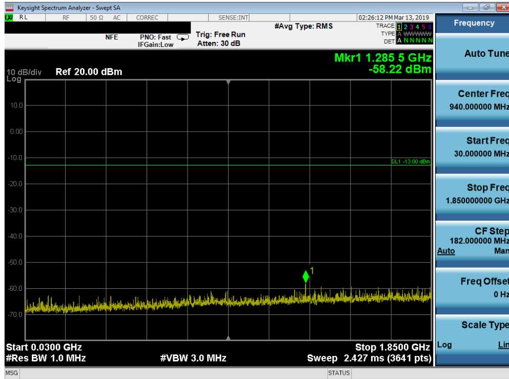
Plot 7-87. Conducted Spurious Plot (Band 25/2 - 1.4MHz QPSK - RB Size 1, RB Offset 0 - High Channel)
