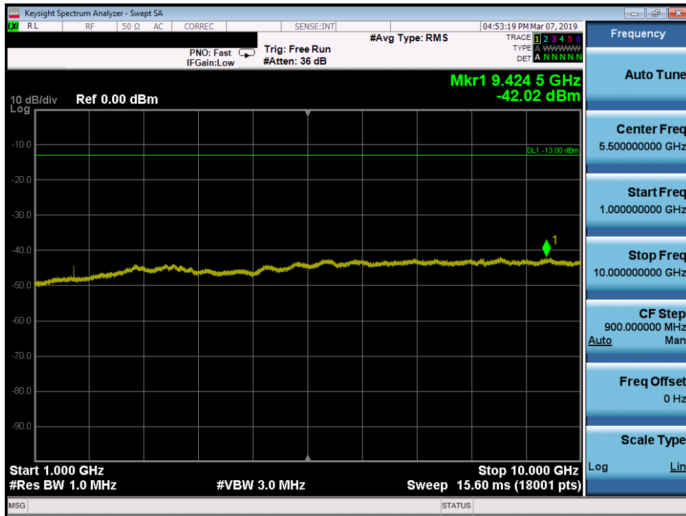
Plot 7-65. Conducted Spurious Plot (Band 5 - 1.4MHz QPSK - RB Size 1, RB Offset 0 - Low Channel)
