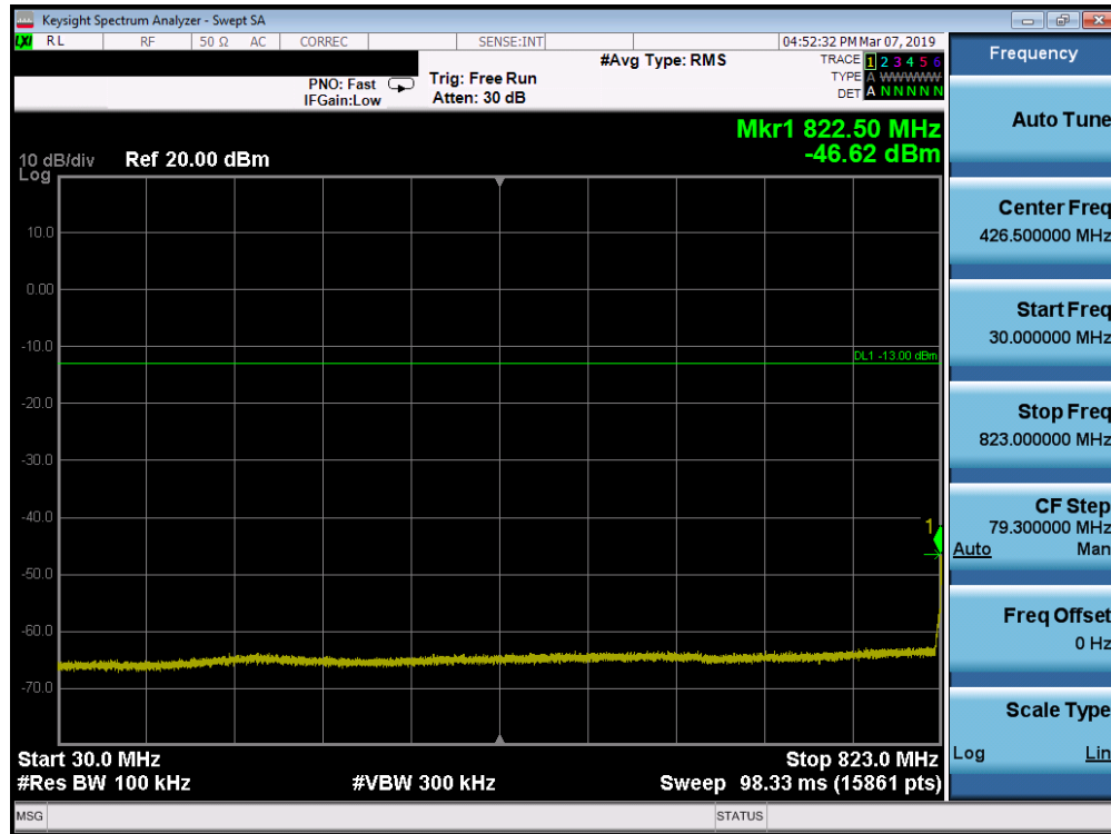
Plot 7-63. Conducted Spurious Plot (Band 5 - 1.4MHz QPSK - RB Size 1, RB Offset 0 - Low Channel)
