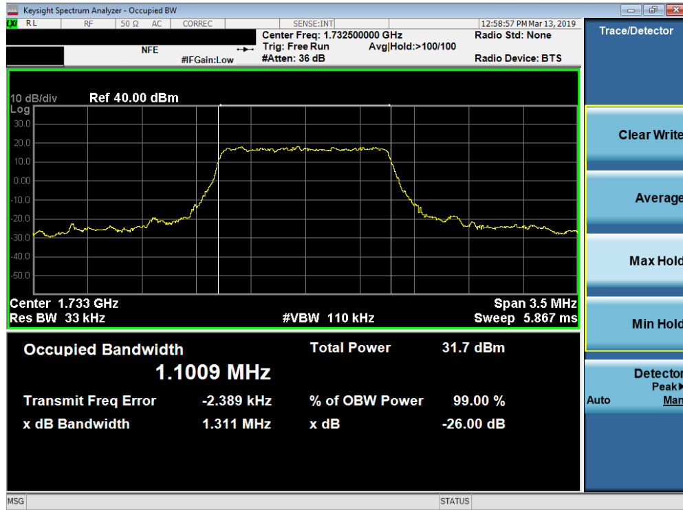
Plot 7-21. Occupied Bandwidth Plot (Band 4 - 1.4MHz QPSK - Full RB Configuration)
