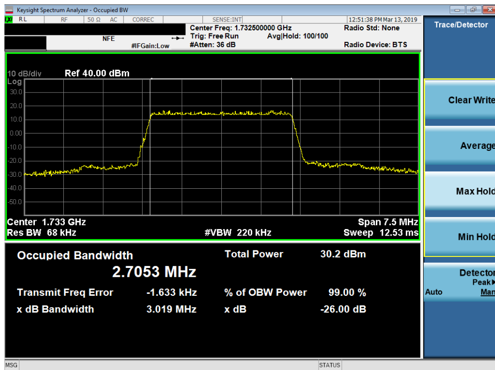
Plot 7-24. Occupied Bandwidth Plot (Band 4 - 3.0MHz 16-QAM - Full RB Configuration)
