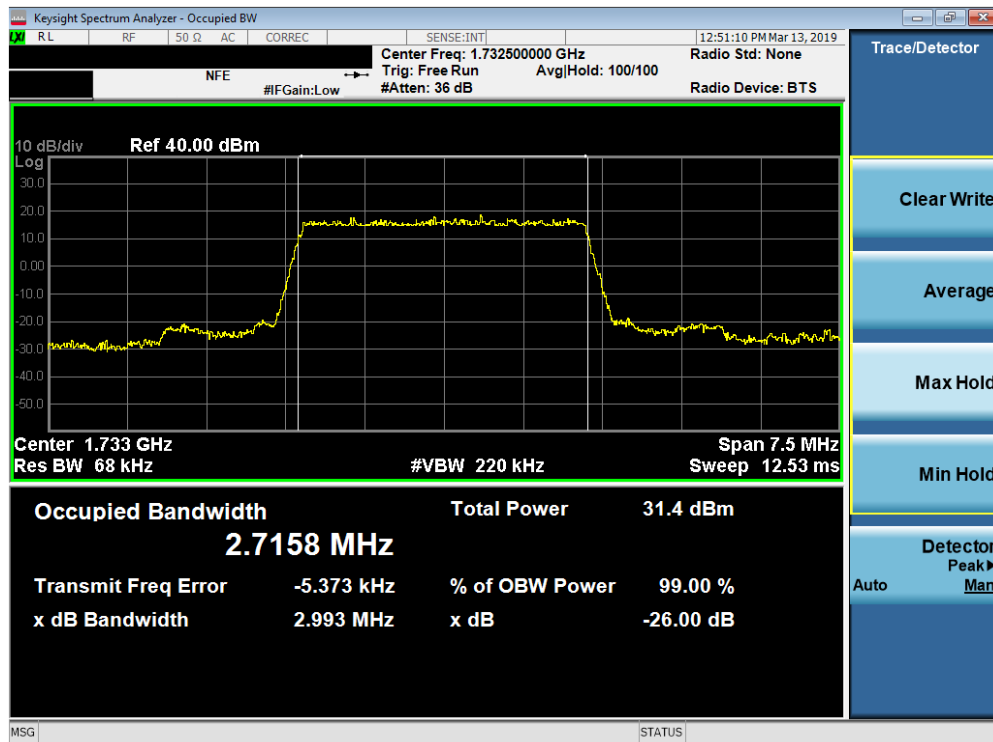
Plot 7-23. Occupied Bandwidth Plot (Band 4 - 3.0MHz QPSK - Full RB Configuration)
