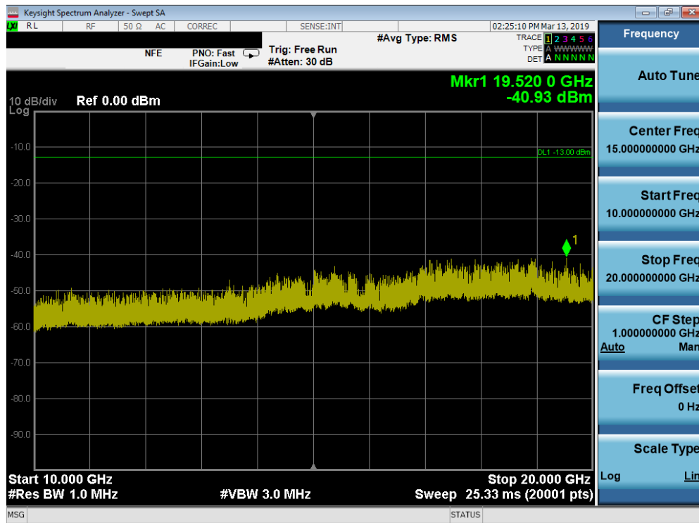
Plot 7-83. Conducted Spurious Plot (Band 25/2 - 1.4MHz QPSK - RB Size 1, RB Offset 0 - Low Channel)
