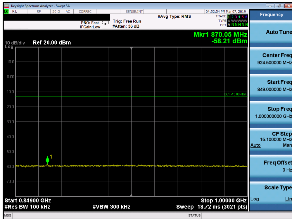
Plot 7-64. Conducted Spurious Plot (Band 5 - 1.4MHz QPSK - RB Size 1, RB Offset 0 - Low Channel)
