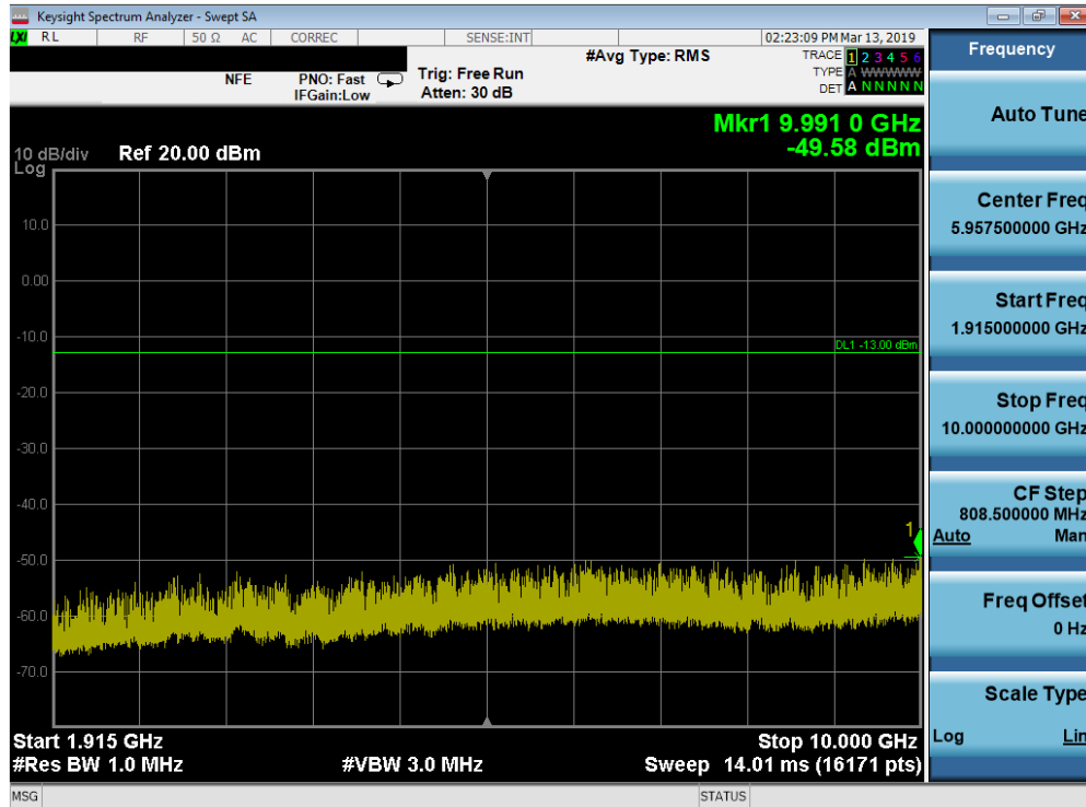
Plot 7-85. Conducted Spurious Plot (Band 25/2 - 1.4MHz QPSK - RB Size 1, RB Offset 0 - Mid Channel)
