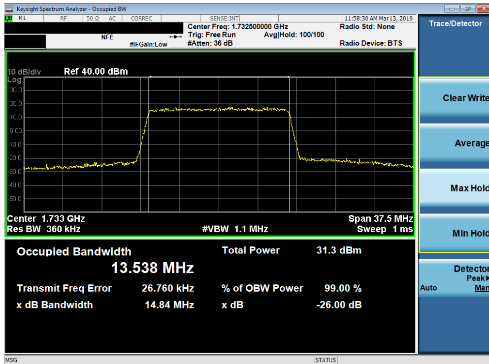
Plot 7-30. Occupied Bandwidth Plot (Band 4 - 15.0MHz 16-QAM - Full RB Configuration)
