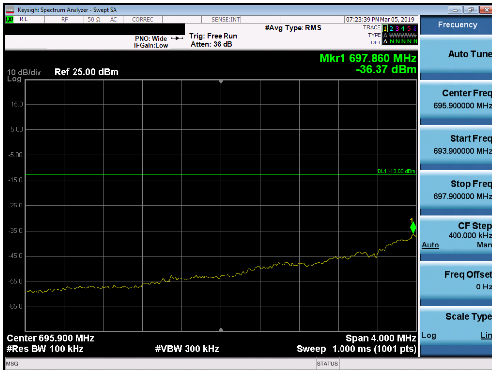
Plot 7-91. Lower Extended Band Edge Plot (Band 12 - 1.4MHz QPSK - Full RB Configuration)
