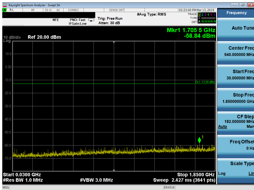
Plot 7-84. Conducted Spurious Plot (Band 25/2 - 1.4MHz QPSK - RB Size 1, RB Offset 0 - Mid Channel)
