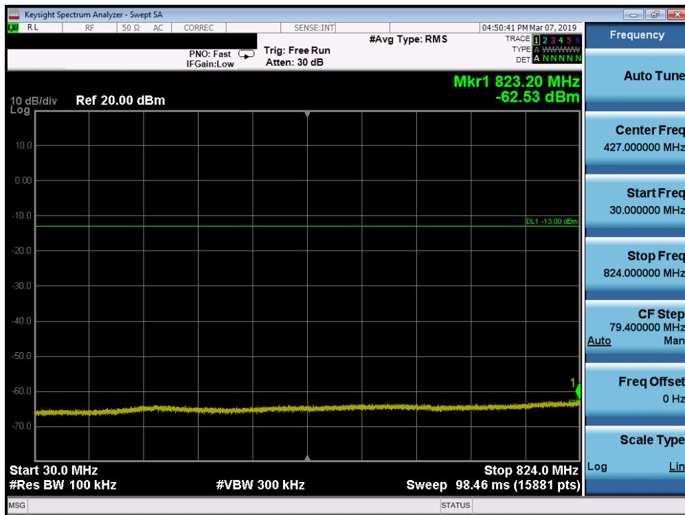
Plot 7-66. Conducted Spurious Plot (Band 5 - 1.4MHz QPSK - RB Size 1, RB Offset 0 - Mid Channel)
