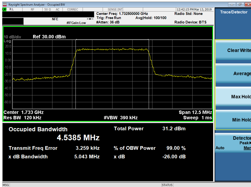
Plot 7-26. Occupied Bandwidth Plot (Band 4 - 5.0MHz 16-QAM - Full RB Configuration)
