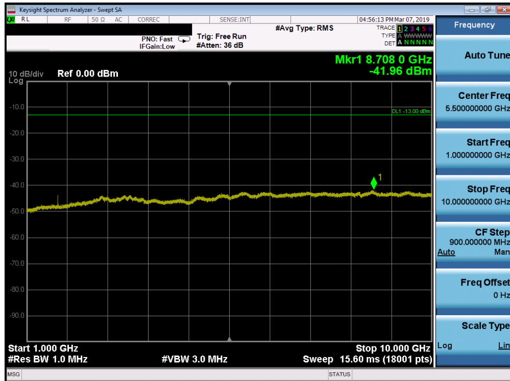
Plot 7-71. Conducted Spurious Plot (Band 5 - 1.4MHz QPSK - RB Size 1, RB Offset 0 - High Channel)
