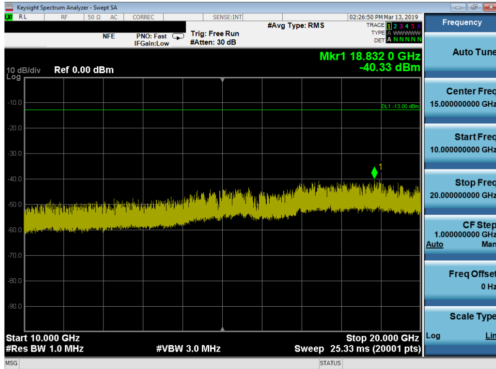
Plot 7-89. Conducted Spurious Plot (Band 25/2 - 1.4MHz QPSK - RB Size 1, RB Offset 0 - High Channel)
