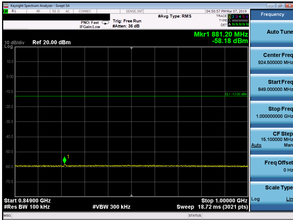
Plot 7-67. Conducted Spurious Plot (Band 5 - 1.4MHz QPSK - RB Size 1, RB Offset 0 - Mid Channel)
