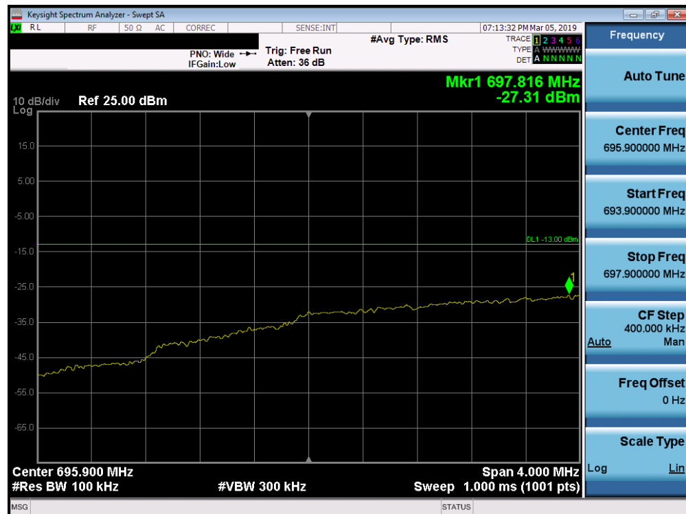
Plot 7-99. Lower Extended Band Edge Plot (Band 12 - 5.0MHz QPSK - Full RB Configuration)
