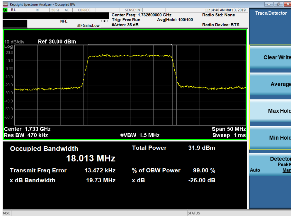
Plot 7-31. Occupied Bandwidth Plot (Band 4 - 20.0MHz QPSK - Full RB Configuration)
