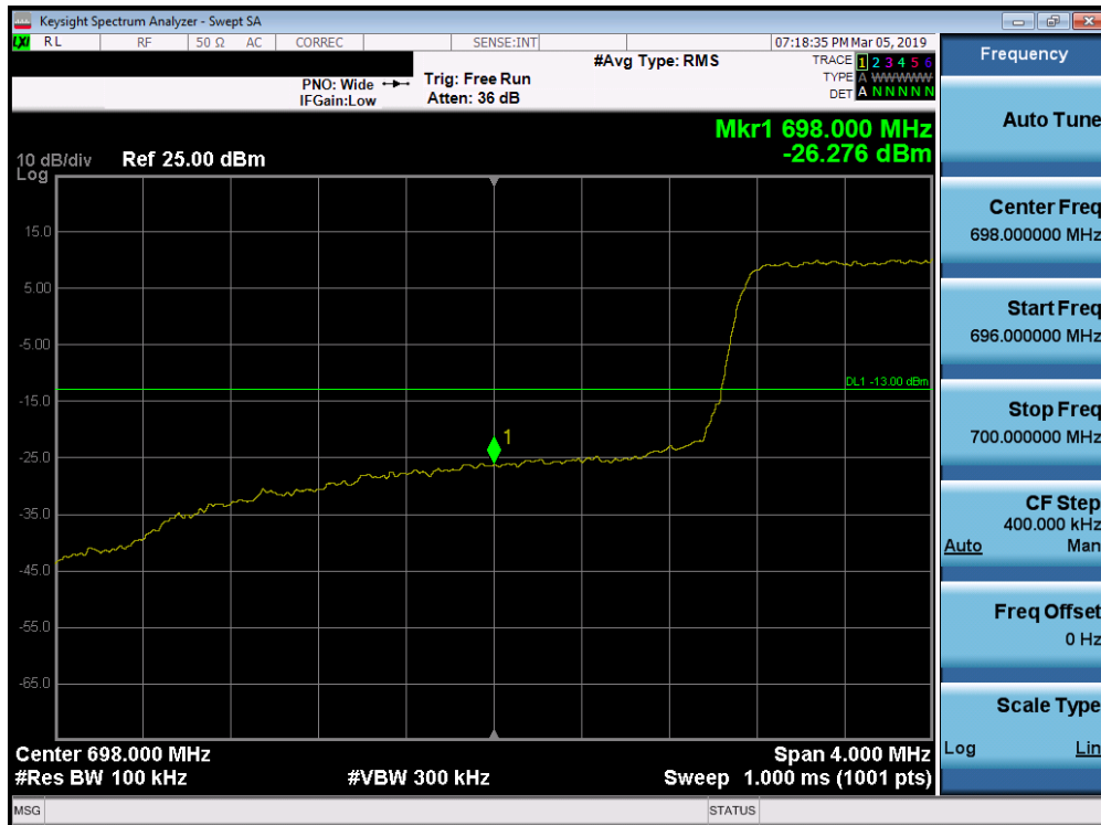
Plot 7-94. Lower Band Edge Plot (Band 12 - 3.0MHz QPSK - Full RB Configuration)
