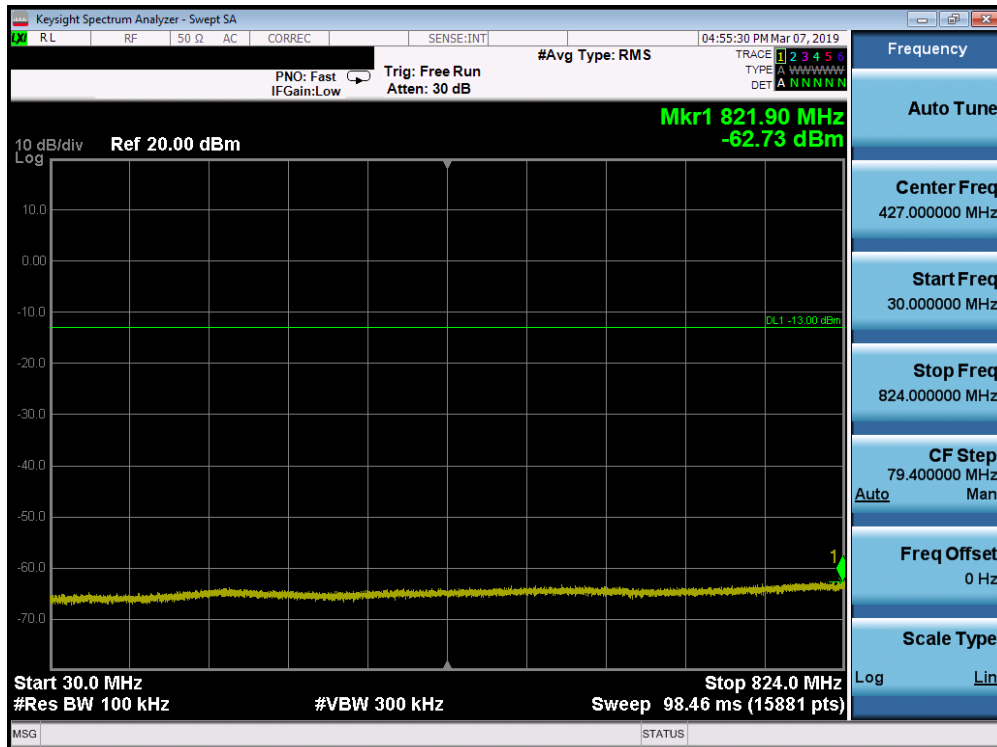
Plot 7-69. Conducted Spurious Plot (Band 5 - 1.4MHz QPSK - RB Size 1, RB Offset 0 - High Channel)
