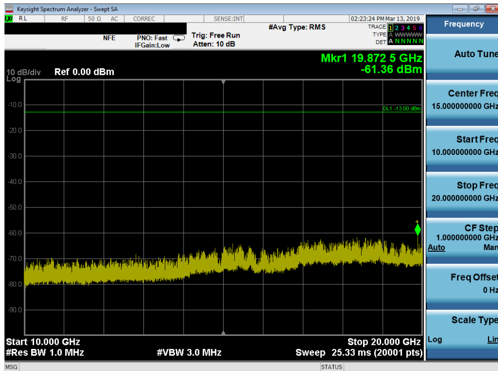
Plot 7-86. Conducted Spurious Plot (Band 25/2 - 1.4MHz QPSK - RB Size 1, RB Offset 0 - Mid Channel)
