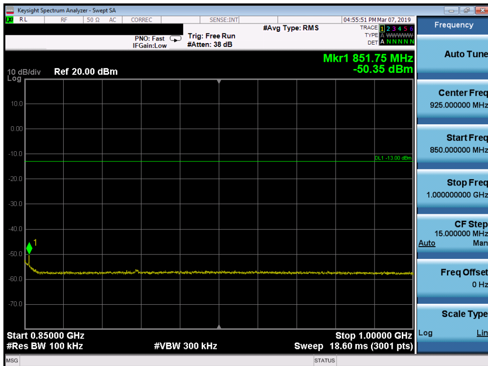
Plot 7-70. Conducted Spurious Plot (Band 5 - 1.4MHz QPSK - RB Size 1, RB Offset 0 - High Channel)
