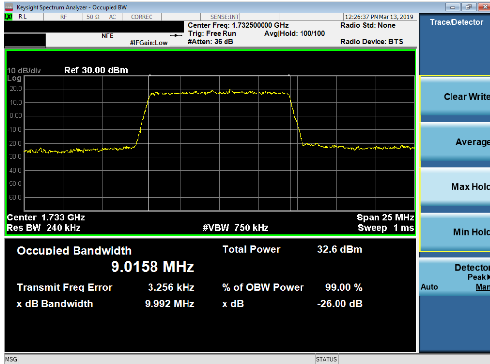
Plot 7-27. Occupied Bandwidth Plot (Band 4 - 10.0MHz QPSK - Full RB Configuration)
