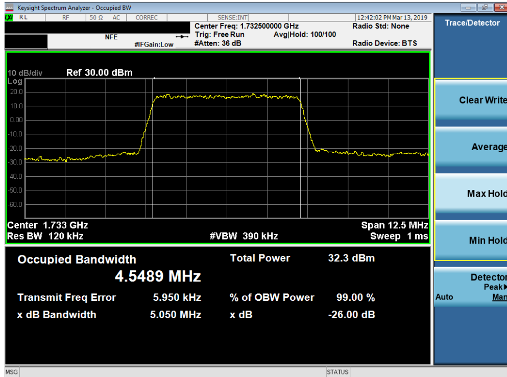
Plot 7-25. Occupied Bandwidth Plot (Band 4 - 5.0MHz QPSK - Full RB Configuration)
