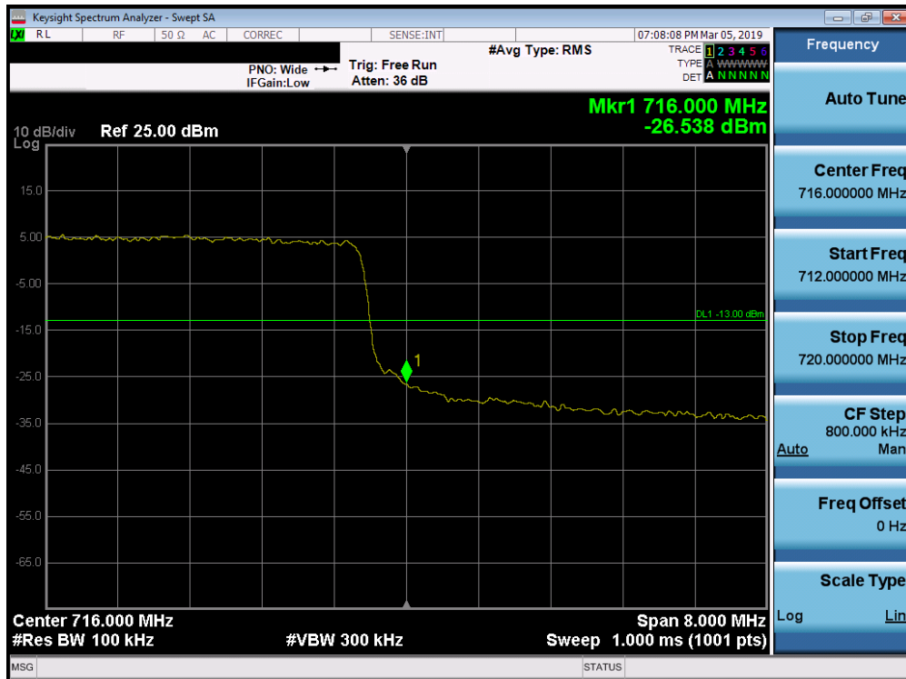
Plot 7-104. Upper Band Edge Plot (Band 12 - 10.0MHz QPSK - Full RB Configuration)
