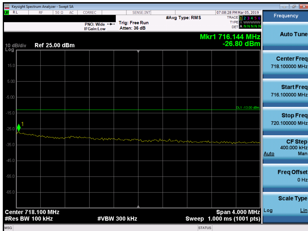
Plot 7-105. Upper Extended Band Edge Plot (Band 12 - 10.0MHz QPSK - Full RB Configuration)
