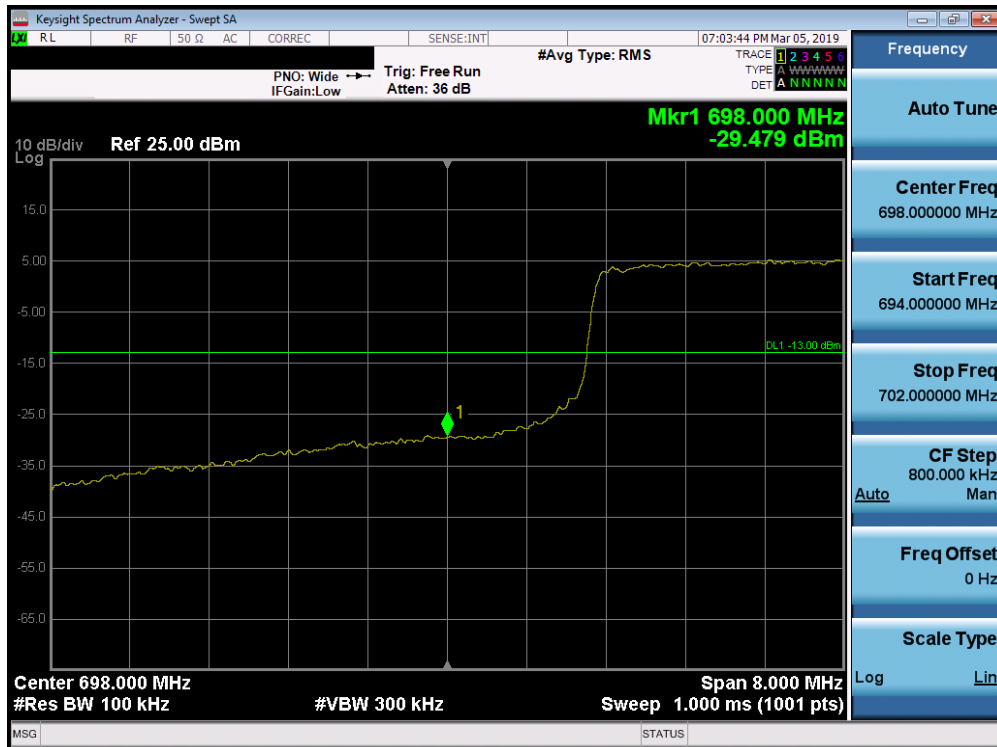
Plot 7-102. Lower Band Edge Plot (Band 12 - 10.0MHz QPSK - Full RB Configuration)
