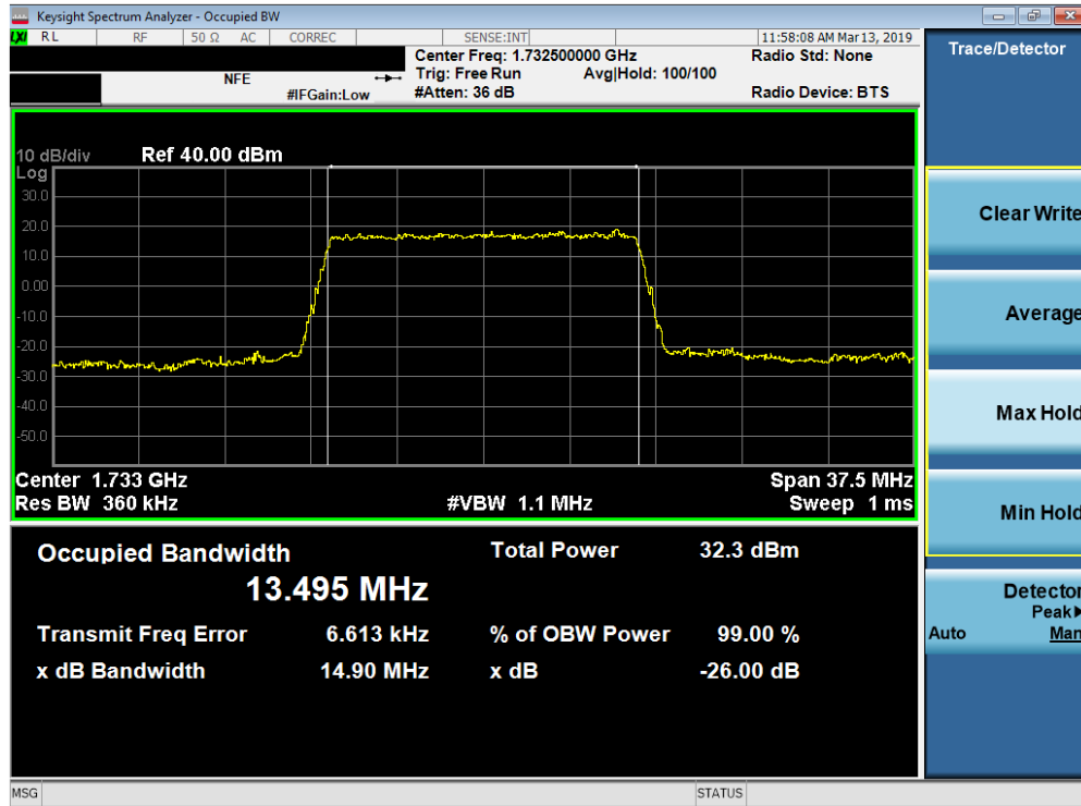
Plot 7-29. Occupied Bandwidth Plot (Band 4 - 15.0MHz QPSK - Full RB Configuration)
