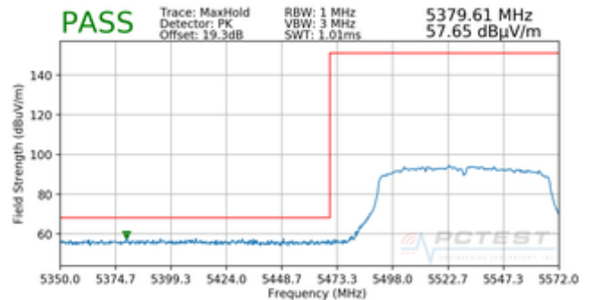
Plot 7-102. Radiated Lower Band Edge Plot (Peak – UNII Band 2C)
