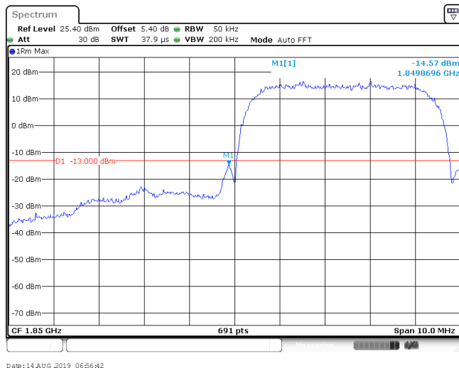
Band II_16QAM_9262
