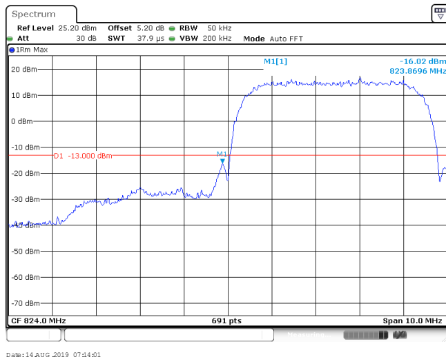
Band V_16QAM_4132
