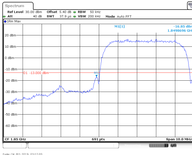
Band II_QPSK_9262
