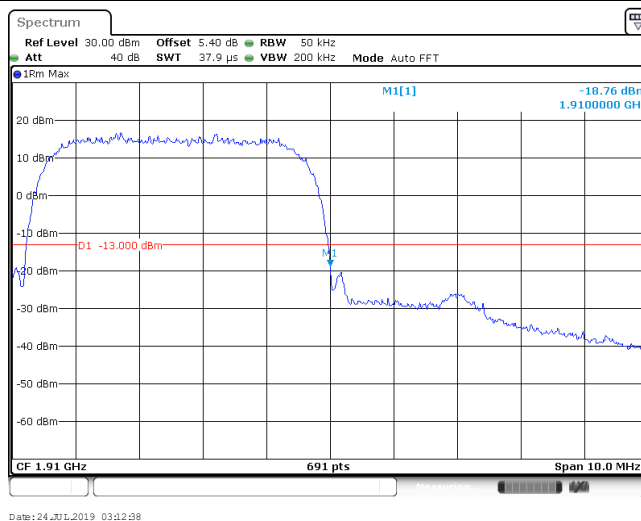
Band II_QPSK_9538
