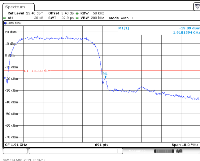
Band II_16QAM_9538
