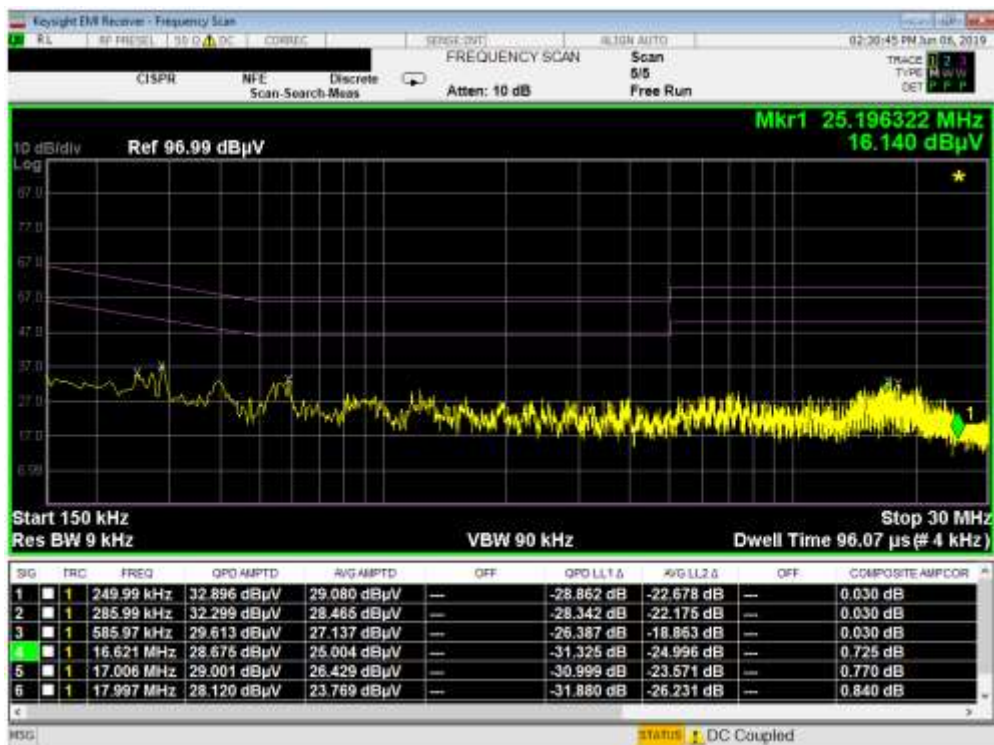
Plot 7-39. Line Conducted Plot with Bluetooth LE (N)
