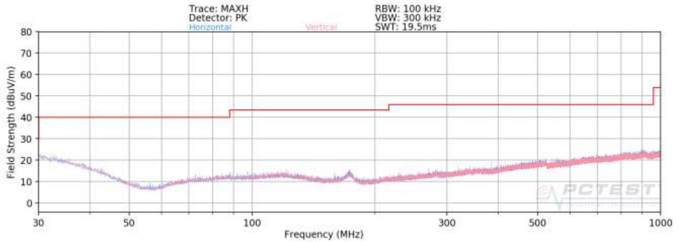
Plot 7-37. Radiated Spurious Plot below 1GHz
