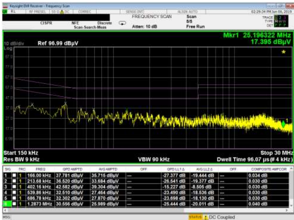
Plot 7-38. Line Conducted Plot with Bluetooth LE (L1)
