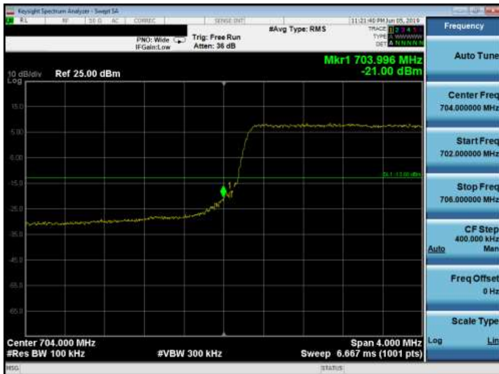
Plot 7-106. Lower Band Edge Plot (Band 17 - 5.0MHz QPSK - Full RB Configuration)
