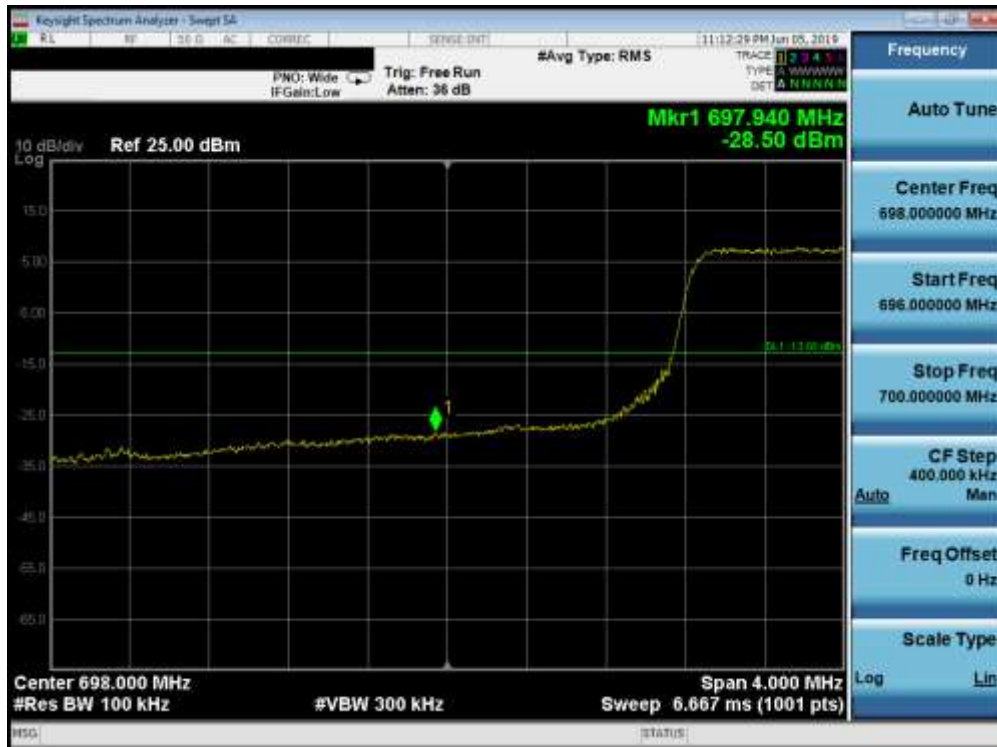
Plot 7-105. Lower Band Edge Plot (Band 12 - 5.0MHz QPSK - Full RB Configuration)
