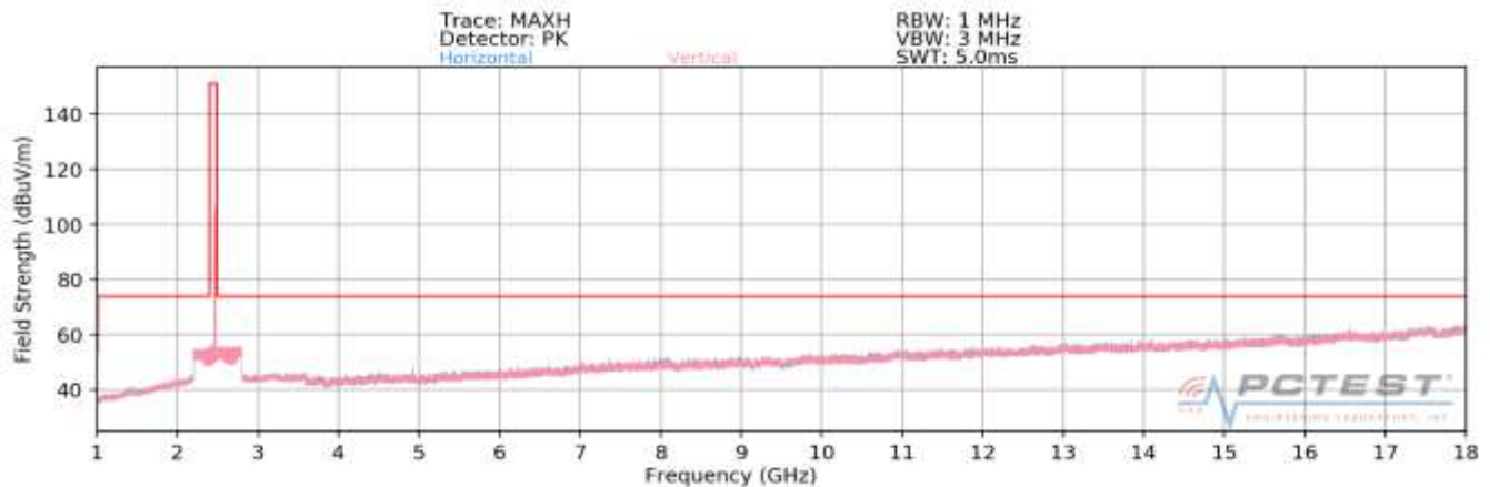
Plot 7-33. Radiated Spurious Plot above 1GHz (802.11b – Ch. 11)
