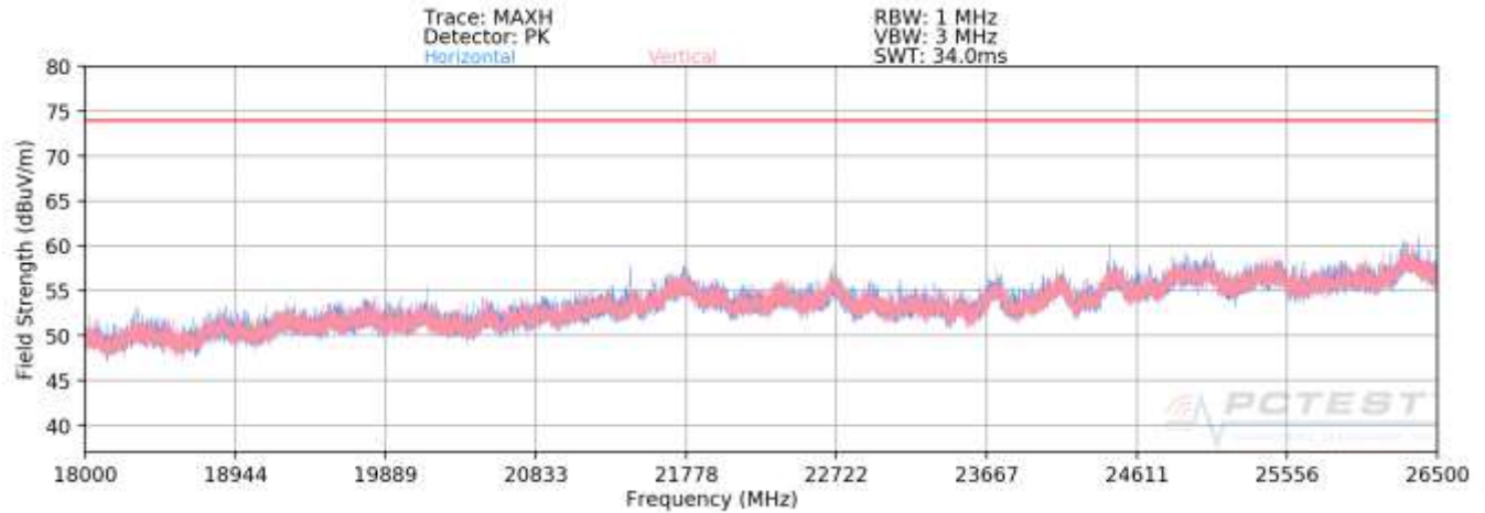
Plot 7-34. Radiated Spurious Plot above 18GHz
