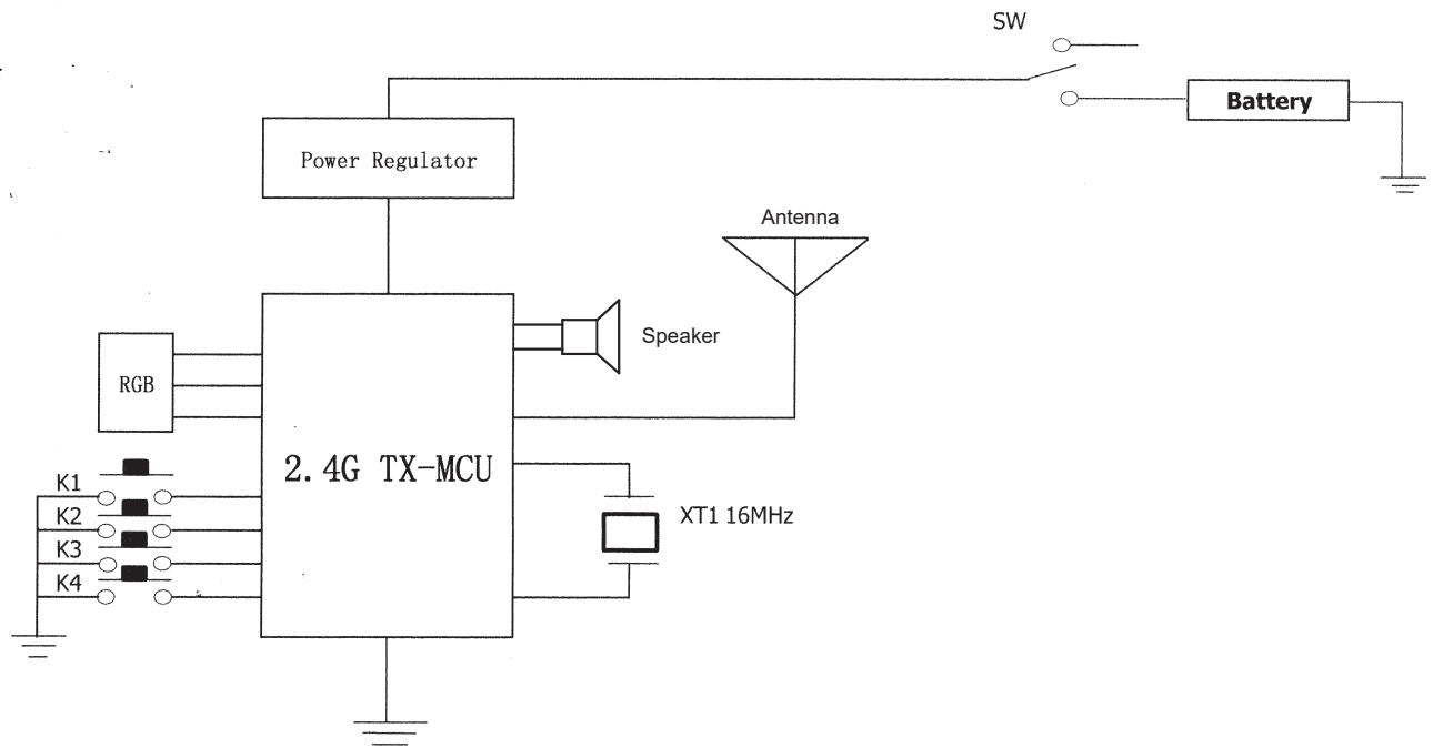
TX Block Diagram
