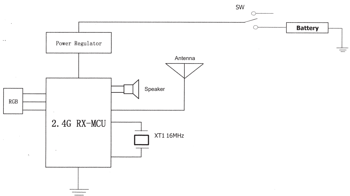
RX Block Diagram
