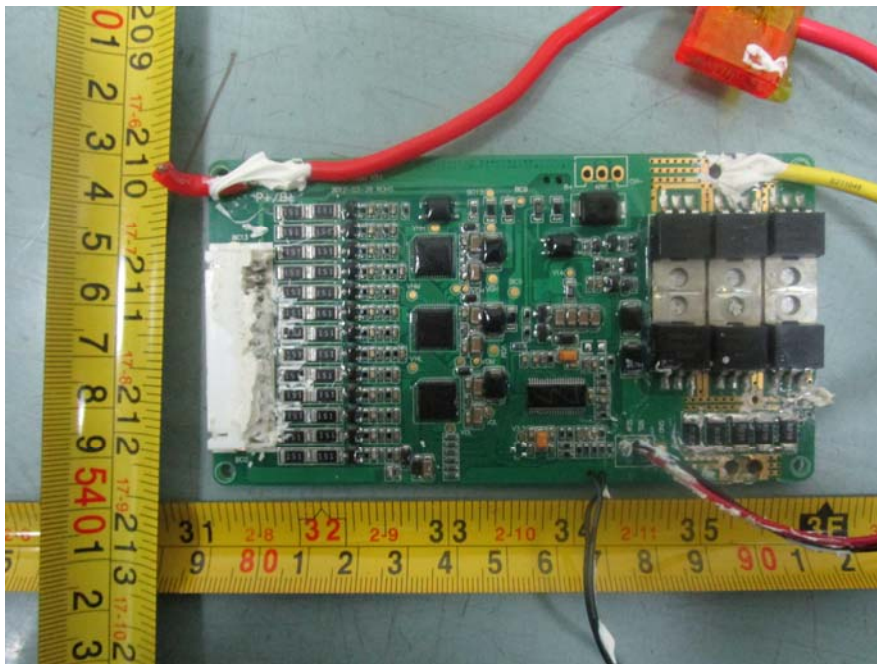
EUT – Charging Board Top View
