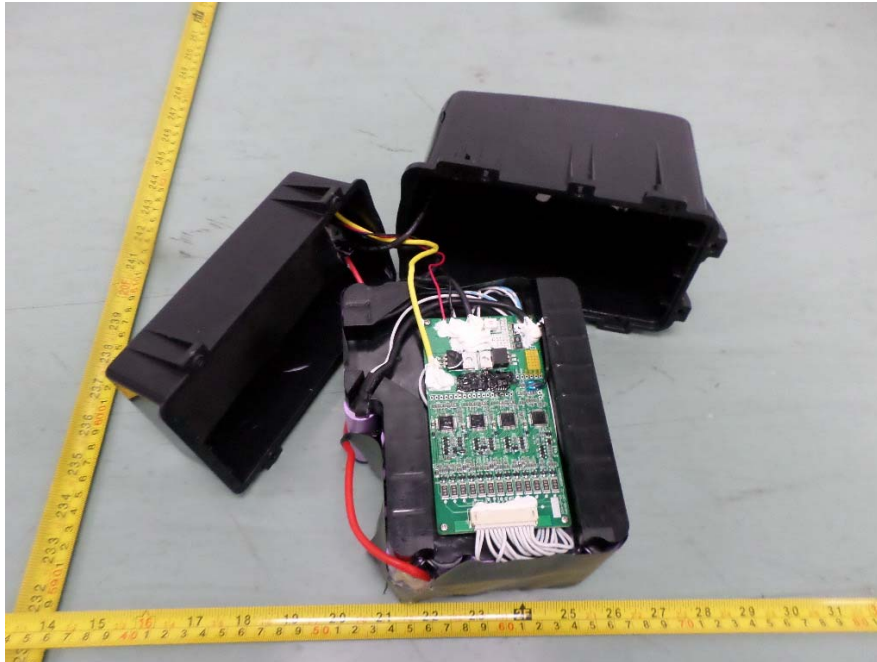
EUT – Battery Box Uncover View
