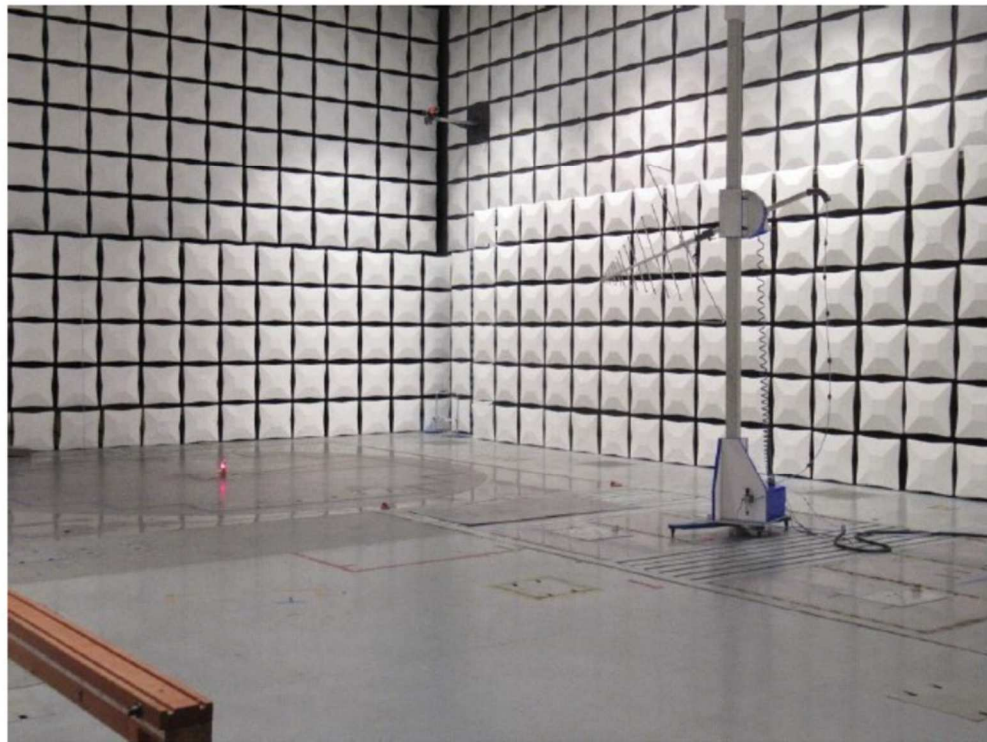
Test setup for radiated emission
