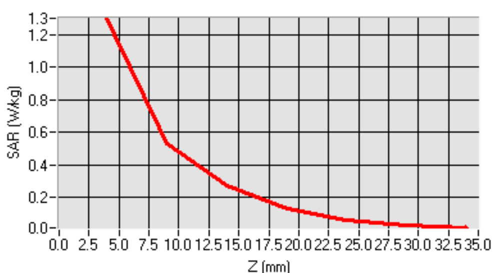
SAR, Z Axis Scan (X = 30, Y = 10)
