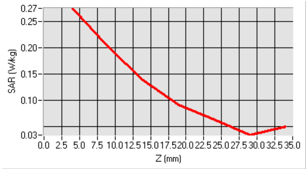
SAR, Z Axis Scan (X = -31, Y = -15)
