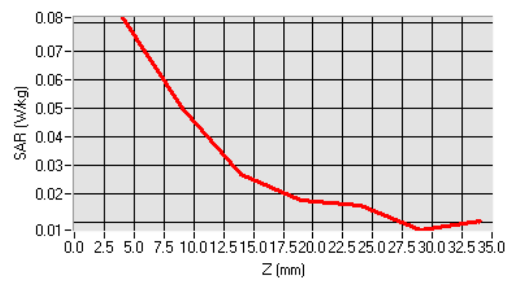
SAR, Z Axis Scan (X = -16, Y = -2)
