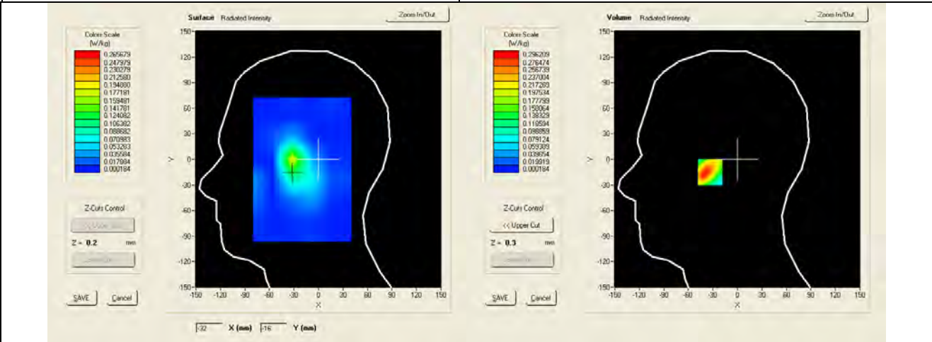
SAR, Z Axis Scan (X = -31, Y = -15)
