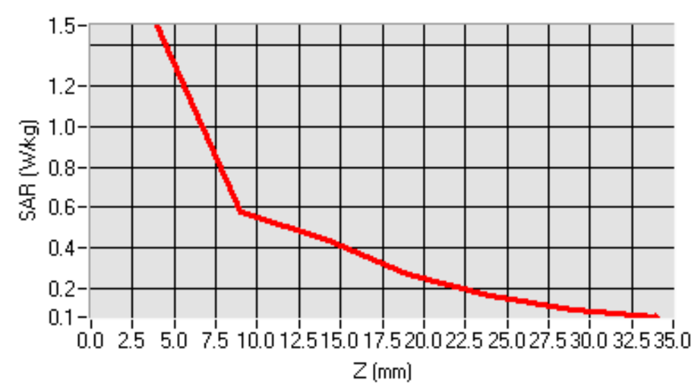
SAR, Z Axis Scan (X = 30, Y = 10)
