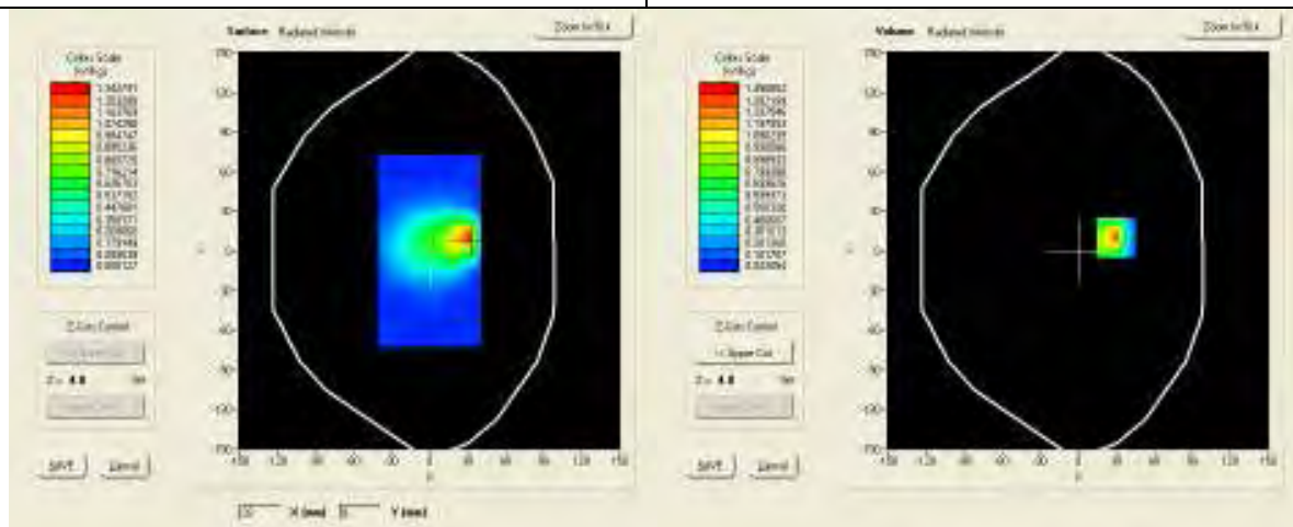
SAR, Z Axis Scan (X = 30, Y = 10)
