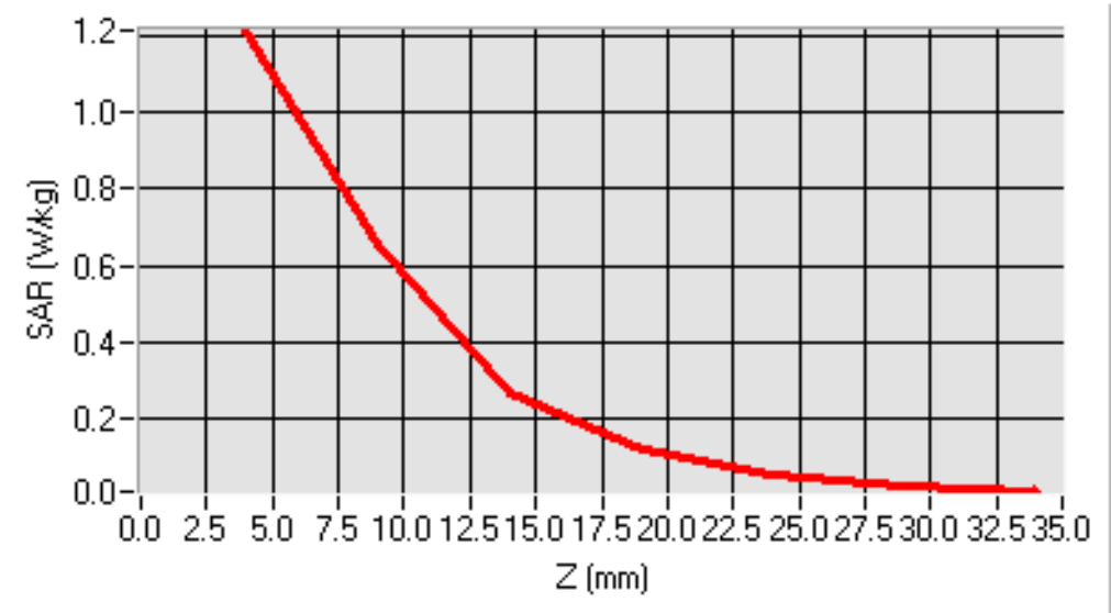
SAR, Z Axis Scan (X = 21, Y = 18)
