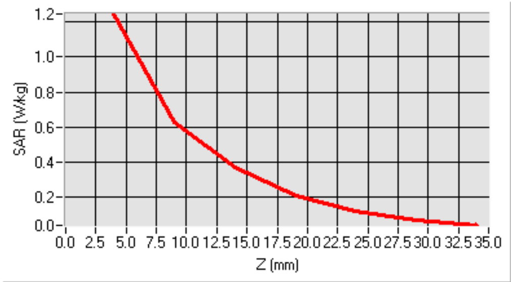
SAR, Z Axis Scan (X = 22, Y = 17)
