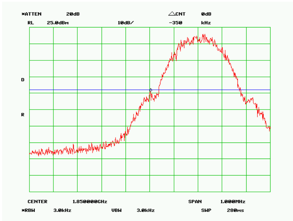
Lower Band Edge Plot – PCS1900, Channel 512, Low Channel
