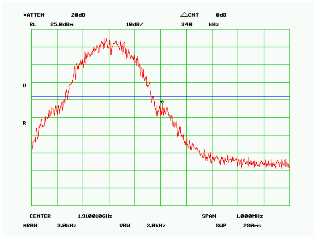
Higher Band Edge Plot – PCS1900, Channel 810, High Channel
