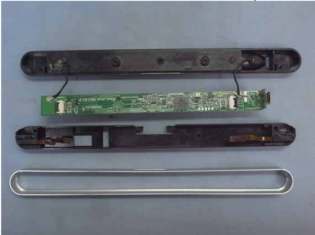
Figure 6 Internal View (Removed Covers)
