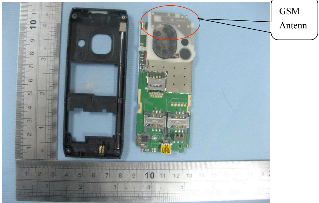
OPEN VIEW OF SAMPLE -3
