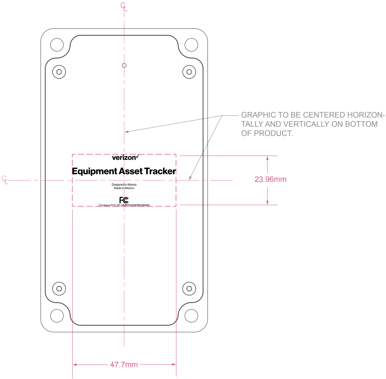
PRIME ARTWORK PLACEMENT SCALE 1:1
