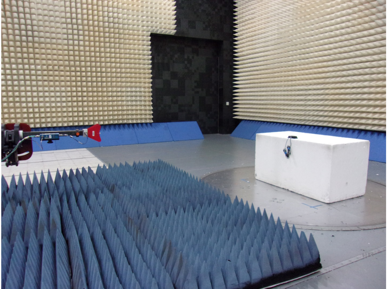
Unintentional emissions – 1-18GHz
