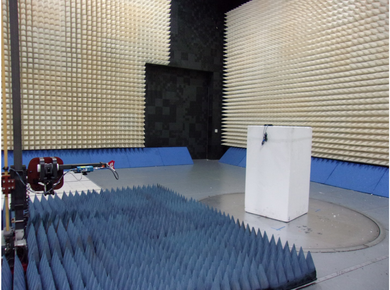
Intentional emissions – 18-40GHz
