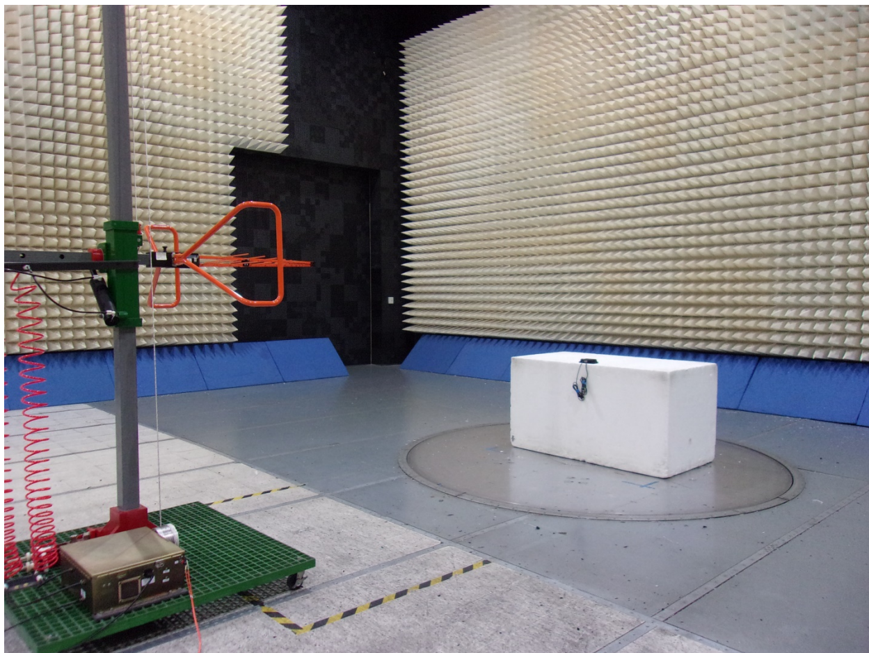
Intentional and unintentional emissions – 30MHz-1GHz
