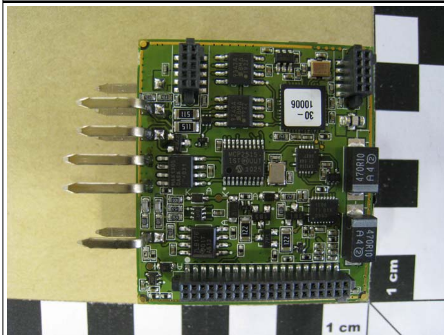
PCB 1 FRONT
