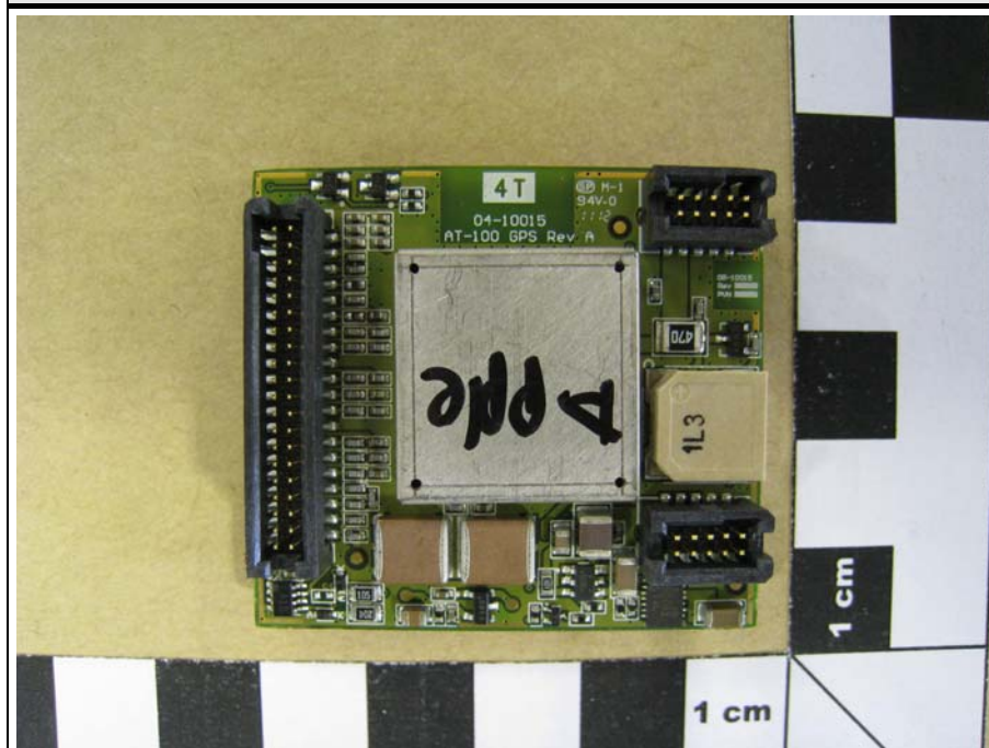
PCB 2 FRONT
