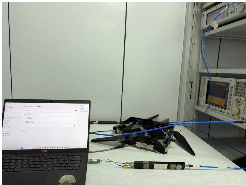
Picture 1 DFS Test Setup
