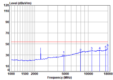
BLE_TX_CH_00_Vertical-Avg
