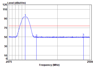
BLE_TX_CH_39_Horizontal-Peak
