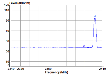
BLE_TX_CH_00_Vertical-AVG
