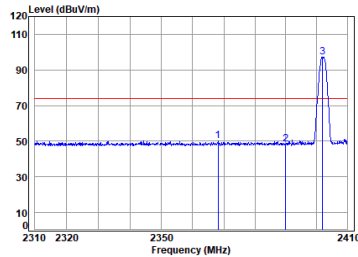
BLE_TX_CH_00_Horizontal-Peak
