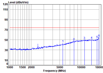
BLE_TX_CH_39_Horizontal-Peak
