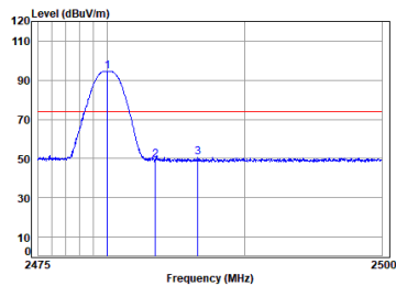
BLE_TX_CH_39_Vertical-Peak
