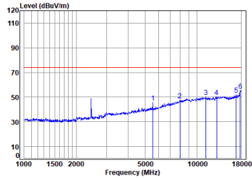
BLE_TX_CH_19_Horizontal-Peak
