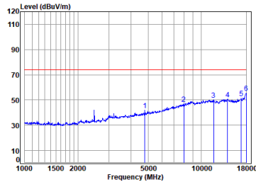
BLE_TX_CH_39_Vertical-Peak
