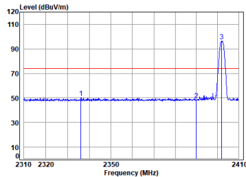
BLE_TX_CH_00_Vertical-Peak
