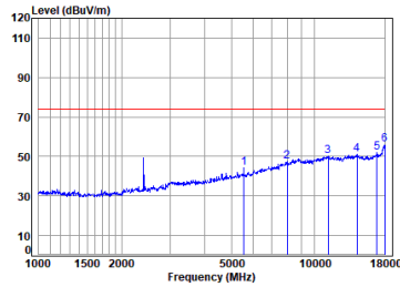
BLE_TX_CH_00_Horizontal-Peak
