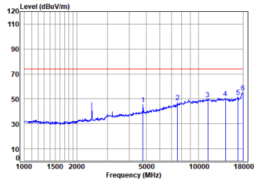
BLE_TX_CH_19_Vertical-Peak
