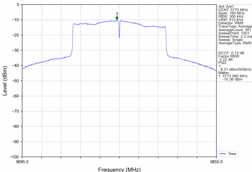
802.11ac(VHT80)_MCH_5775MHz_Ant1_NTNV
