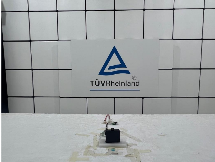
Photograph 3: Test Setup for Spurious Emissions (Front View 3)
