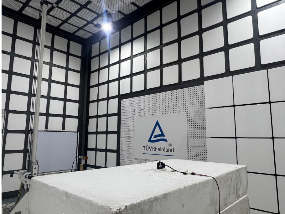
Photograph 7: Test Setup for Spurious Emissions (Back View 4)
