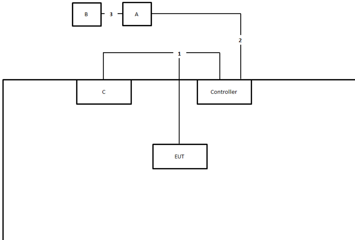
Test Setup Diagram - Radiated Above 1GHz Test
