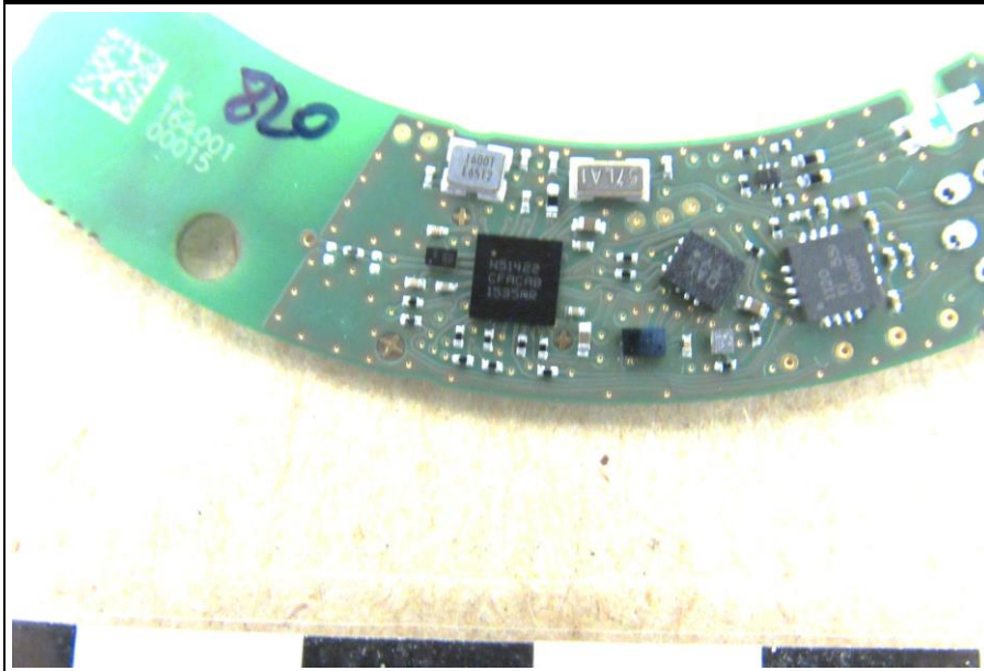
PCB Detail 2
