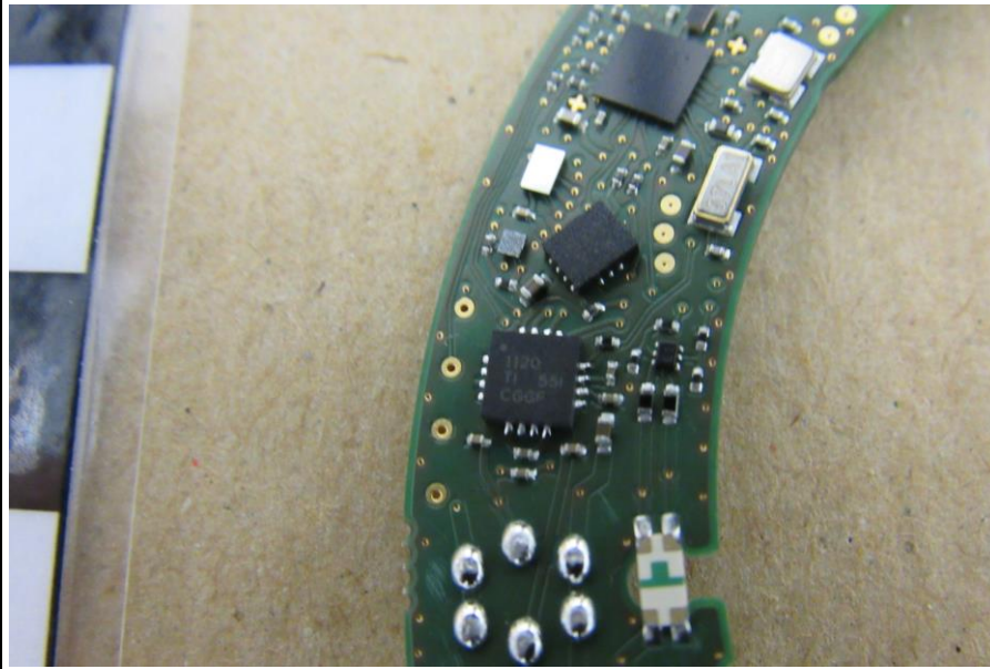
PCB Detail
