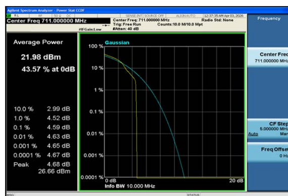
Band12-10MHz-16QAM-23130-1RB#0-PASS
