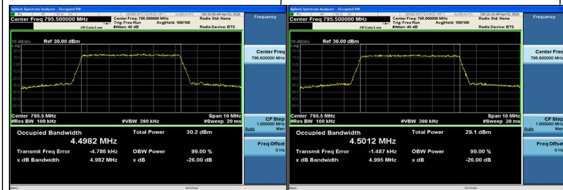
Band14-5MHz-QPSK-23355-25RB#0-PASS
