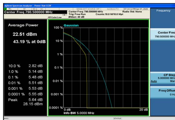
Band14-5MHz-16QAM-23305-1RB#0-PASS
