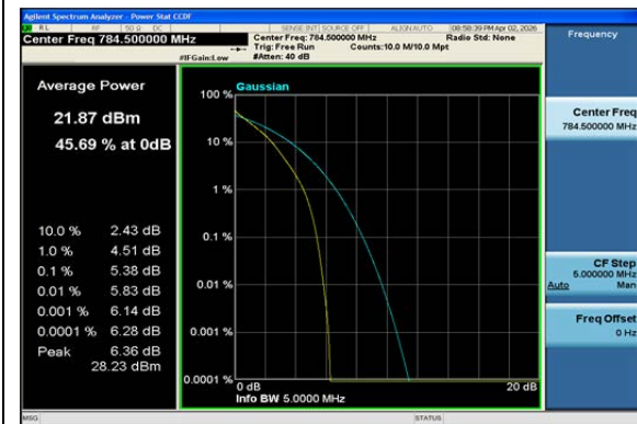
Band13-5MHz-QPSK-23255-25RB#0-PASS
