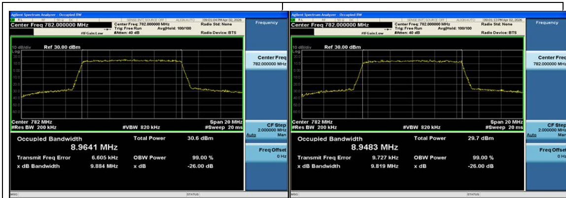
Band13-10MHz-QPSK-23230-50RB#0-PASS
