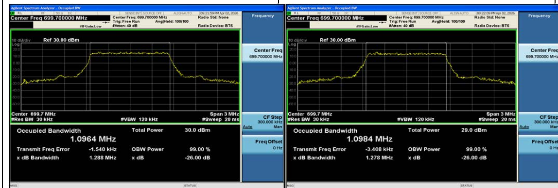
Band12-1.4MHz-QPSK-23017-6RB#0-PASS
