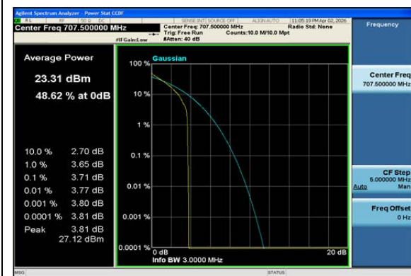
Band12-3MHz-QPSK-23095-1RB#0-PASS
