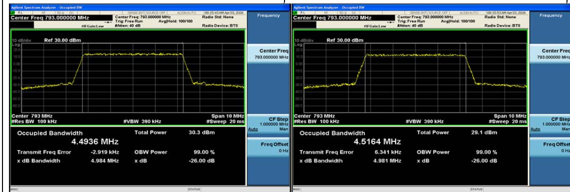
Band14-5MHz-QPSK-23330-25RB#0-PASS
