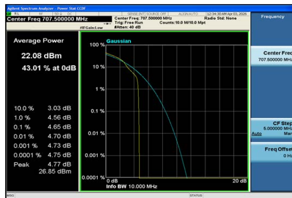
Band12-10MHz-16QAM-23095-1RB#0-PASS
