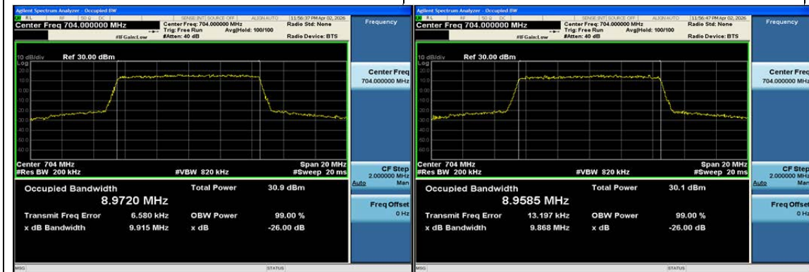
Band12-10MHz-QPSK-23060-50RB#0-PASS
