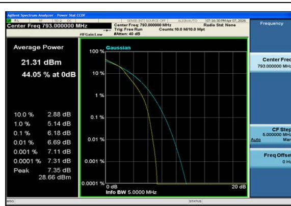
Band14-5MHz-16QAM-23330-25RB#0-PASS
