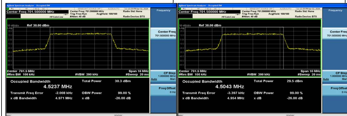
Band12-5MHz-QPSK-23035-25RB#0-PASS
