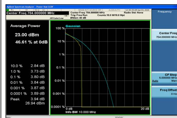
Band12-10MHz-QPSK-23060-1RB#0-PASS
