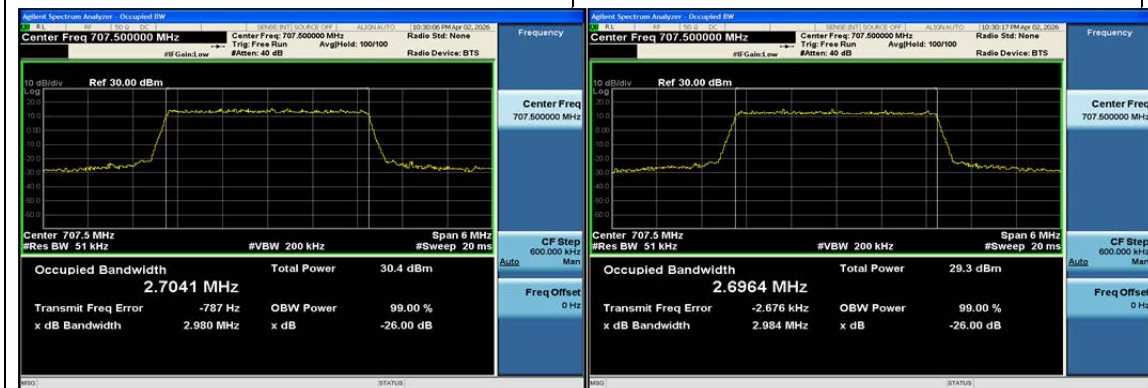
Band12-3MHz-QPSK-23095-15RB#0-PASS
