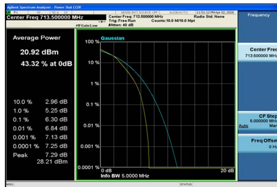
Band12-5MHz-16QAM-23155-25RB#0-PASS
