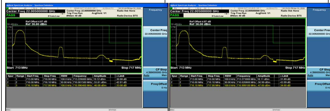
Band12-3MHz-QPSK-23165-1RB#0-PASS
