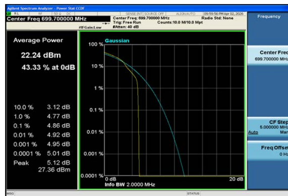
Band12-1.4MHz-16QAM-23017-1RB#0-PASS
