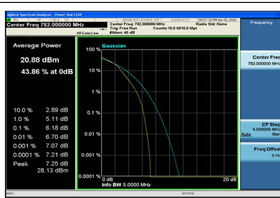
Band13-5MHz-16QAM-23230-25RB#0-PASS
