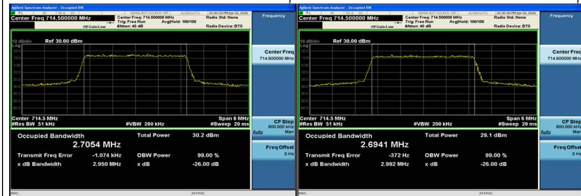
Band12-3MHz-QPSK-23165-15RB#0-PASS
