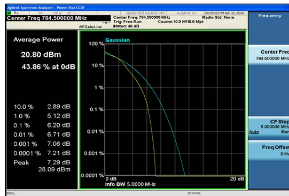
Band13-5MHz-16QAM-23255-25RB#0-PASS
