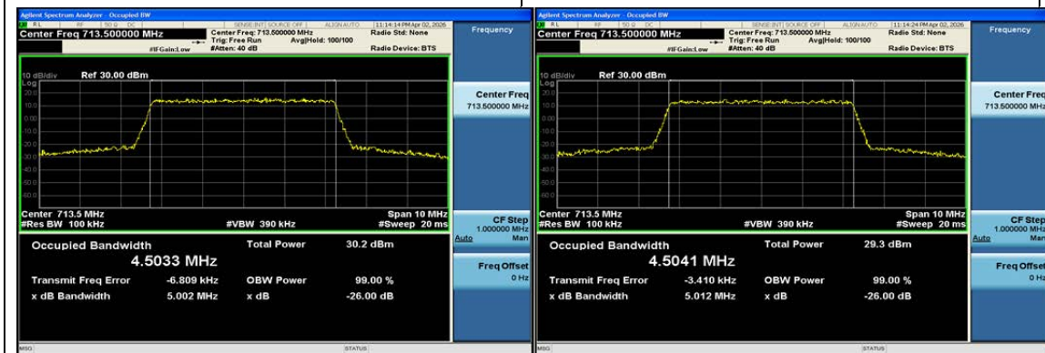
Band12-5MHz-QPSK-23155-25RB#0-PASS
