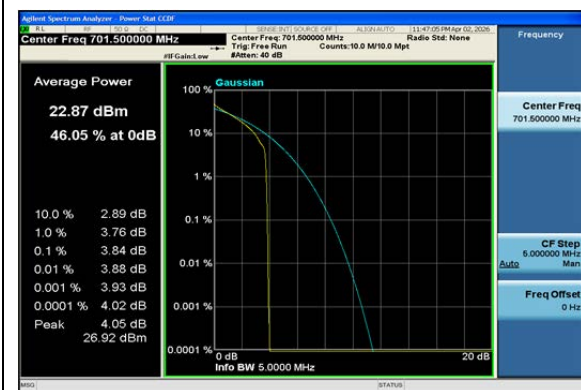
Band12-5MHz-QPSK-23035-1RB#0-PASS
