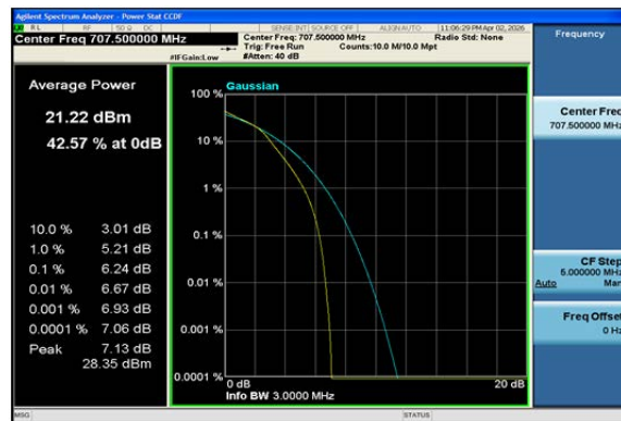
Band12-3MHz-16QAM-23095-15RB#0-PASS
