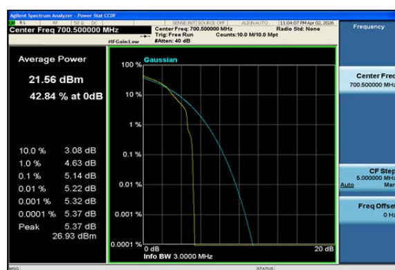
Band12-3MHz-16QAM-23025-1RB#0-PASS
