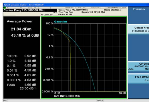
Band12-5MHz-16QAM-23155-1RB#0-PASS
