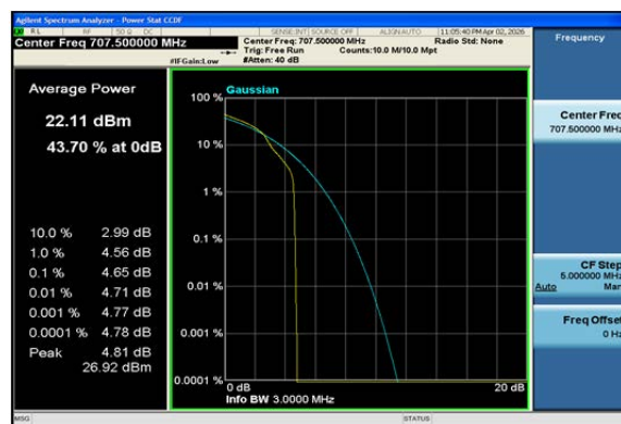
Band12-3MHz-16QAM-23095-1RB#0-PASS
