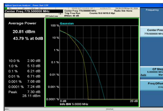
Band13-5MHz-16QAM-23205-25RB#0-PASS
