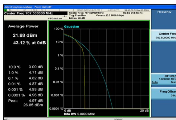
Band12-5MHz-16QAM-23095-1RB#0-PASS
