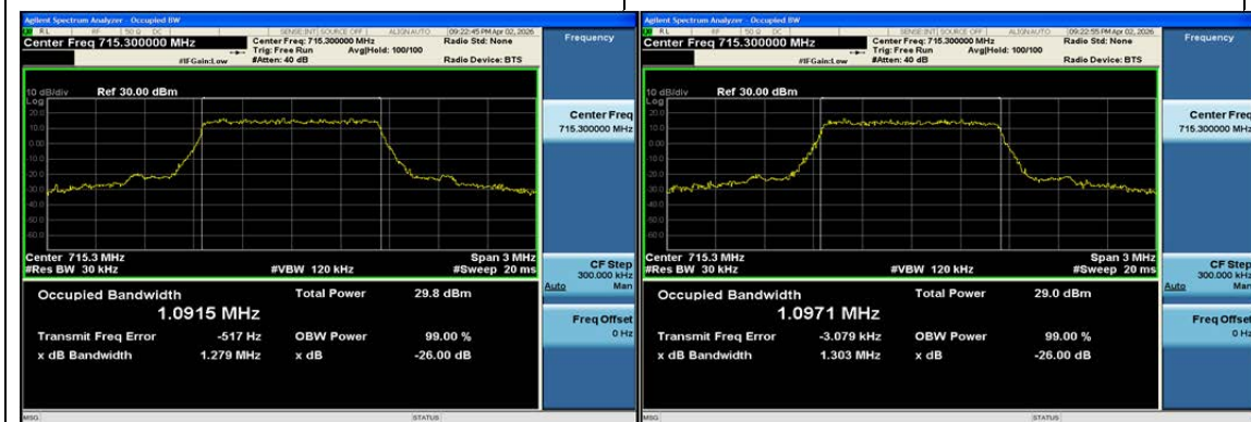
Band12-1.4MHz-QPSK-23173-6RB#0-PASS
