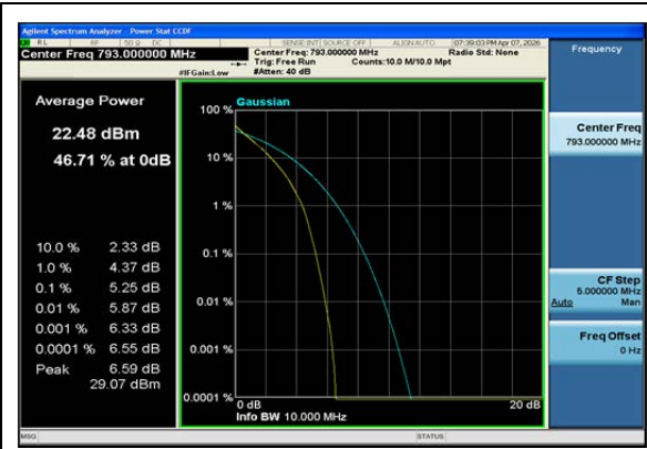
Band14-10MHz-QPSK-23330-50RB#0-PASS
