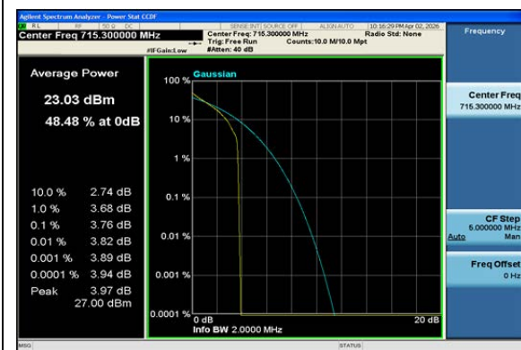
Band12-1.4MHz-QPSK-23173-1RB#0-PASS
