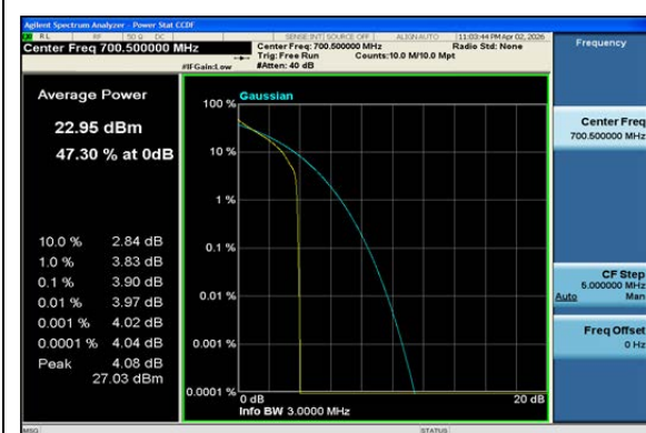
Band12-3MHz-QPSK-23025-1RB#0-PASS
