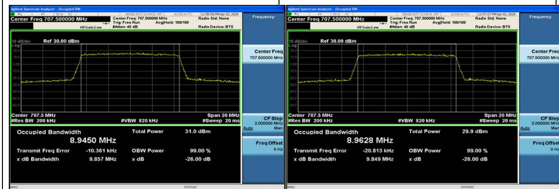
Band12-10MHz-QPSK-23095-50RB#0-PASS
