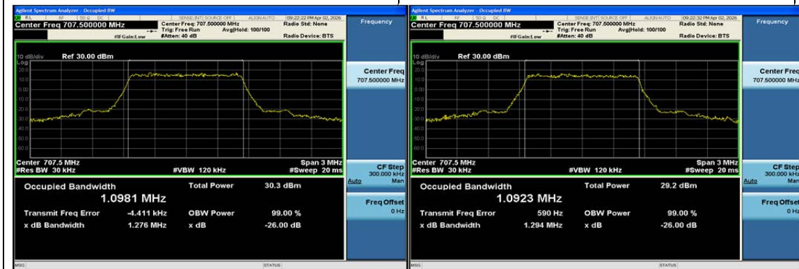
Band12-1.4MHz-QPSK-23095-6RB#0-PASS
