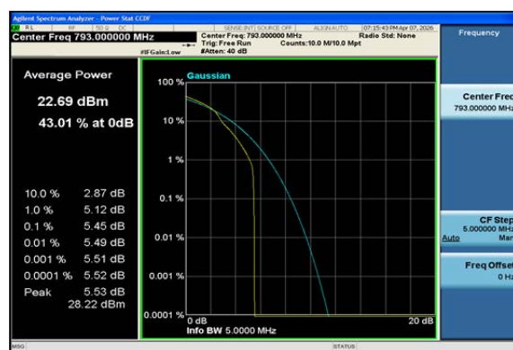
Band14-5MHz-16QAM-23330-1RB#0-PASS
