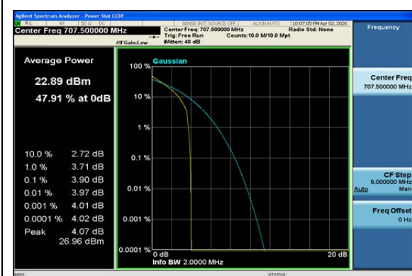
Band12-1.4MHz-QPSK-23095-1RB#0-PASS
