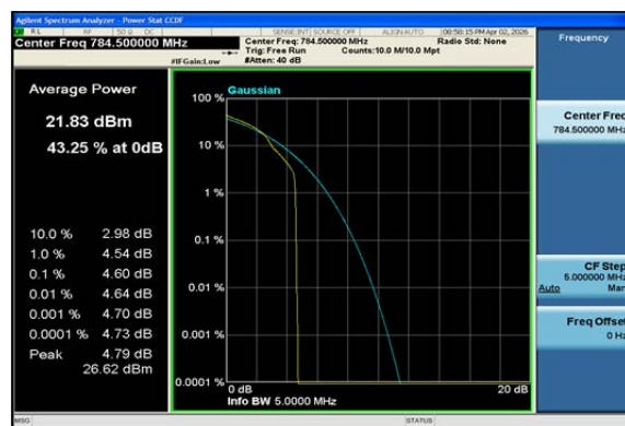
Band13-5MHz-16QAM-23255-1RB#0-PASS
