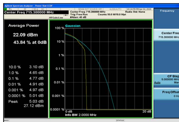
Band12-1.4MHz-16QAM-23173-1RB#0-PASS
