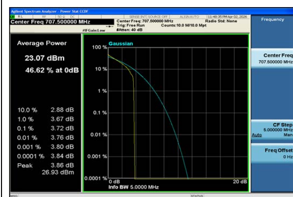
Band12-5MHz-QPSK-23095-1RB#0-PASS
