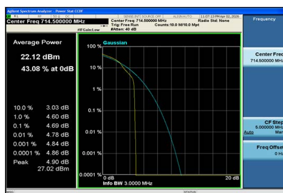
Band12-3MHz-16QAM-23165-1RB#0-PASS
