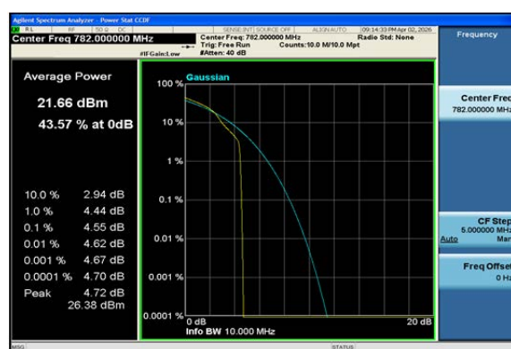
Band13-10MHz-16QAM-23230-1RB#0-PASS
