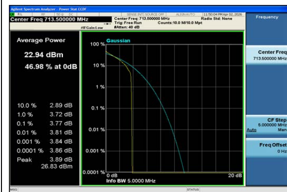
Band12-5MHz-QPSK-23155-1RB#0-PASS
