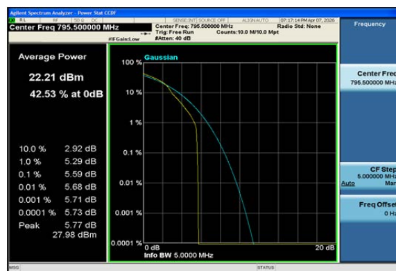
Band14-5MHz-16QAM-23355-1RB#0-PASS
