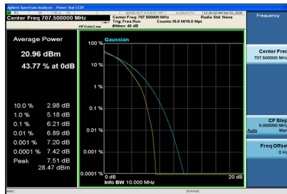
Band12-10MHz-16QAM-23095-50RB#0-PASS
