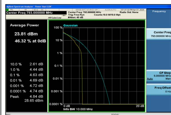
Band14-10MHz-QPSK-23330-1RB#0-PASS
