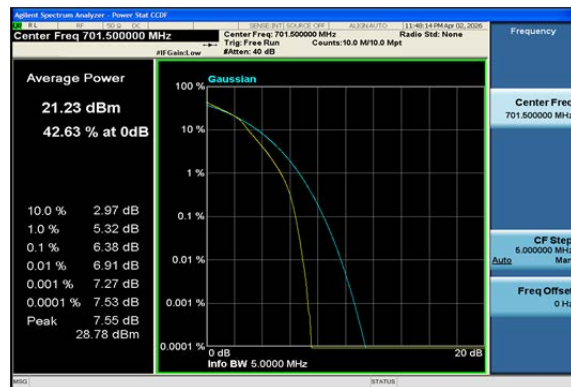
Band12-5MHz-16QAM-23035-25RB#0-PASS
