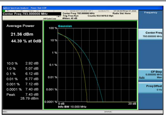
Band14-10MHz-16QAM-23330-50RB#0-PASS
