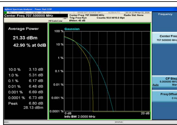
Band12-1.4MHz-16QAM-23095-6RB#0-PASS
