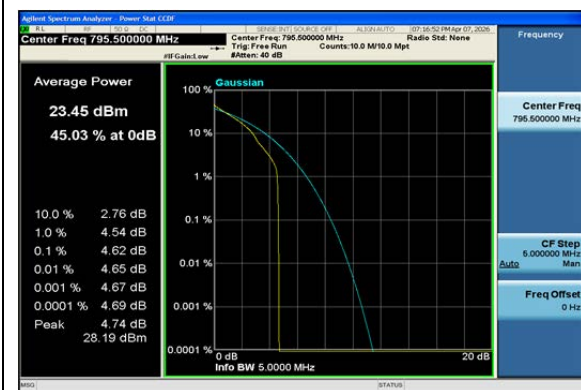
Band14-5MHz-QPSK-23355-1RB#0-PASS
