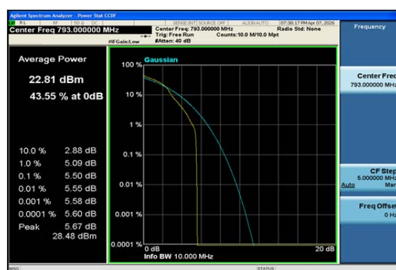
Band14-10MHz-16QAM-23330-1RB#0-PASS
