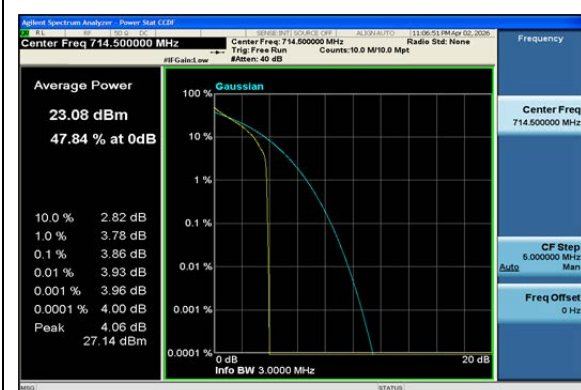
Band12-3MHz-QPSK-23165-1RB#0-PASS
