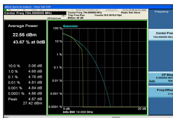
Band12-10MHz-16QAM-23060-1RB#0-PASS
