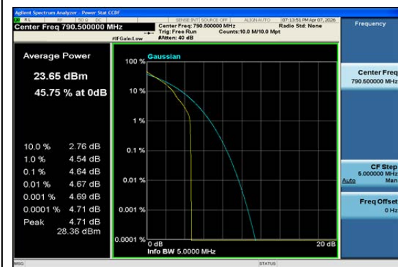
Band14-5MHz-QPSK-23305-1RB#0-PASS
