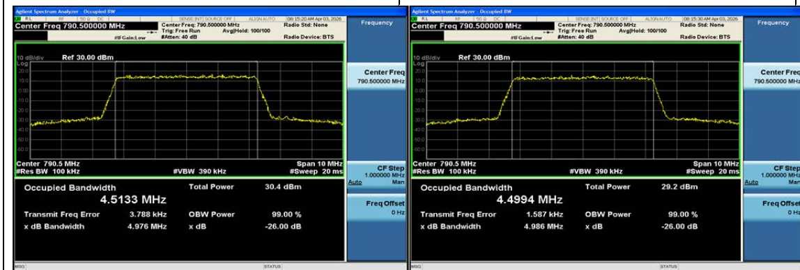
Band14-5MHz-QPSK-23305-25RB#0-PASS
