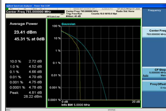
Band14-5MHz-QPSK-23330-1RB#0-PASS
