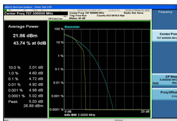
Band12-1.4MHz-16QAM-23095-1RB#0-PASS
