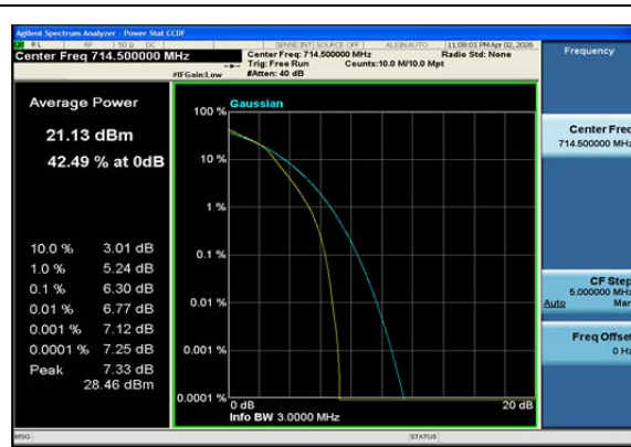
Band12-3MHz-16QAM-23165-15RB#0-PASS
