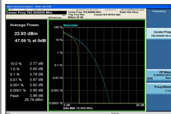
Band13-10MHz-QPSK-23230-1RB#0-PASS
