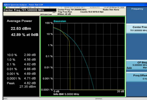
Band12-5MHz-16QAM-23035-1RB#0-PASS
