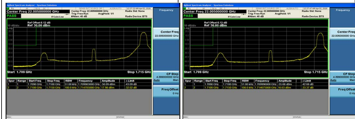
Band4-5MHz-QPSK-19975-1RB#24-PASS
