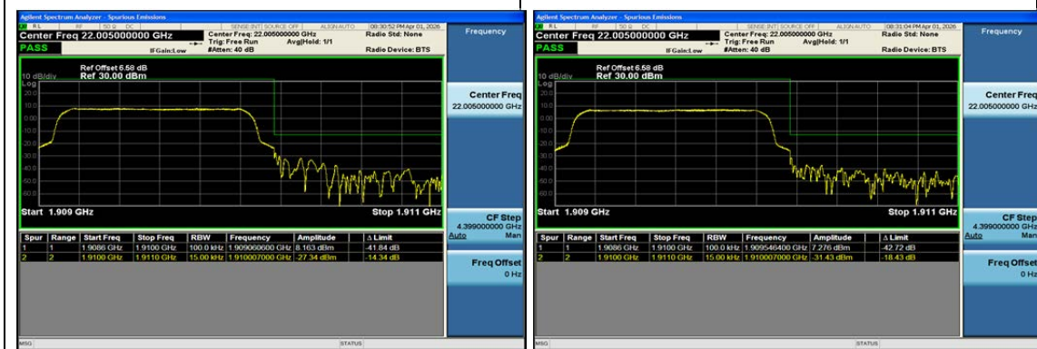
Band2-1.4MHz-QPSK-19193-6RB#0-PASS
