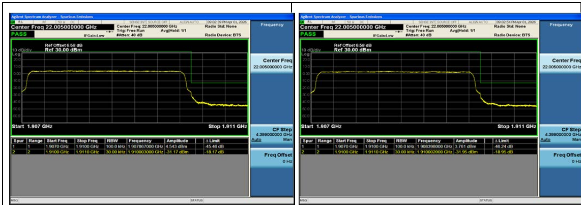
Band2-3MHz-QPSK-19185-15RB#0-PASS
