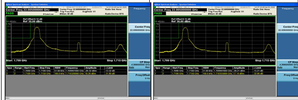
Band4-5MHz-QPSK-19975-1RB#0-PASS
