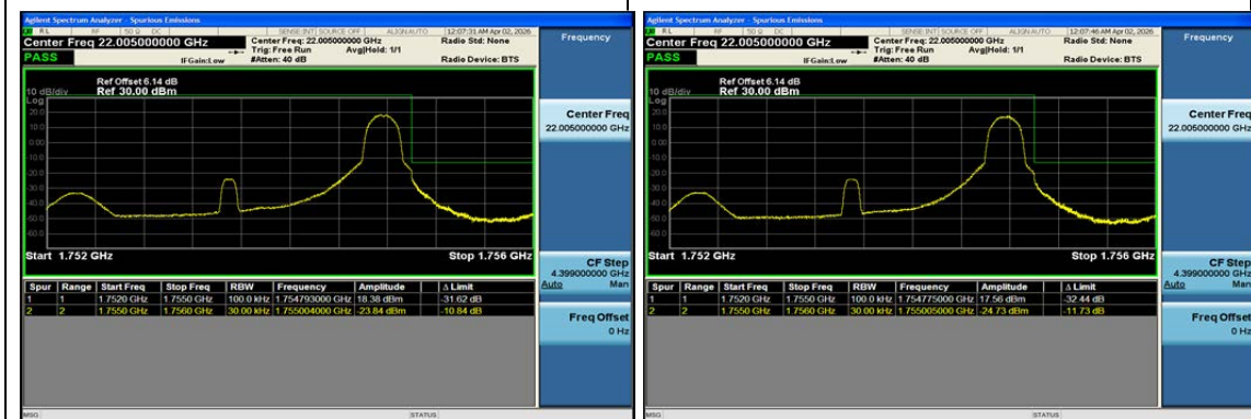
Band4-3MHz-QPSK-20385-1RB#14-PASS
