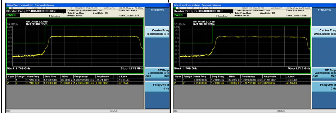
Band4-3MHz-QPSK-19965-15RB#0-PASS
