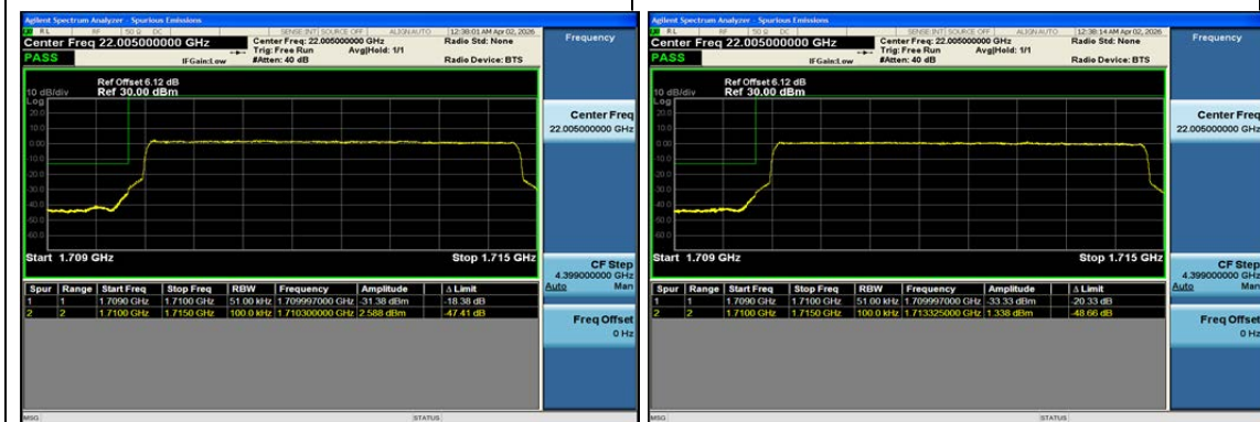
Band4-5MHz-QPSK-19975-25RB#0-PASS
