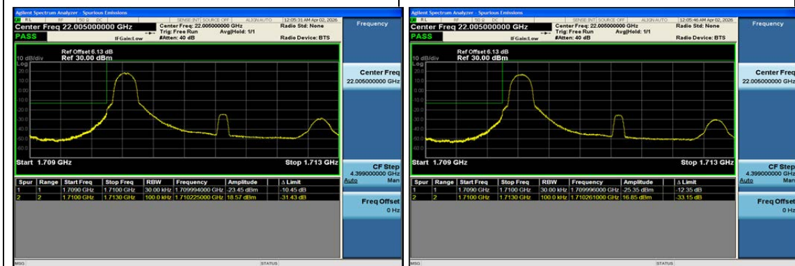
Band4-3MHz-QPSK-19965-1RB#0-PASS
