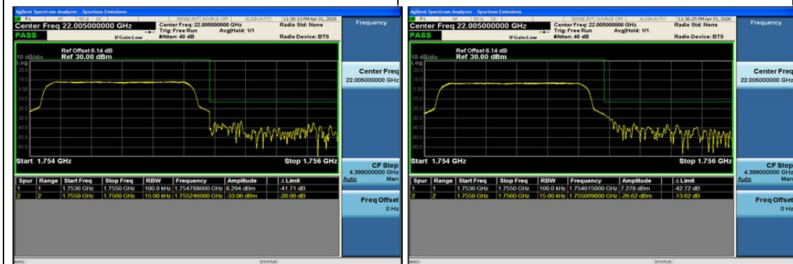
Band4-1.4MHz-QPSK-20393-6RB#0-PASS
