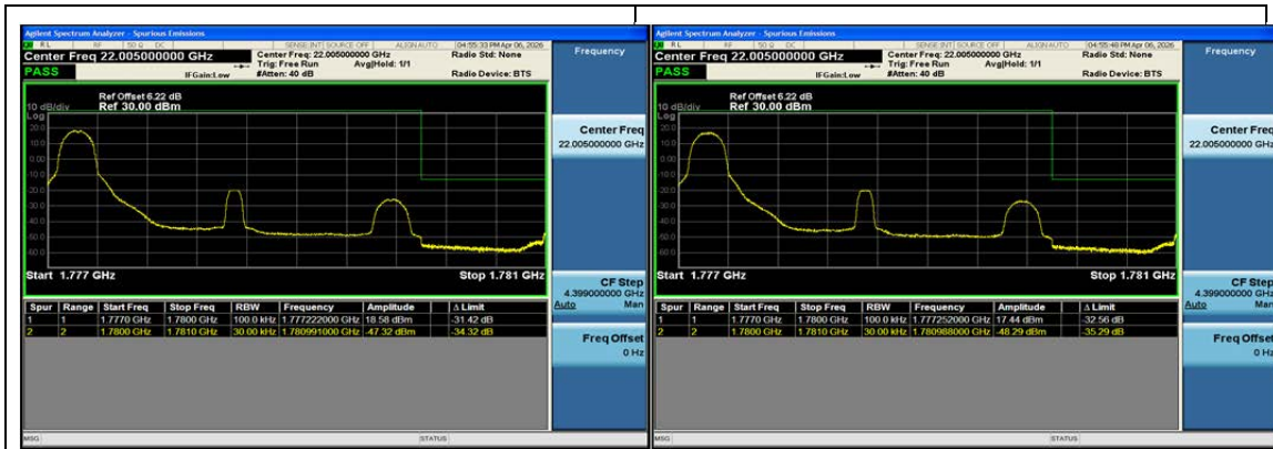
Band66-3MHz-QPSK-132657-1RB#0-PASS
