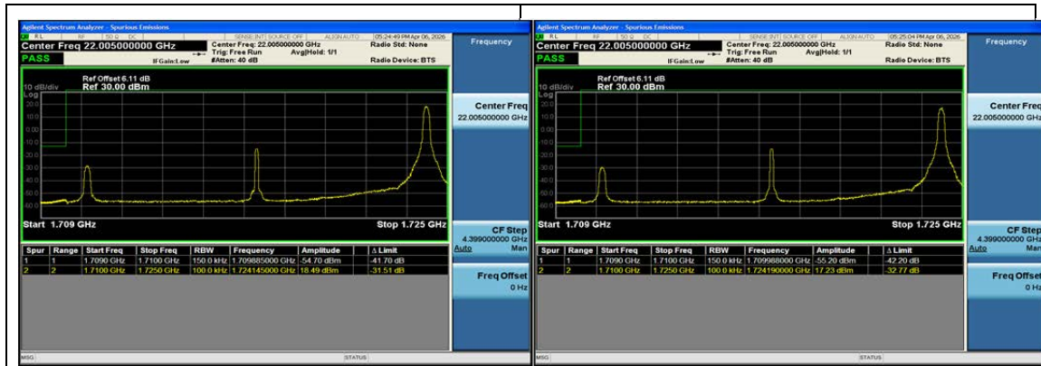
Band66-15MHz-QPSK-132047-1RB#74-PASS
