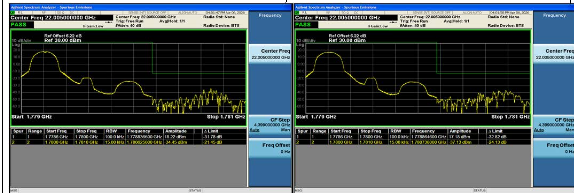
Band66-1.4MHz-QPSK-132665-1RB#0-PASS
