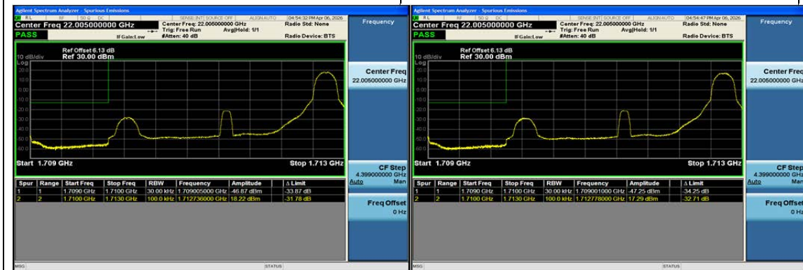
Band66-3MHz-QPSK-131987-1RB#14-PASS
