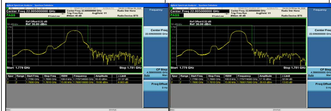
Band66-1.4MHz-QPSK-132665-1RB#5-PASS
