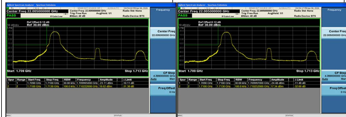
Band66-3MHz-QPSK-131987-1RB#0-PASS
