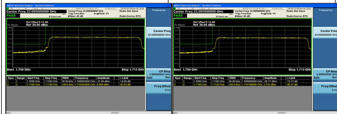
Band66-3MHz-QPSK-131987-15RB#0-PASS
