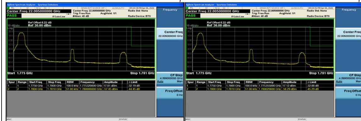
Band66-5MHz-QPSK-132647-1RB#0-PASS
