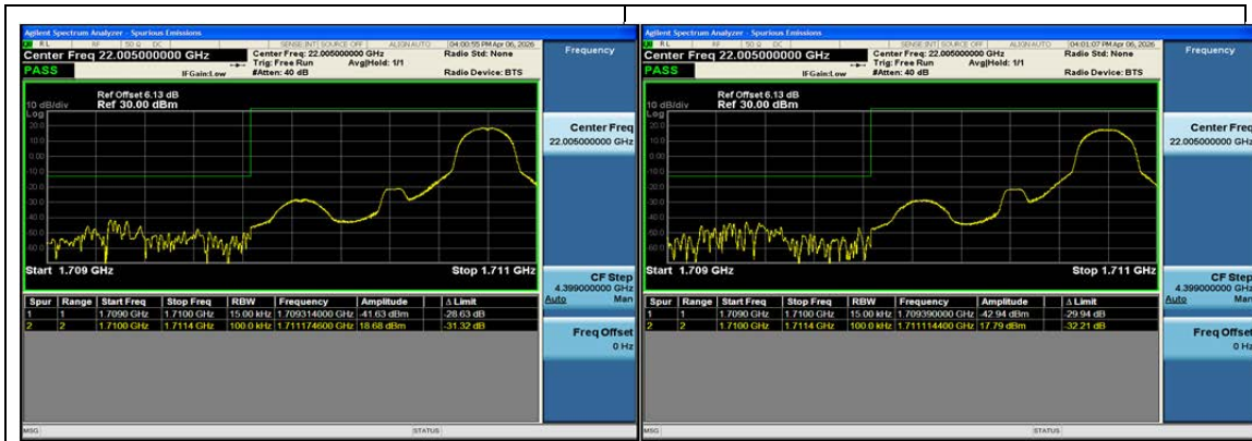
Band66-1.4MHz-QPSK-131979-1RB#5-PASS
