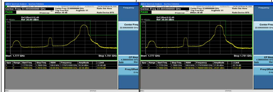
Band66-3MHz-QPSK-132657-1RB#14-PASS
