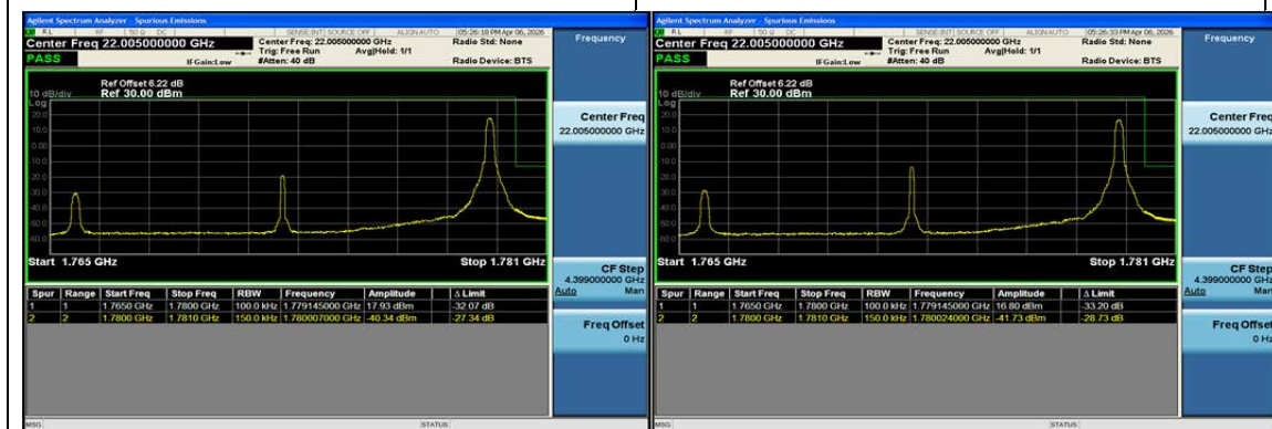
Band66-15MHz-QPSK-132597-1RB#74-PASS
