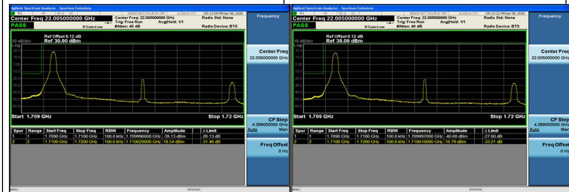
Band66-10MHz-QPSK-132022-1RB#0-PASS
