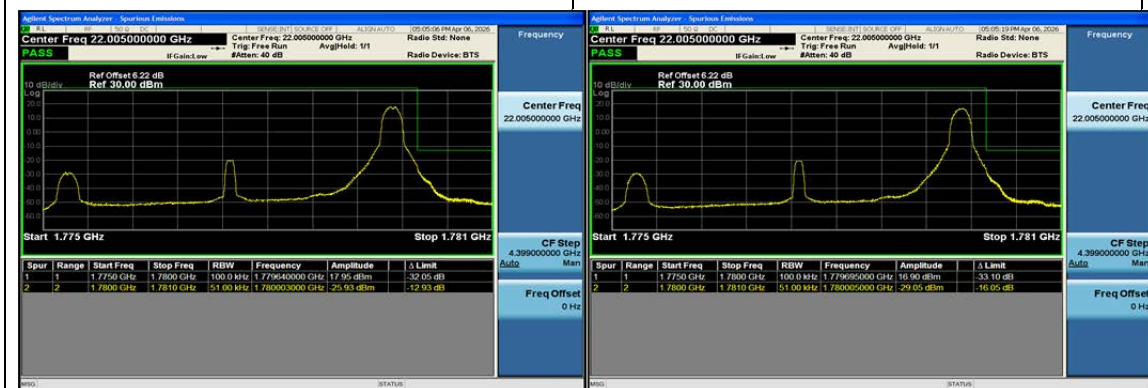
Band66-5MHz-QPSK-132647-1RB#24-PASS
