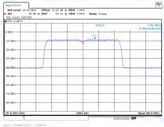
11AX40SISO-Ant1-6925-PASS
