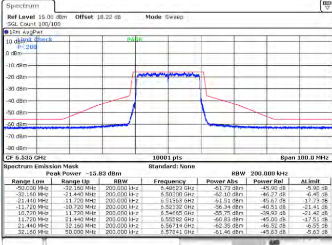
NTNV-11AX20SISO-Ant1-6535-PASS
