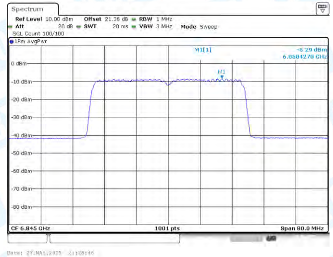
11AX40SISO-Ant1-6845-PASS
