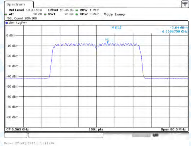
11AX40SISO-Ant1-6565-PASS
