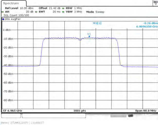
11AX40SISO-Ant1-6965-PASS
