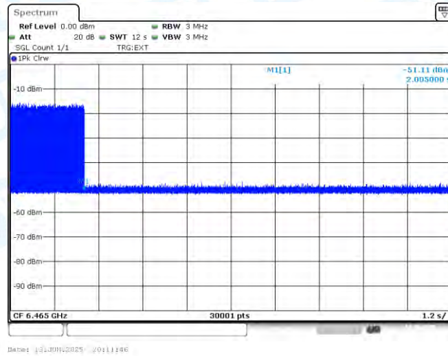
11AX80SISO-Ant1-6465-High-6498.5215-OFF-PASS
