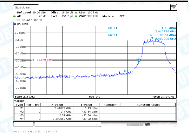
11N20MIMO-Ant2-2412-PASS
