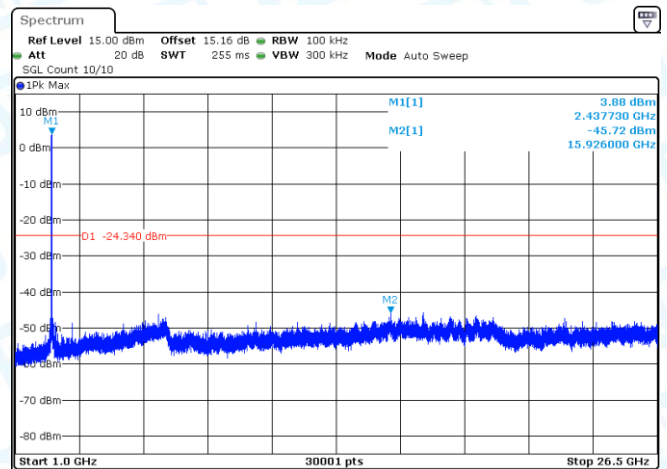
11B-Ant1-2437-0~Reference-PASS
